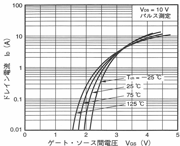
TRANSFER CHARACTERISTIC
