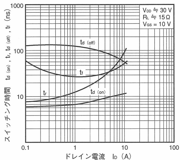
SWITCHING TIME vs. DRAIN CURRENT
