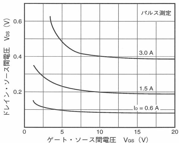
DRAIN TO SOURCE ON-STATE VOLTAGE vs. GATE TO SOURCE VOLTAGE
