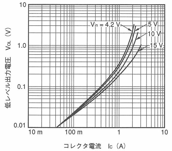
LOW LEVEL OUTPUT VOLTAGE vs. COLLECTOR CURRENT
