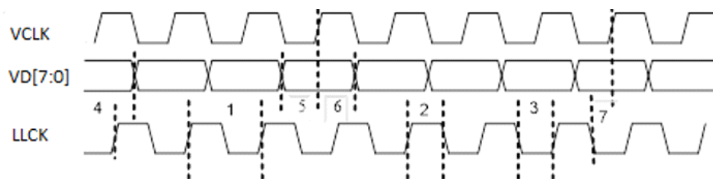
FIGURE 3. CLOCK TIMING DIAGRAM
