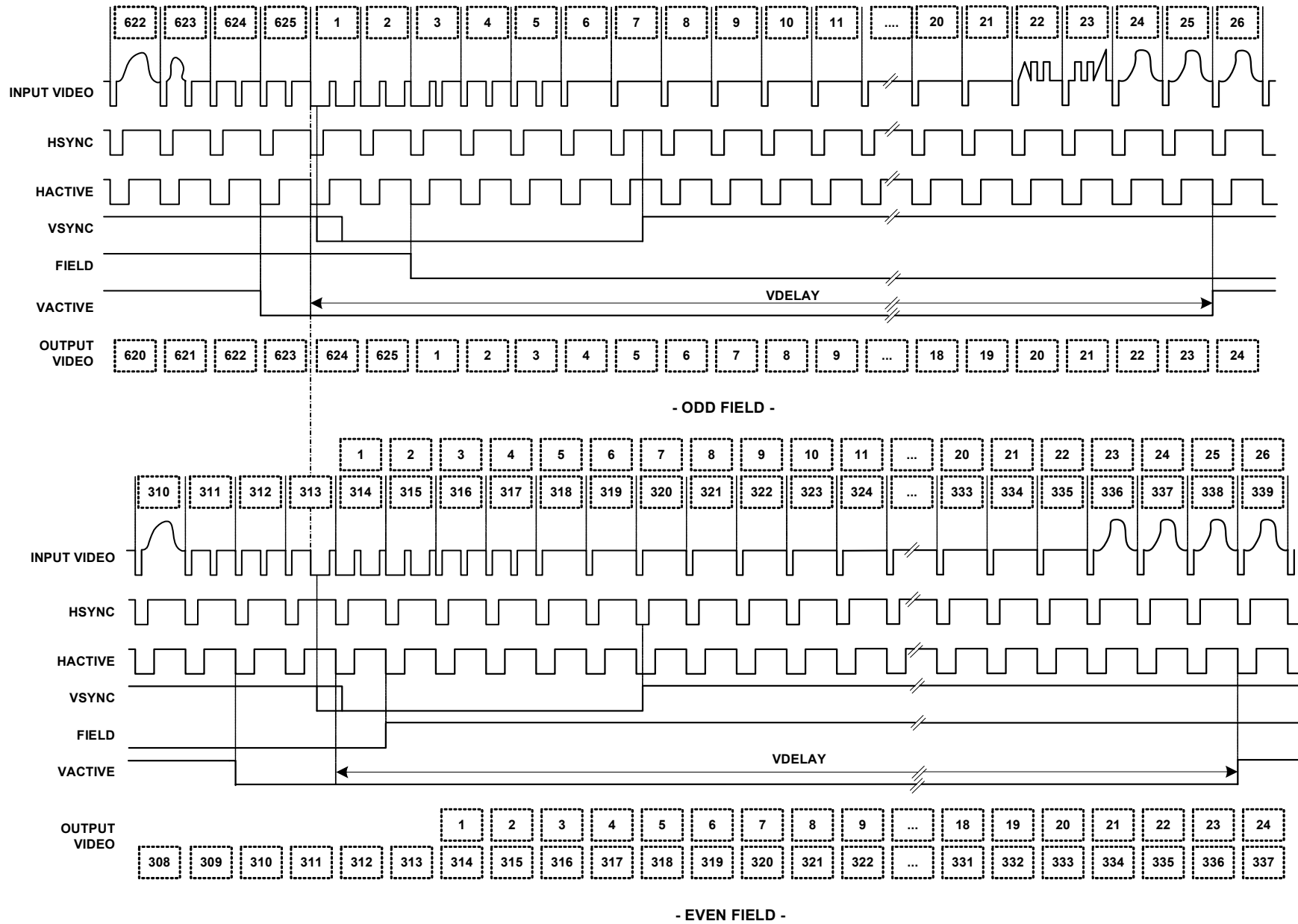
FIGURE 5. VERTICAL TIMING DIAGRAM FOR 50Hz/625 LINE SYSTEM
