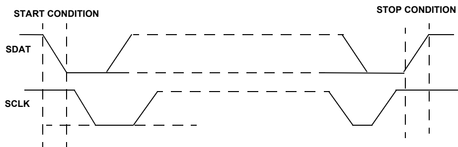
FIGURE 8. DEFINITION OF THE SERIAL BUS INTERFACE BUS START AND STOP
