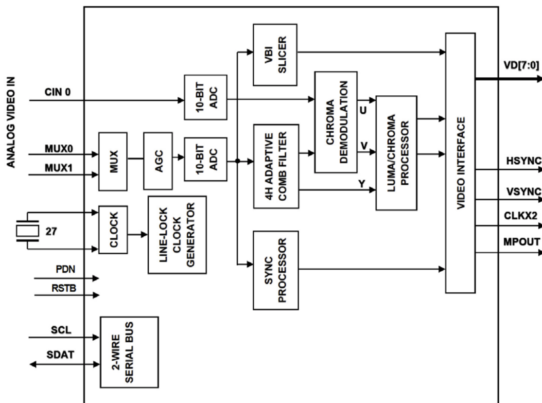
FIGURE 2. BLOCK DIAGRAM
