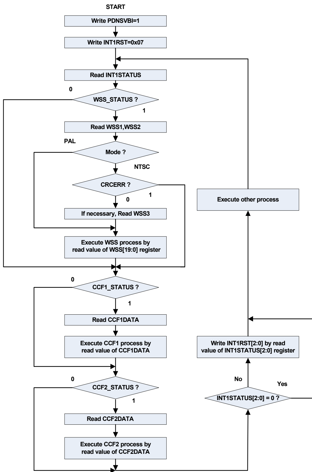
FIGURE 7. VBI RECEIVED DATA REGISTER ACCESS
