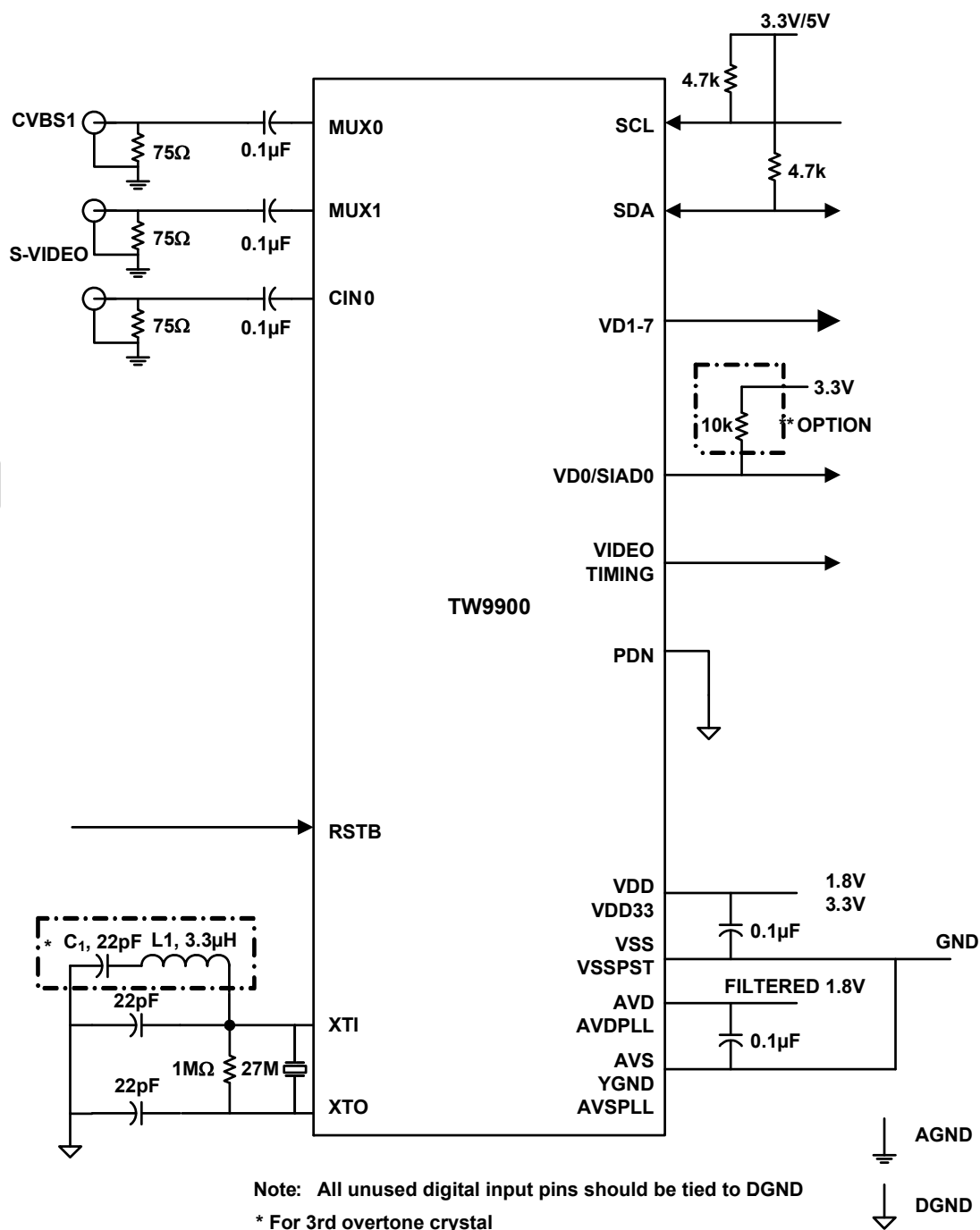
FIGURE 1. TYPICAL TW9900 EXTERNAL CIRCUITRY
