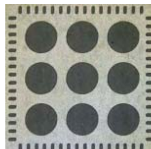
FIGURE 20C. RECOMMEND COVERAGE 65% FIGURE 20. STENCIL RECOMMENDED COVERAGE
