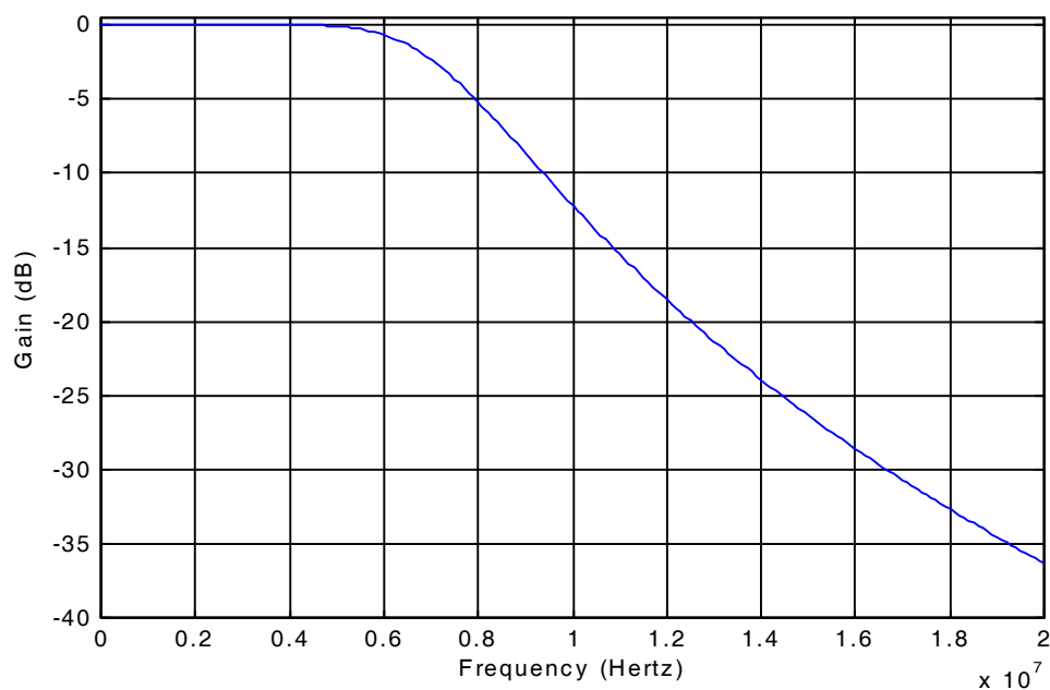
FIGURE 11. ANTI-ALIAS FILTER
