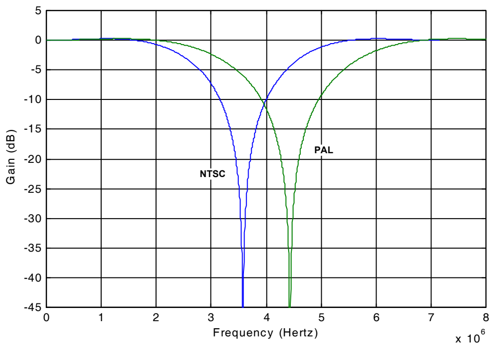
FIGURE 14. LUMA NOTCH FILTER CURVE FOR NTSC AND PAL/SECAM
