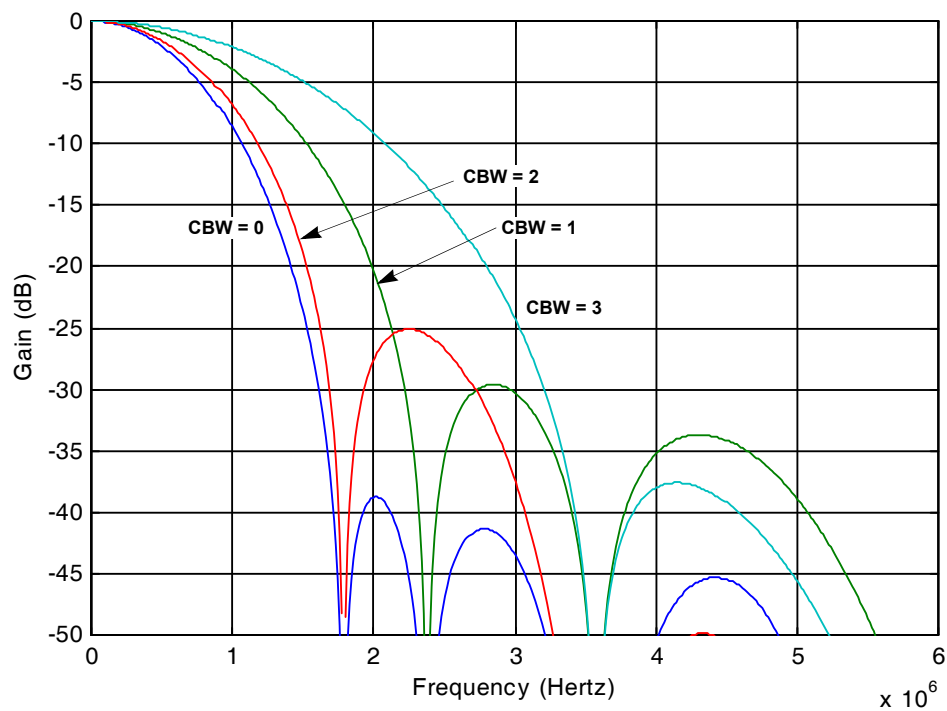
FIGURE 15. CHROMINANCE LOW-PASS FILTER CURVE
