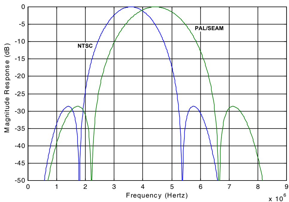
FIGURE 13. CHROMA BAND PASS FILTER CURVES
