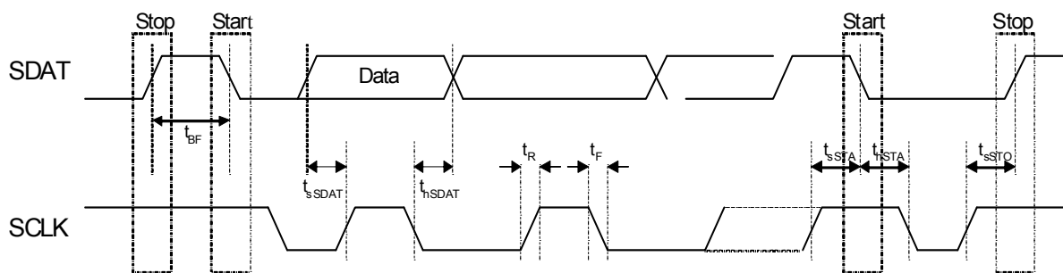
FIGURE 4. SERIAL HOST INTERFACE TIMING DIAGRAM
