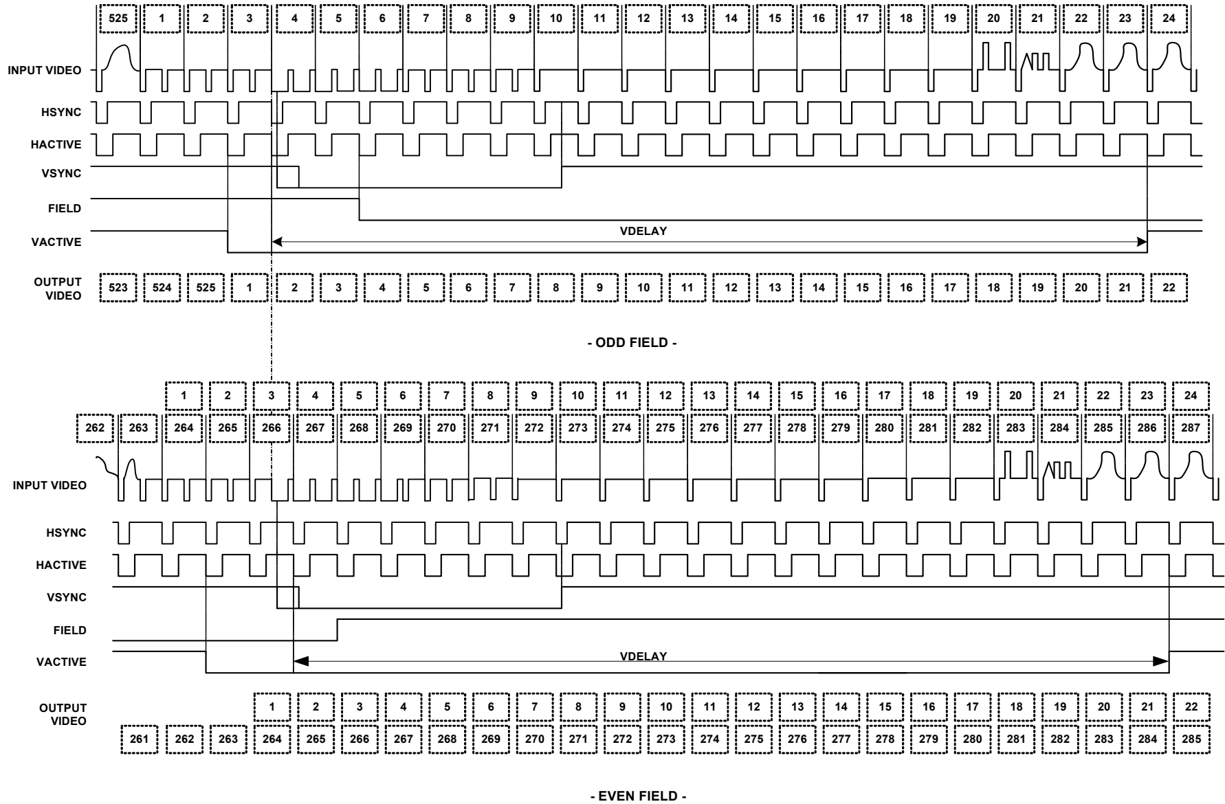
FIGURE 6. VERTICAL TIMING DIAGRAM FOR 60Hz/525 LINE SYSTEM
