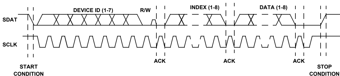
FIGURE 10. ONE COMPLETE REGISTER WRITE SEQUENCE VIA THE SERIAL BUS INTERFACE
