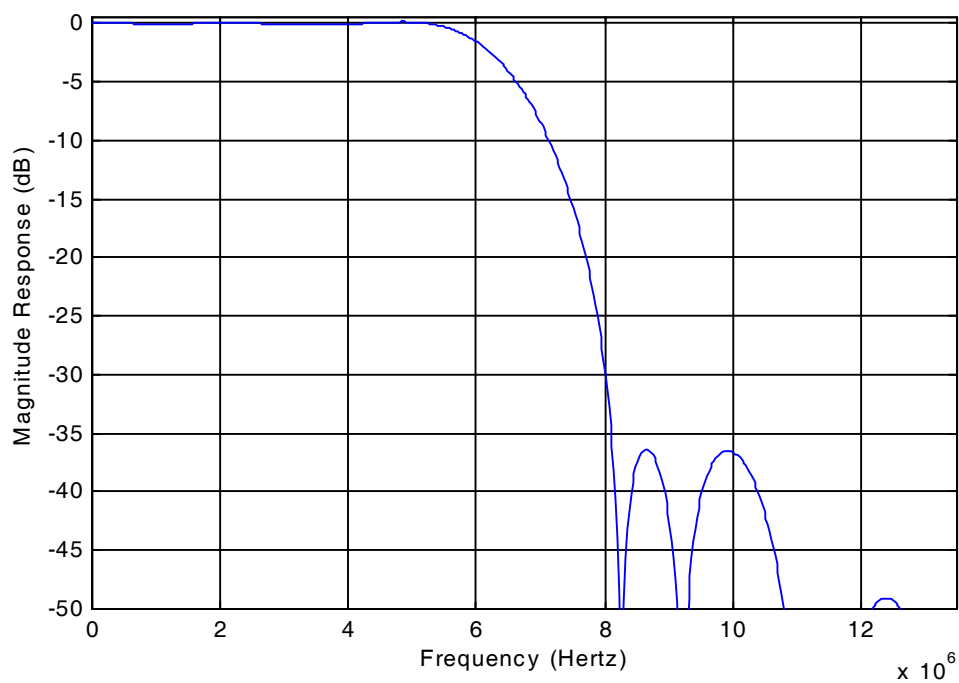
FIGURE 12. DECIMATION FILTER
