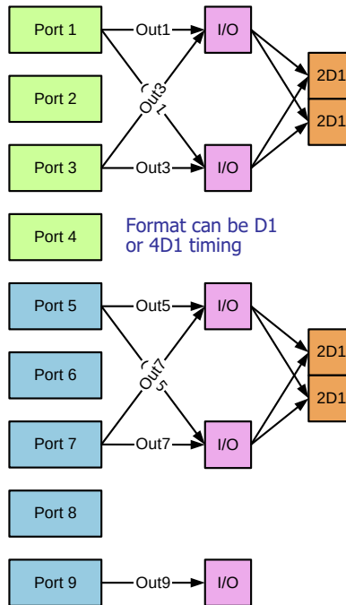
8 channel + Network 16b output @ 27 MHz
