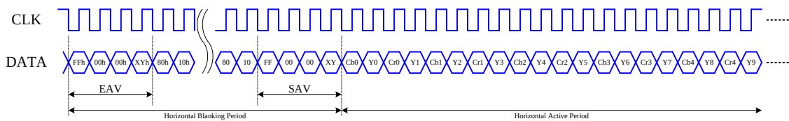
Timing Diagram of BT.656 format for digital video input
