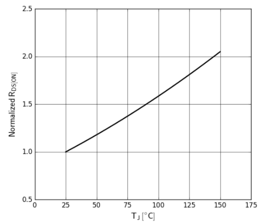
Figure 5. Normalized On-resistance
