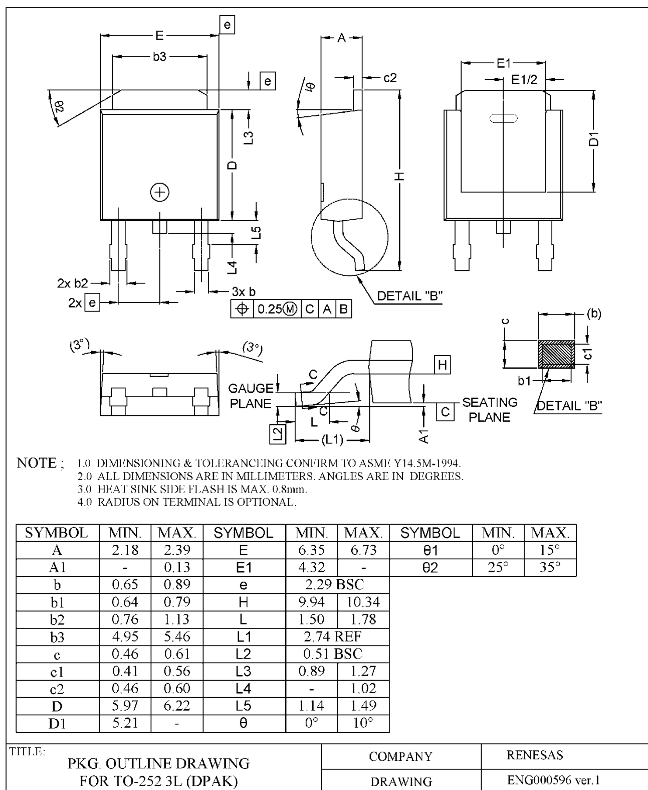
Figure 19. Package Outline Drawing – TO252-3L
