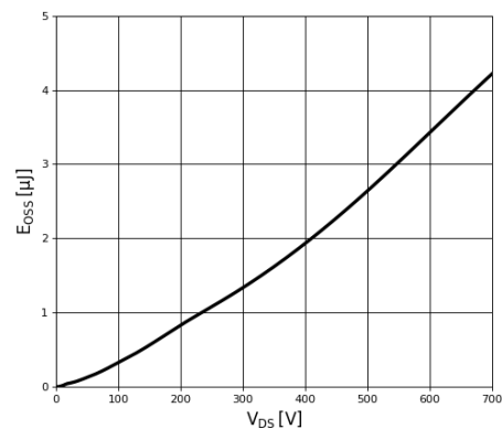
Figure 7. Typical C_{OSS} Stored Energy
