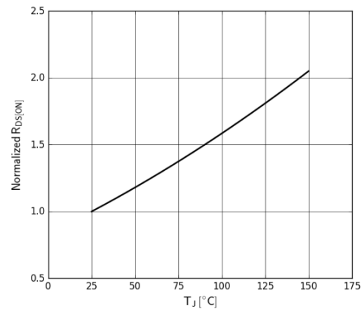
Figure 5. Normalized On-resistance
