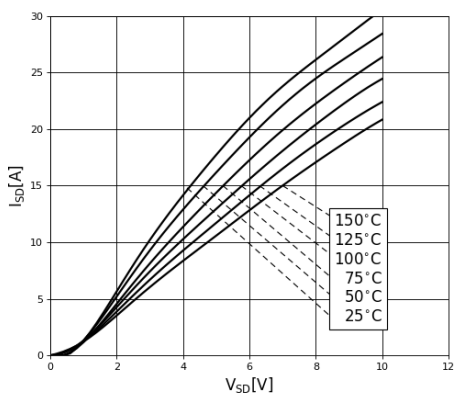
Figure 12. Forward Characteristics of Rev. Diode
