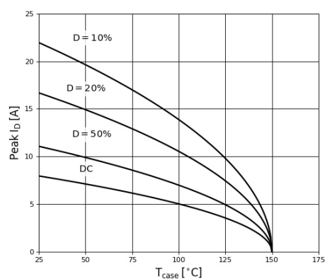
Figure 11. Current Derating
