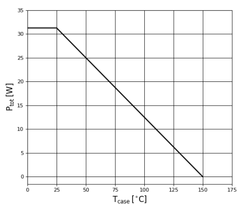
Figure 10. Power Dissipation
