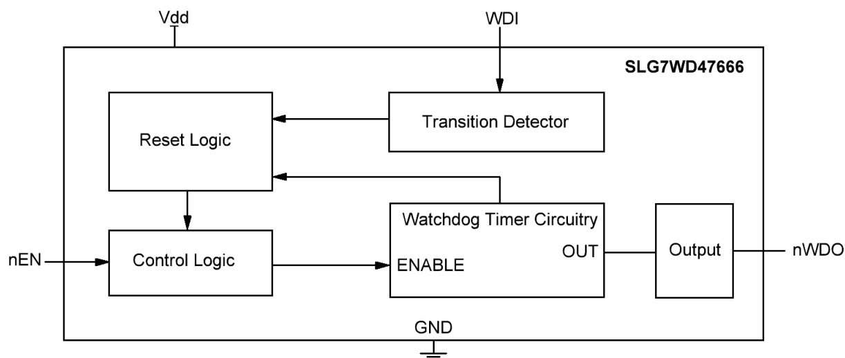
Figure 1. Functional Diagram
