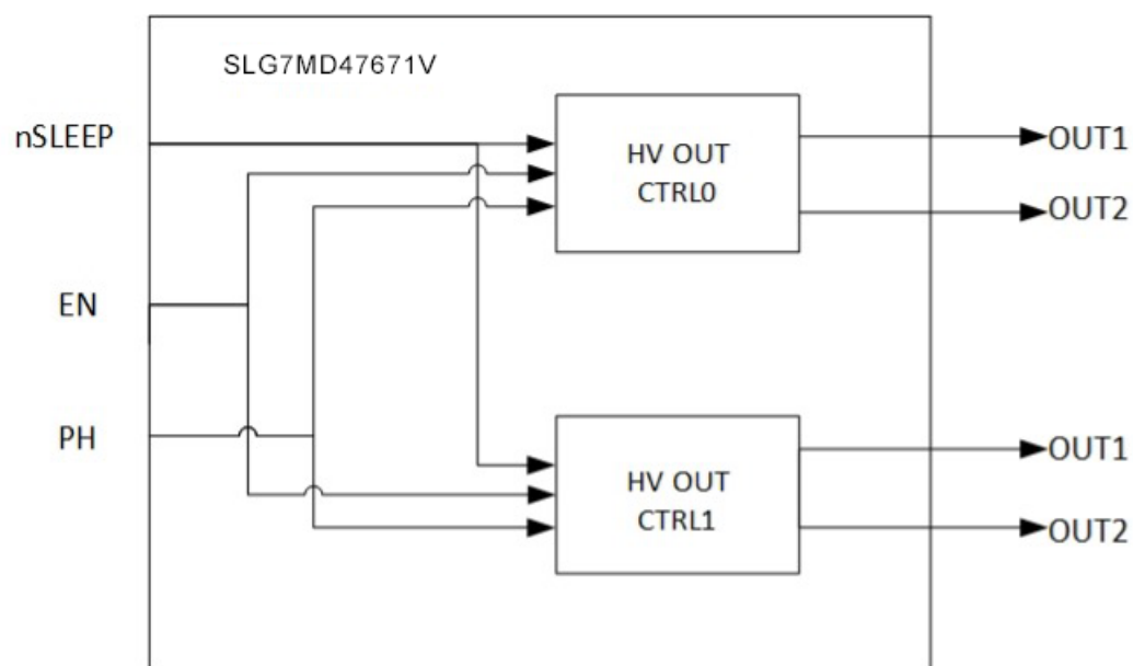
Figure 1. Functional Diagram
