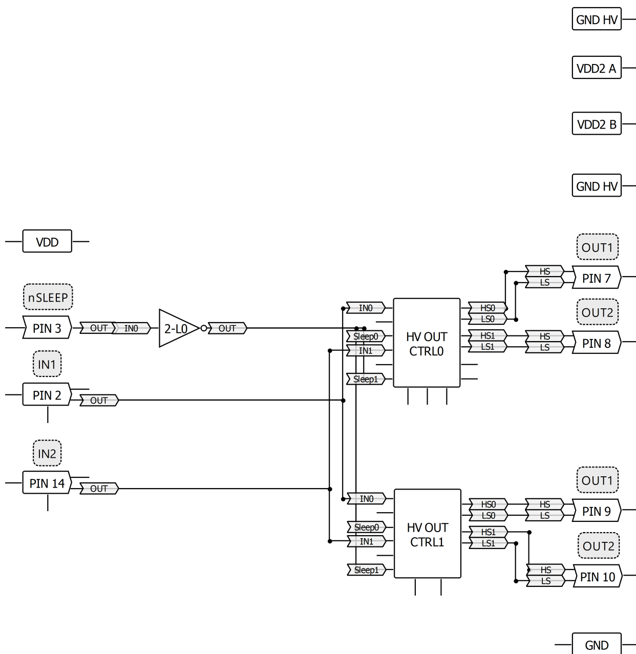
Figure 2. Block Diagram
