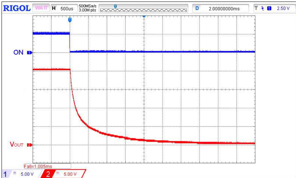
Figure 5. Typical Turn OFF operation waveform for V_{IN} = 20 V, C_{SLEW} = 10 nF, C_{LOAD} = 10 μF, R_{LOAD} = 100 Ω
