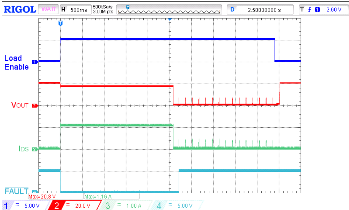
Figure 6. Thermally induced SOA shutdown for V_{IN} = 20 V, C_{LOAD} = 10 μF, I_{ACL} = 1 A, R_{SET} = 91 kΩ
