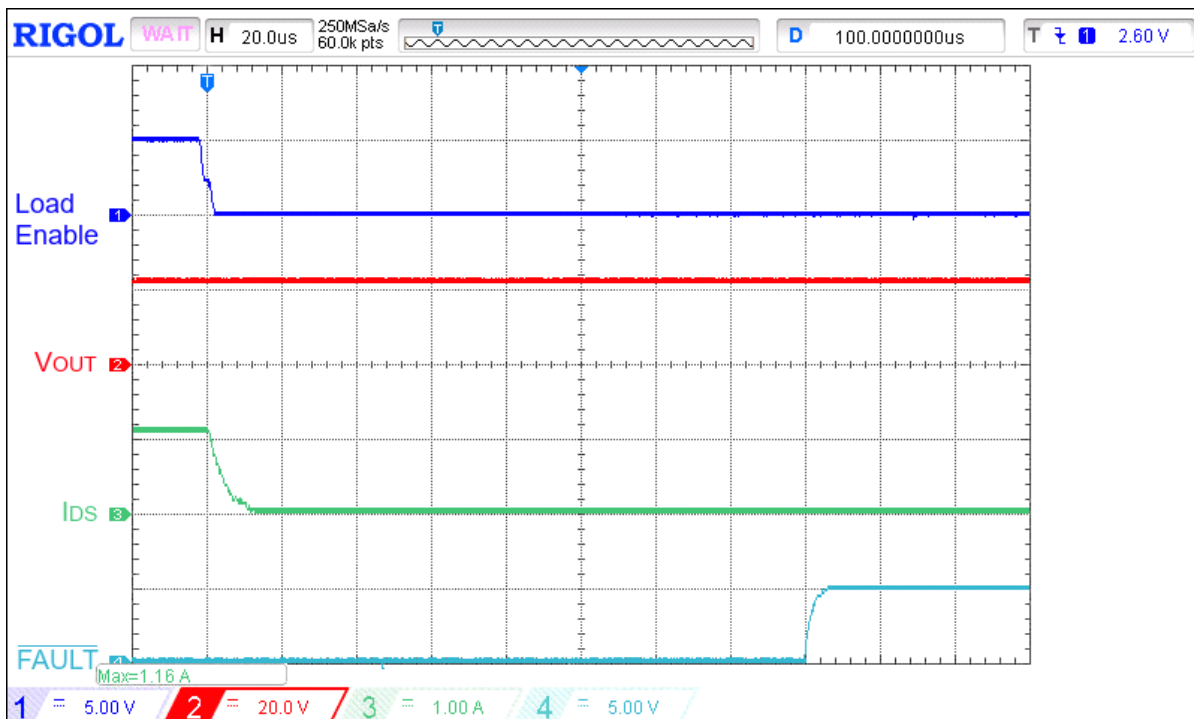
Figure 8. Typical FAULT de-assertion waveform for V_{IN} = 20 V, C_{LOAD} = 10 μF, I_{ACL} = 1 A, R_{SET} = 91 kΩ, switch out 20 Ω load
