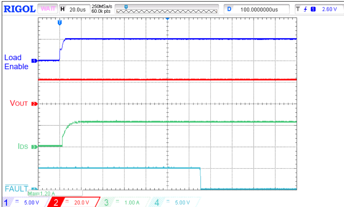
Figure 7. Typical FAULT assertion waveform for V_{IN} = 20 V, C_{LOAD} = 10 μF, I_{ACL} = 1 A, R_{SET} = 91 kΩ, switch in 20 Ω load
