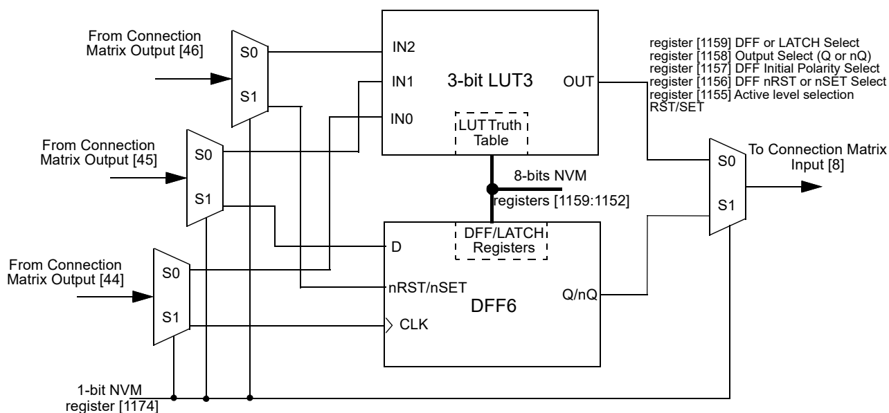
Figure 61. 3-bit LUT3 or DFF6
