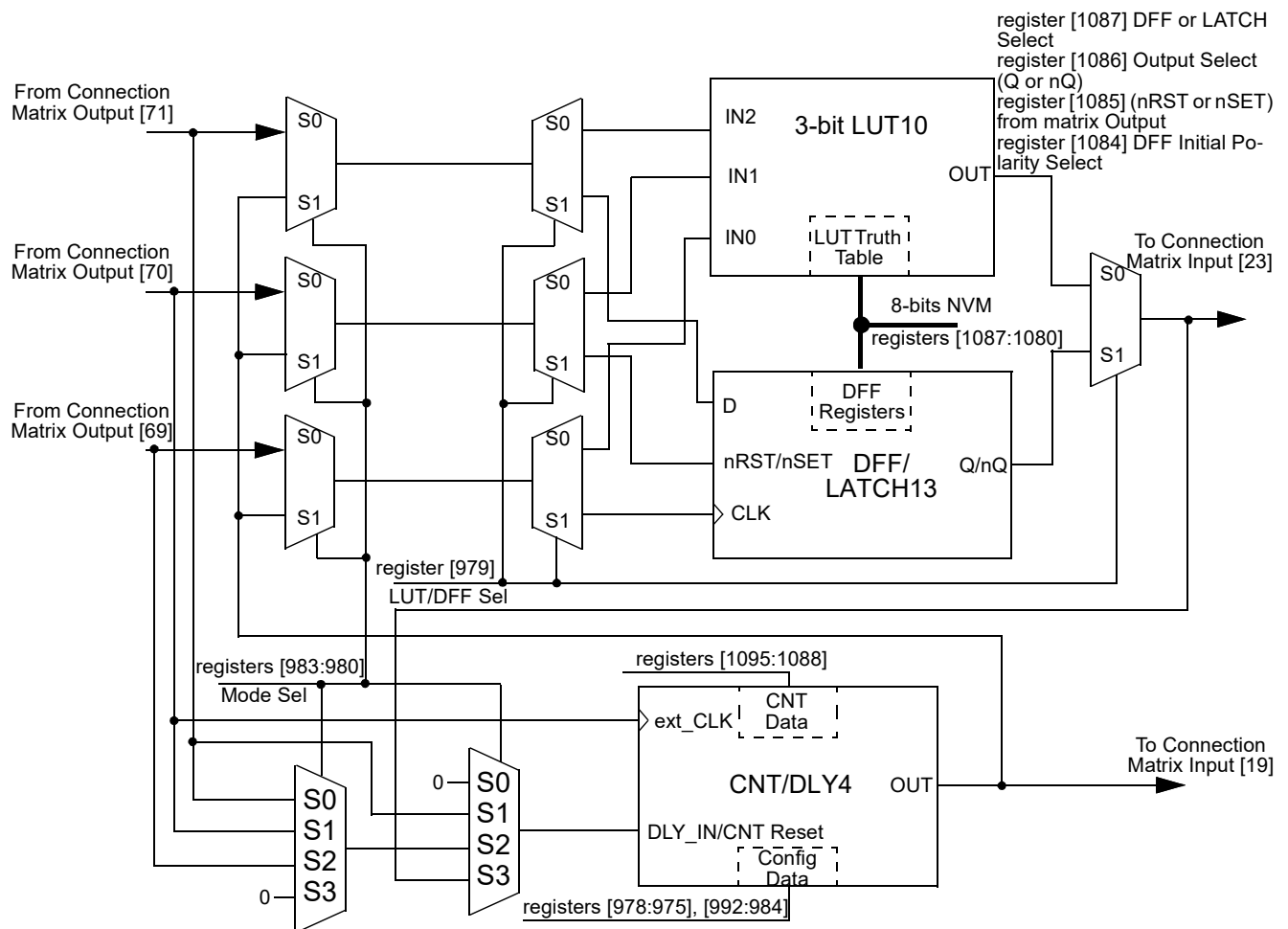
Figure 84. 8-bit Multi-Function Macrocells Block Diagram (3-bit LUT10/DFF13, CNT/DLY4)
