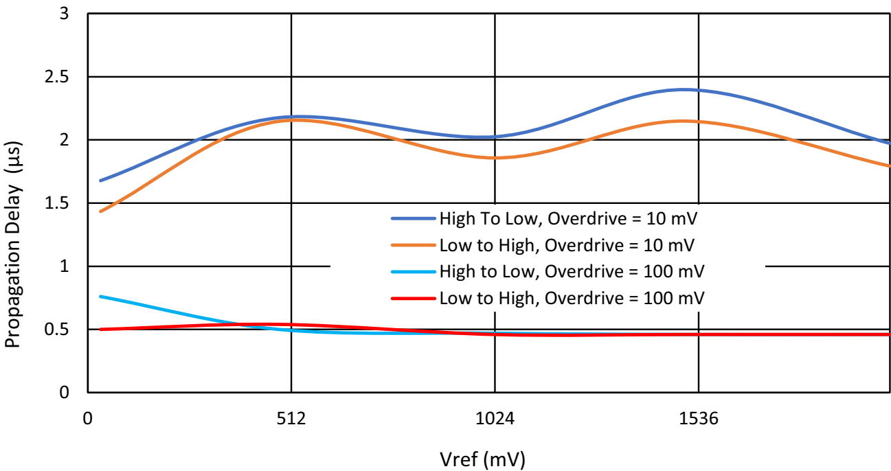
Figure 119. Propagation Delay vs. Vref for ACMPxH at T A = 25 °C, at V DD = 2.3 V to 5.5 V, Gain = 1, Hysteresis = 0
