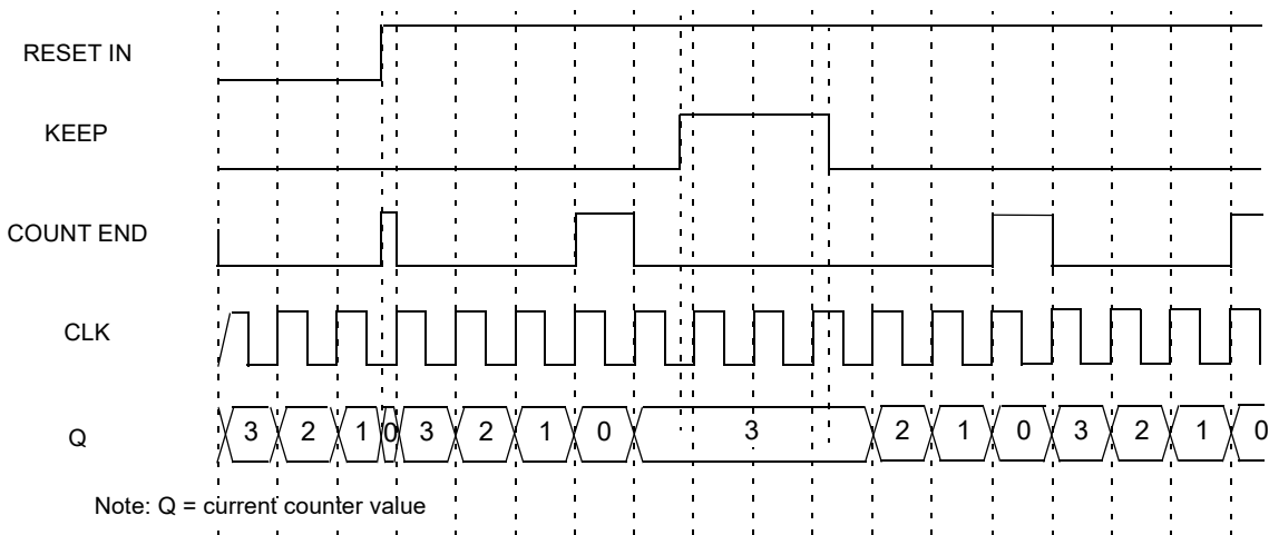
Figure 93. CNT/FSM Timing Diagram (Reset Rising Edge Mode, Oscillator is Forced On, UP = 0) for Counter Data = 3
