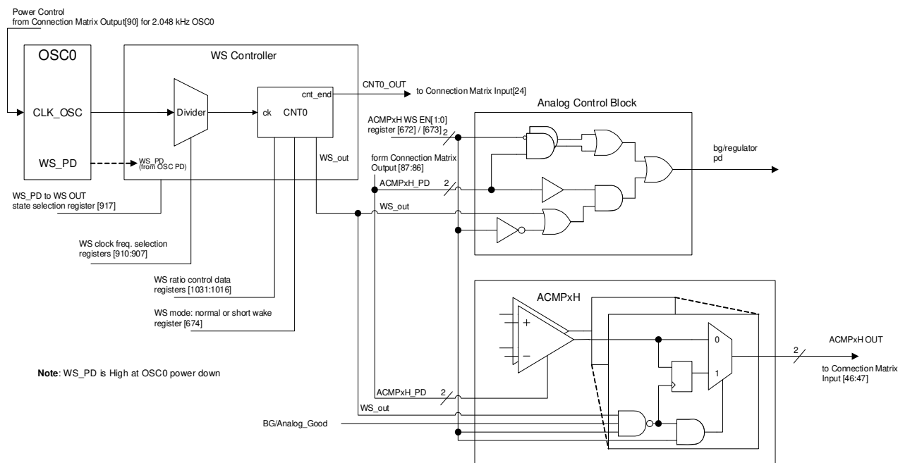
Figure 99. Wake/Sleep Controller
