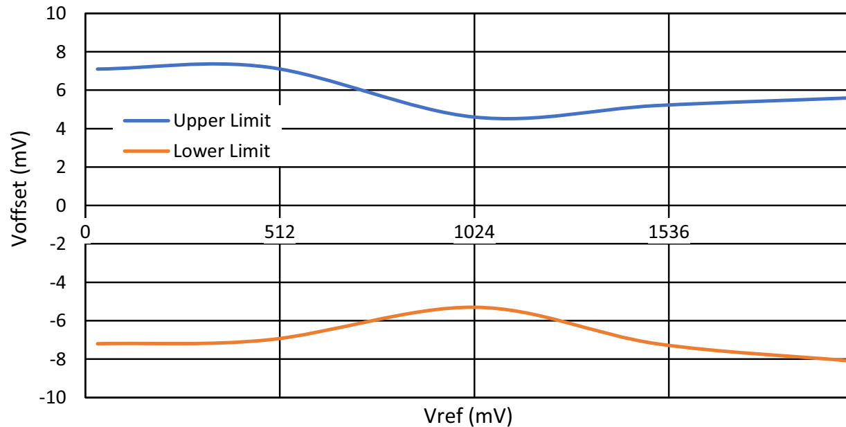
Figure 112: ACMPxH Input Offset Voltage vs. Vref at V_{DD} = 2.3 \text{ V to } 5.5 \text{ V} , T = -40^\circ \text{C to } 85^\circ \text{C}
