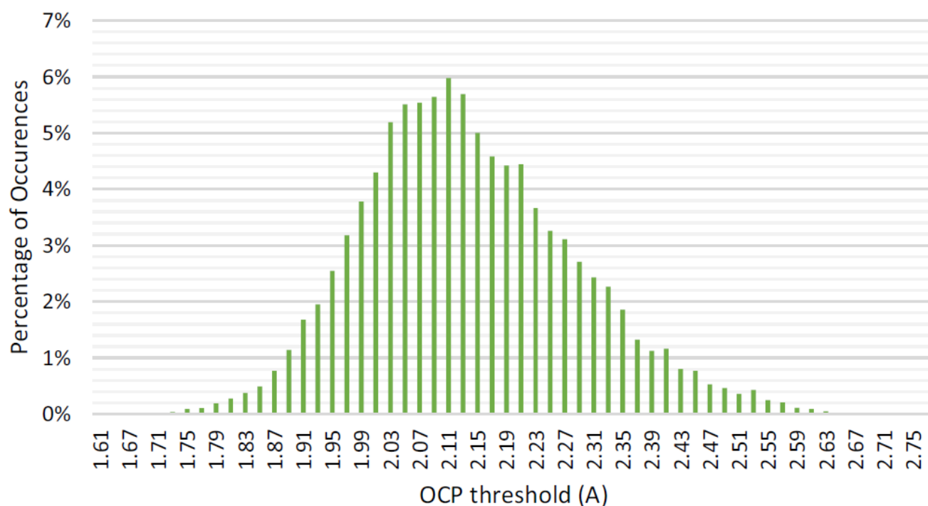
Figure 26. Full Bridge High Side OCP Threshold Distribution at V_{DD} = 2.3 \text{ V to } 5.5 \text{ V} , V_{DD2} = 3 \text{ V to } 13.2 \text{ V} , T_J = -40 \text{ }^{\circ}\text{C to } +150 \text{ }^{\circ}\text{C}
