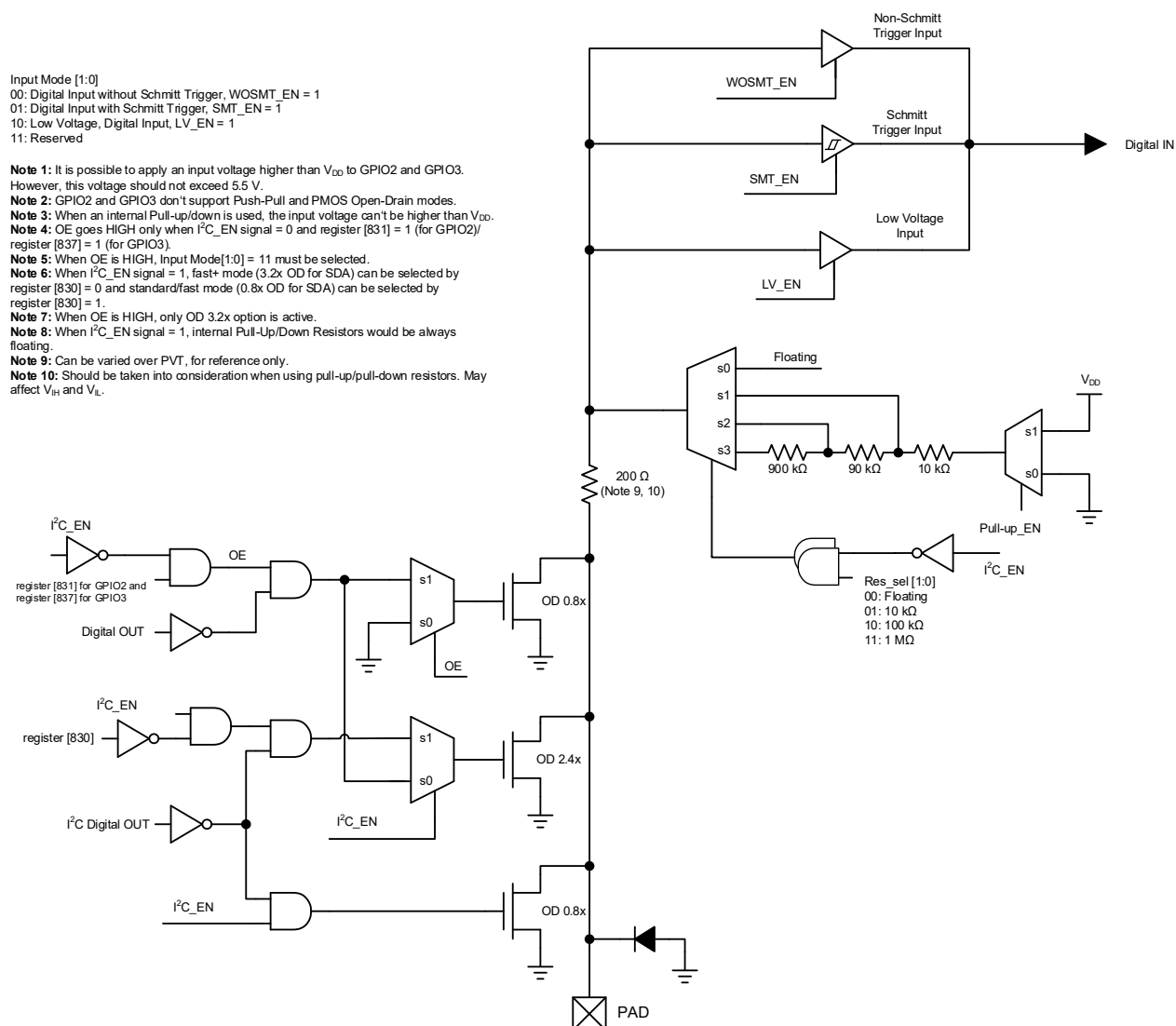
Figure 5. GPIO with I 2 C Mode Structure Diagram
