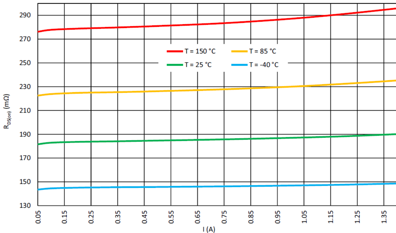
Figure 19. Full Bridge Typical Drain-Source Low Side On-Resistance vs. Load Current at V_{DD} = 5.5\text{ V} , V_{DD2} = 5\text{ V}
