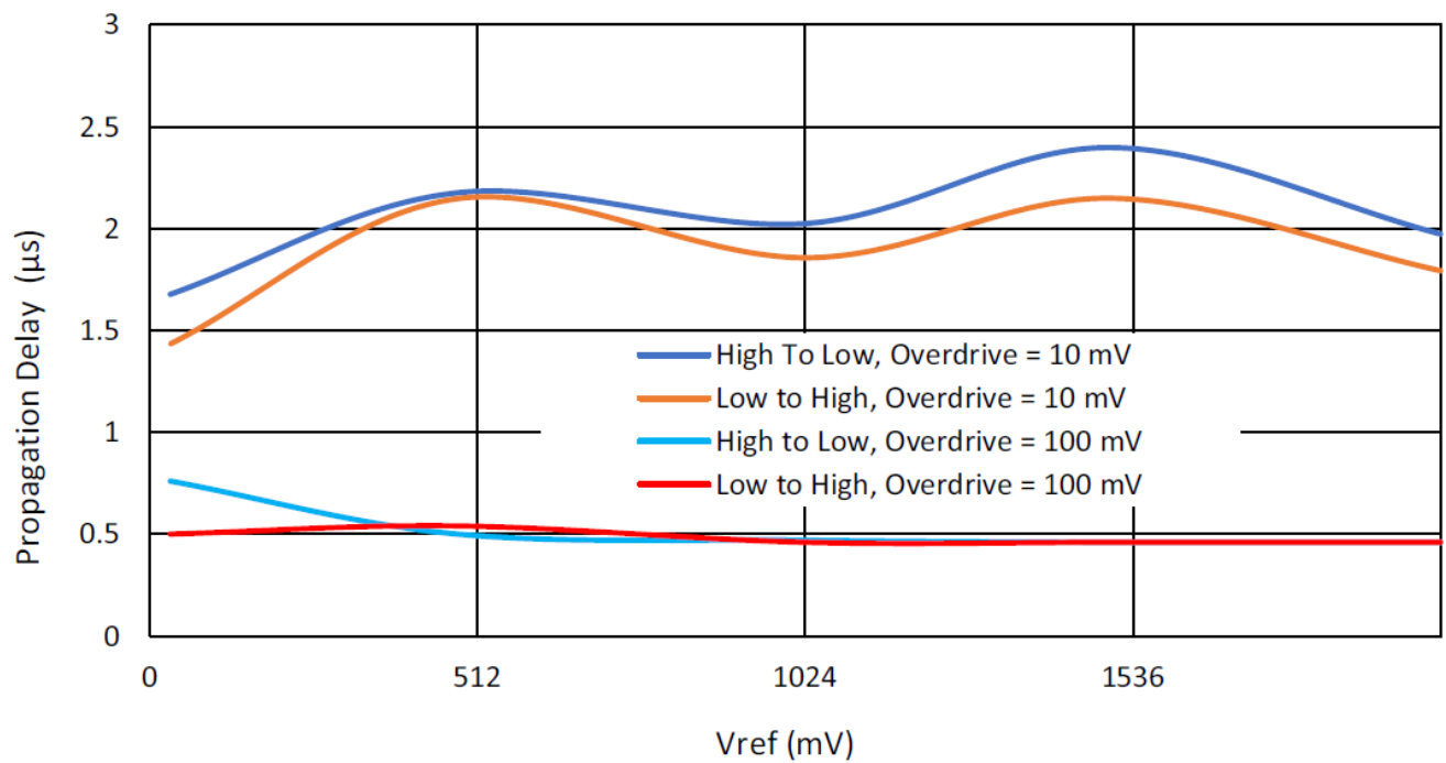
Figure 98. Propagation Delay vs. VREF for ACMPH at T = +25 °C, at VDD = 2.3 V to 5.5 V, Gain = 1, Hysteresis = 0
