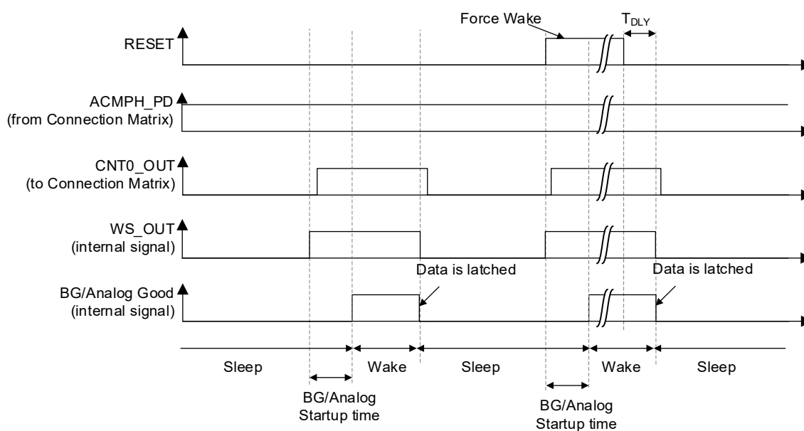
Figure 80. Wake/Sleep Controller
