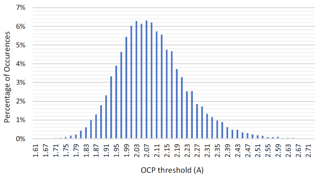
Figure 27. Full Bridge Low Side OCP Threshold Distribution at V_{DD} = 2.3 \text{ V to } 5.5 \text{ V} , V_{DD2} = 3 \text{ V to } 13.2 \text{ V} , T_J = -40 \text{ }^{\circ}\text{C to } +150 \text{ }^{\circ}\text{C}
