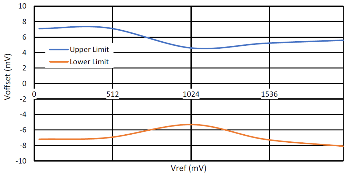
Figure 97. ACMPH Input Offset Voltage vs. VREF at VDD = 2.3 V to 5.5 V, T = -40 °C to +85 °C
