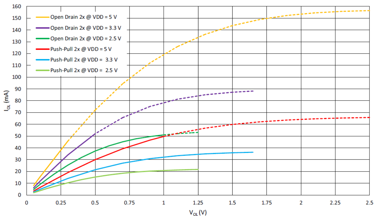
Figure 11. Typical Low Level Output Current vs. Low Level Output Voltage, 2x Drive at T = +25\text{ }^{\circ}\text{C} , Full Range
