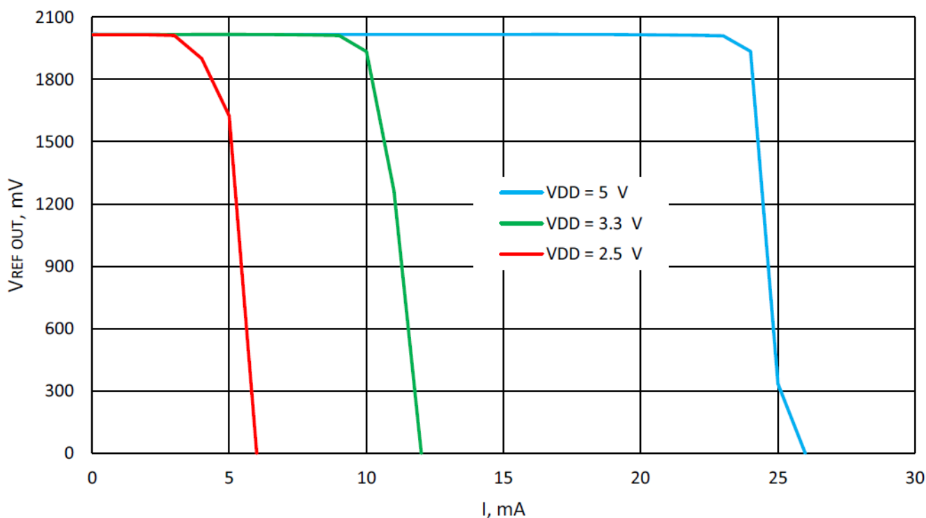
Figure 108. Typical Load Regulation, V_{REF} = 2016 \text{ mV} , T = -40^\circ\text{C} to +85^\circ\text{C} , Buffer – Enabled
