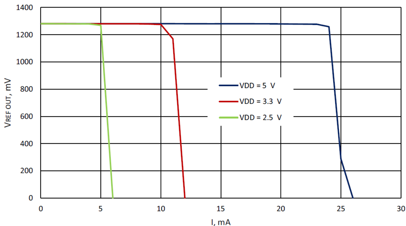
Figure 107. Typical Load Regulation, V_{REF} = 1280 \text{ mV} , T = -40^\circ\text{C} to +85^\circ\text{C} , Buffer – Enabled
