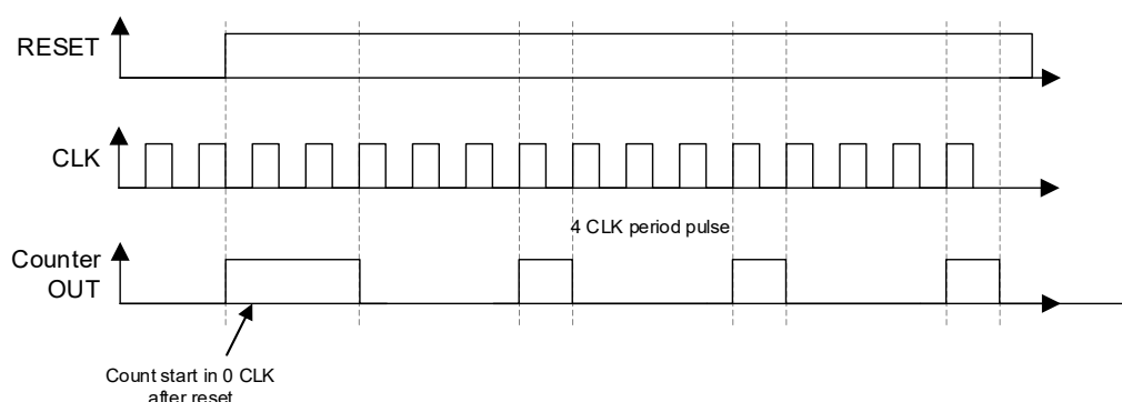
Figure 70. Counter Mode Timing Diagram with Two DFFs Synced Up
