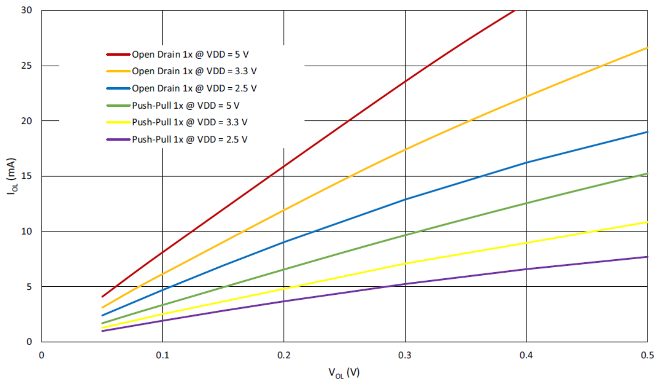
Figure 10. Typical Low Level Output Current vs. Low Level Output Voltage, 1x Drive at T = +25\text{ }^{\circ}\text{C}
