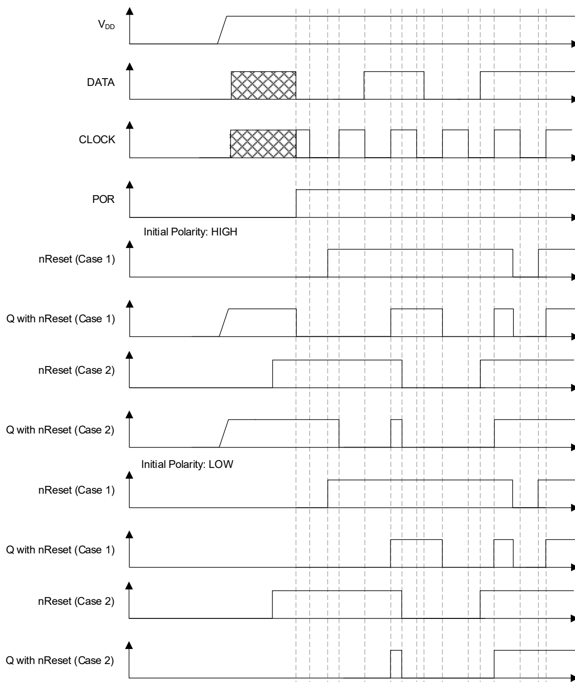
Figure 58. DFF Polarity Operations with n\text{Reset}
