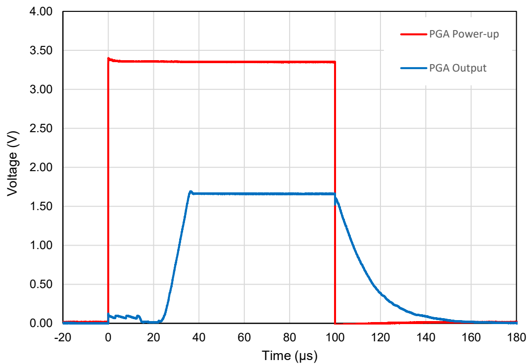
Figure 102. Output Response to Power-Down Signal at T_A = +25\text{ }^{\circ}\text{C} , V_{DD} = 3.3\text{ V}
