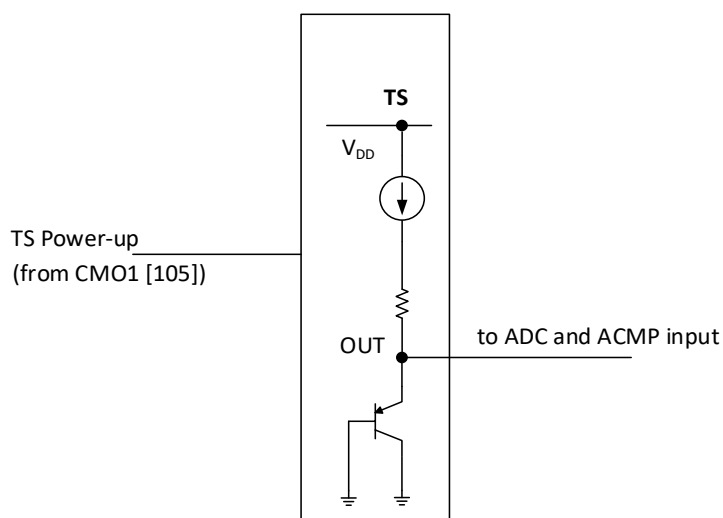
Figure 219. Analog Temperature Sensor Structure Diagram
