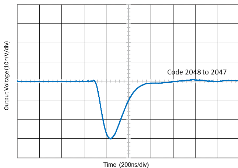
Figure 135. Worst Case Glitch Response at T_A = +25^\circ\text{C} , V_{DD} = 1.8\text{ V} , V_{REF} = 1.62\text{ V} (Internal), DAC Buffer ON
