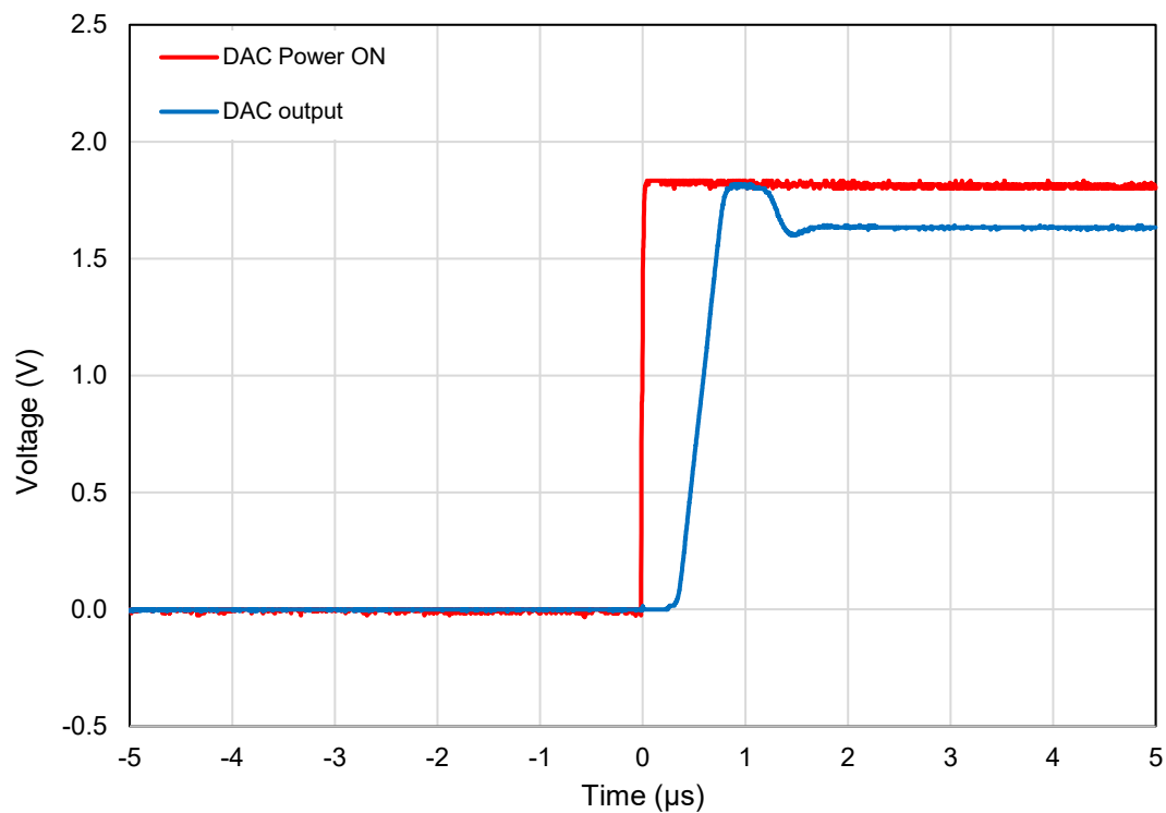
Figure 134. Wake-Up Time/Full-Scale Settling Time at T_A = +25^\circ\text{C} , V_{DD} = 1.8\text{ V} , V_{REF} = 1.62\text{ V} (Internal), DAC Buffer ON
