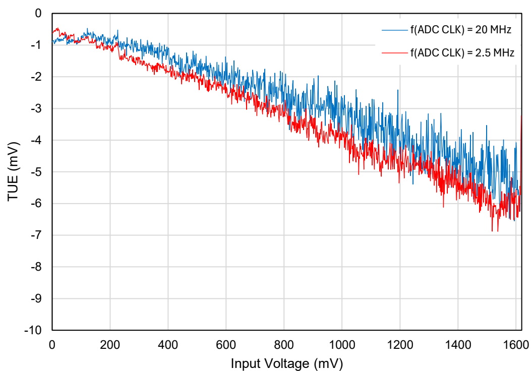
Figure 126. Total Unadjusted Error (TUE) vs. Input Voltage at T_A = +25\text{ }^{\circ}\text{C} , V_{DD} = 3.3\text{ V} , Resolution = 14 bit, V_{REF} = 1.62\text{ V} (Internal). Typical TUE without ADC system calibration.
