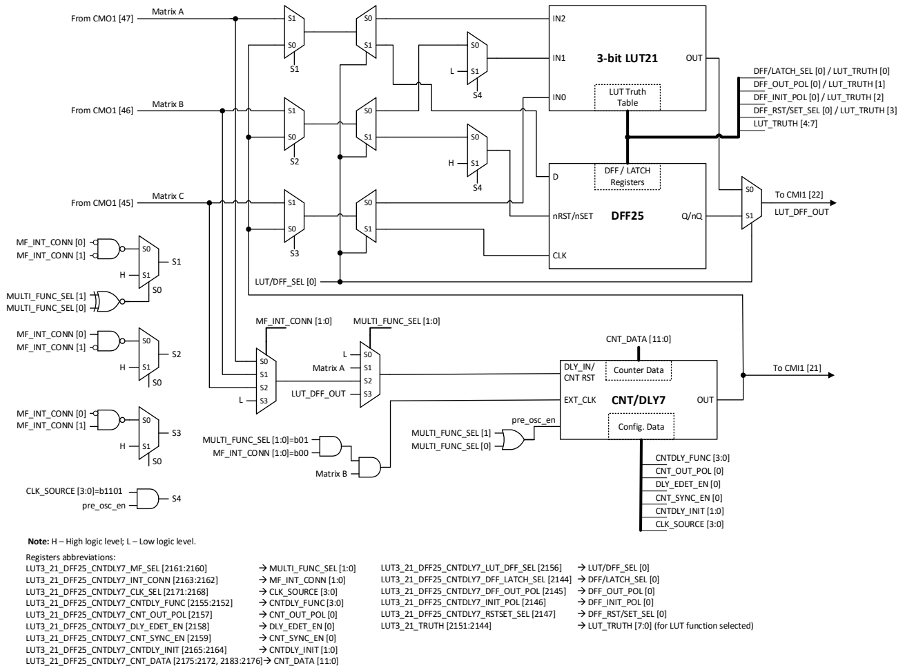
Figure 48. 12-bit Multi-Function Macrocells Block Diagram (3-bit LUT21/DFF25, CNT/DLY7)
