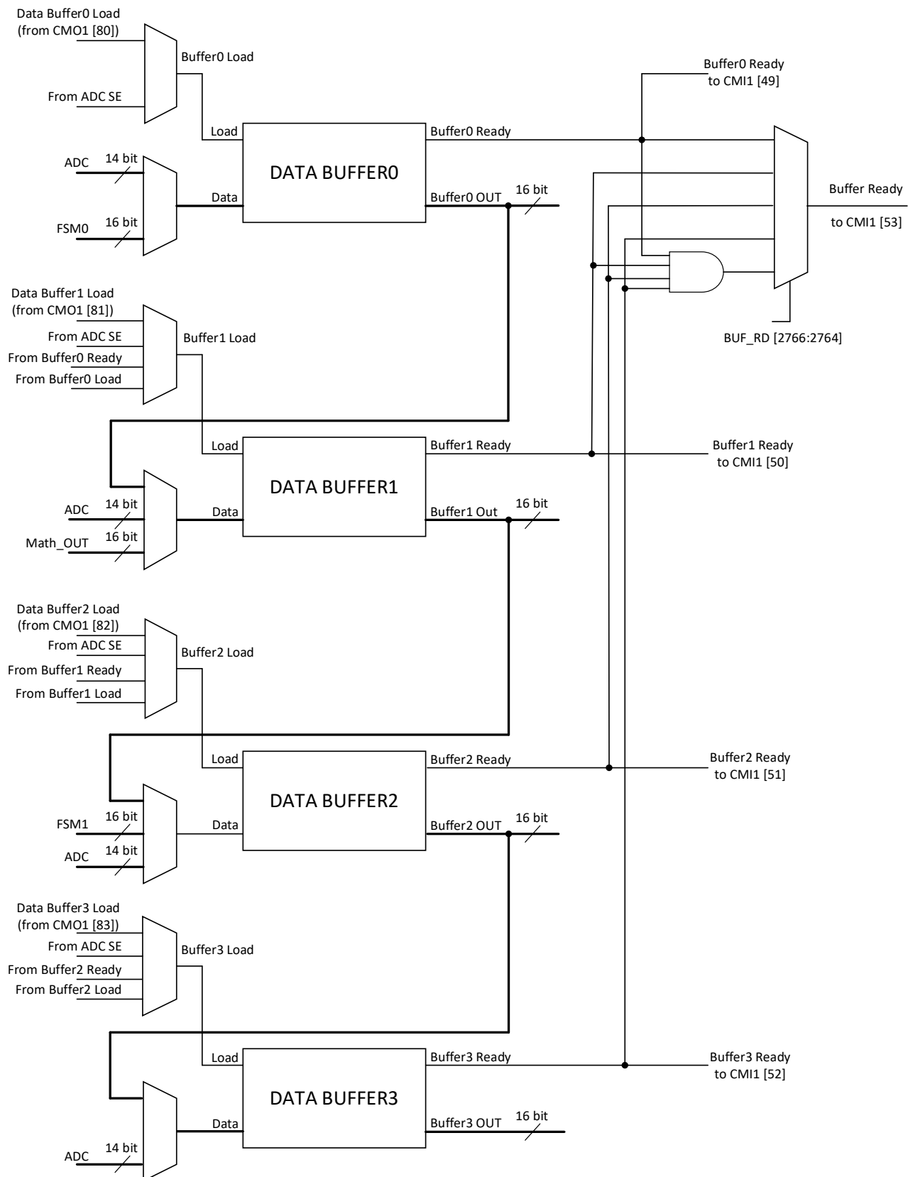
Figure 146. Data Buffers Structure Diagram
