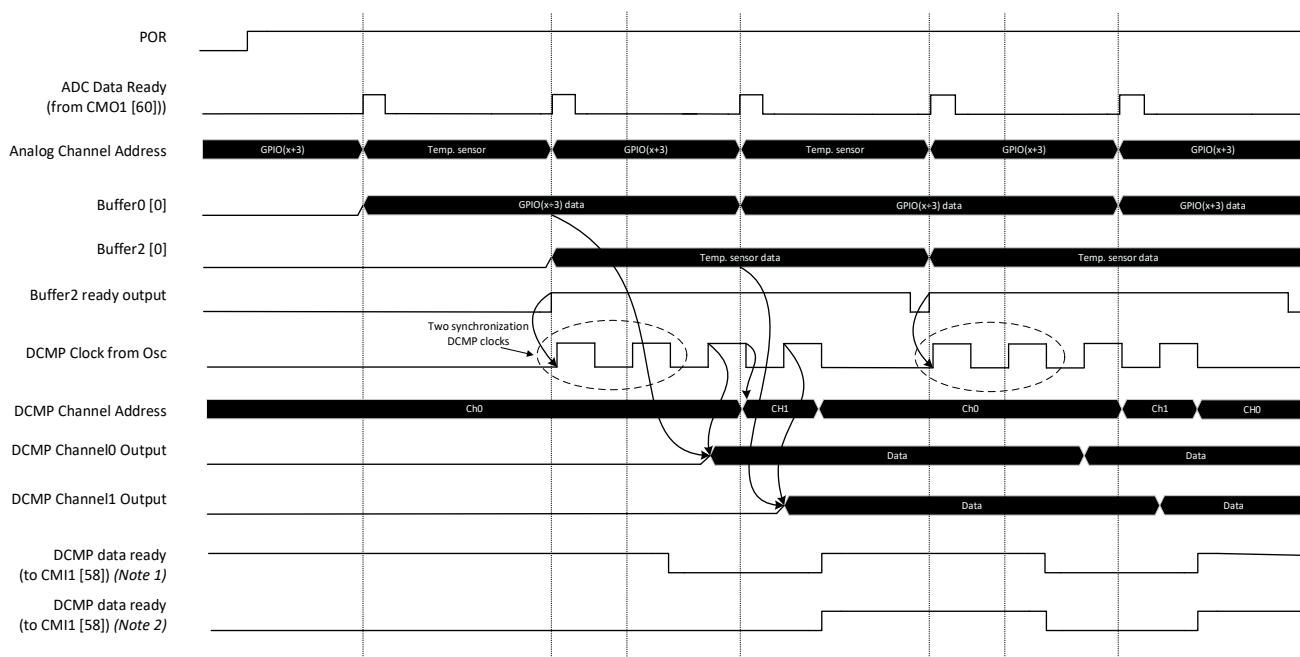
Figure 158. Multichannel DCMP Operation in Continuous Mode
