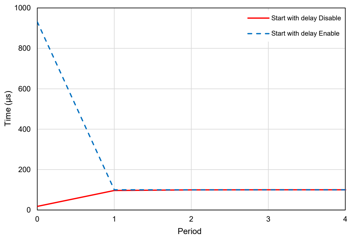
Figure 193. Oscillator0 Settling Time, OSC0 = 10 kHz at T_A = +25^\circ\text{C} , V_{DD} = 3.3\text{ V}
