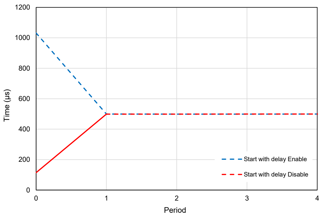
Figure 192. Oscillator0 Settling Time, OSC0 = 2 kHz at T_A = +25^\circ\text{C} , V_{DD} = 3.3\text{ V}
