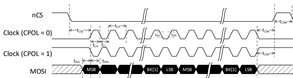
Figure 218. SPI Timing Diagram (CPHA = 0)
