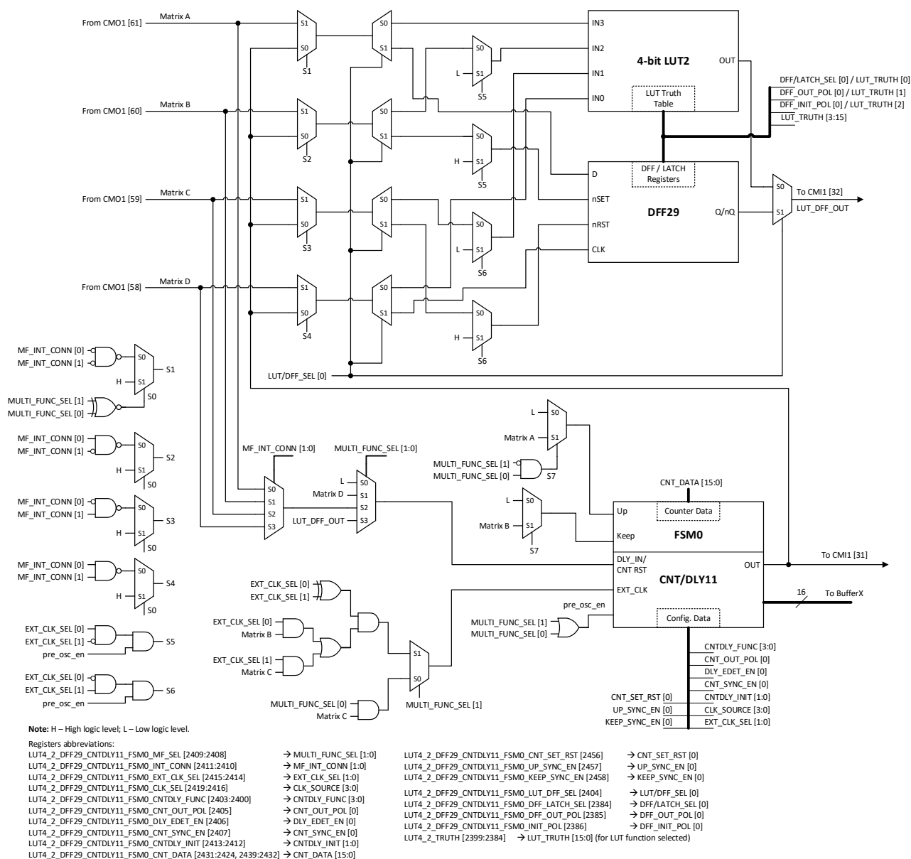
Figure 66. 4-bit LUT2 or DFF29, or CNT/DLY11/FSM0 Macrocell
