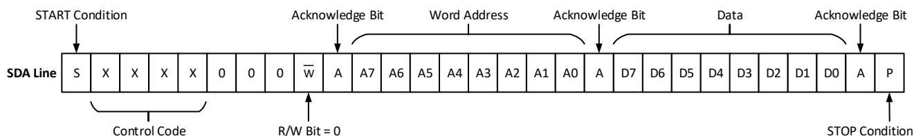
Figure 105. Byte Write Command, R/W = 0
