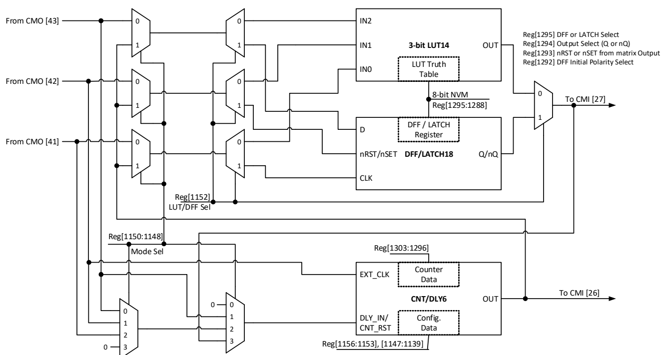
Figure 45. 8-bit Multi-Function Macrocells Block Diagram (3-bit LUT14/DFF18, CNT/DLY6)
