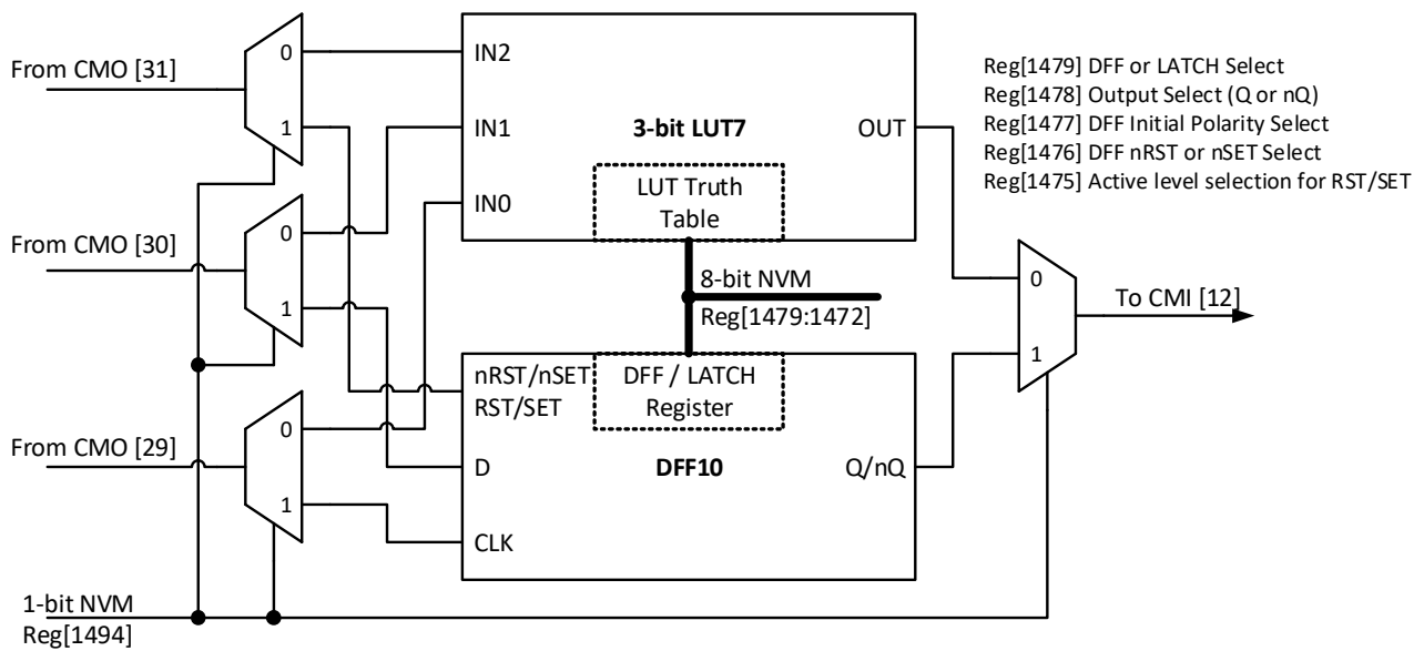
Figure 32. 3-bit LUT7 or DFF10
