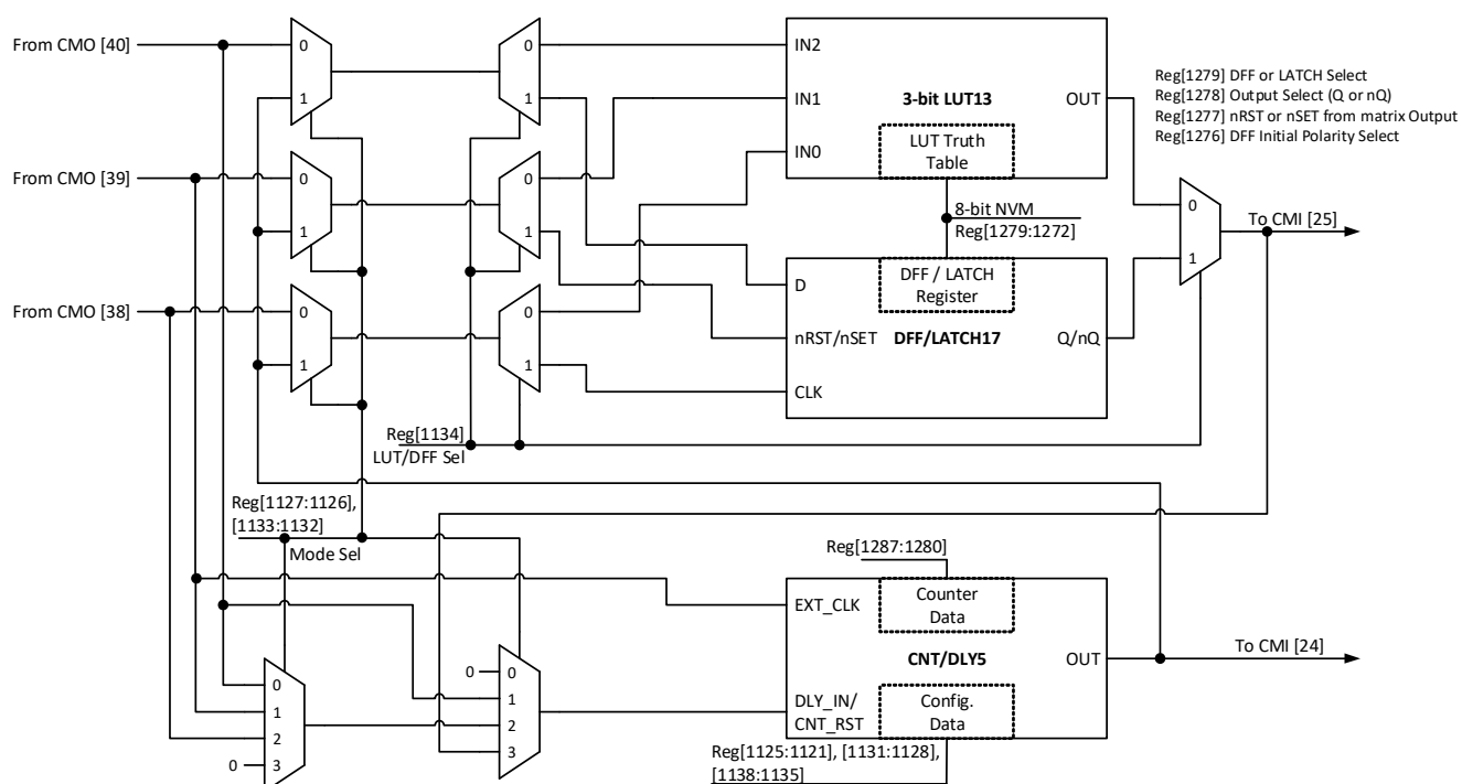
Figure 44. 8-bit Multi-Function Macrocells Block Diagram (3-bit LUT13/DFF17, CNT/DLY5)
