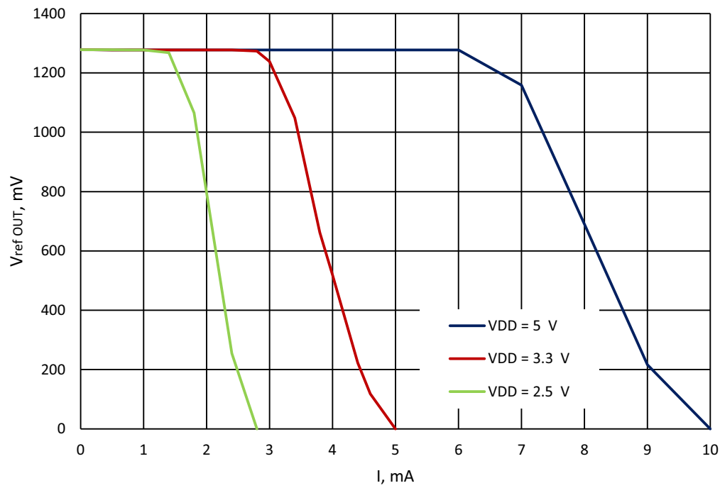
Figure 82. Typical Load Regulation, V_{ref} = 1280 \text{ mV} , T = -40^\circ\text{C} to +105^\circ\text{C} , Buffer - Enabled
