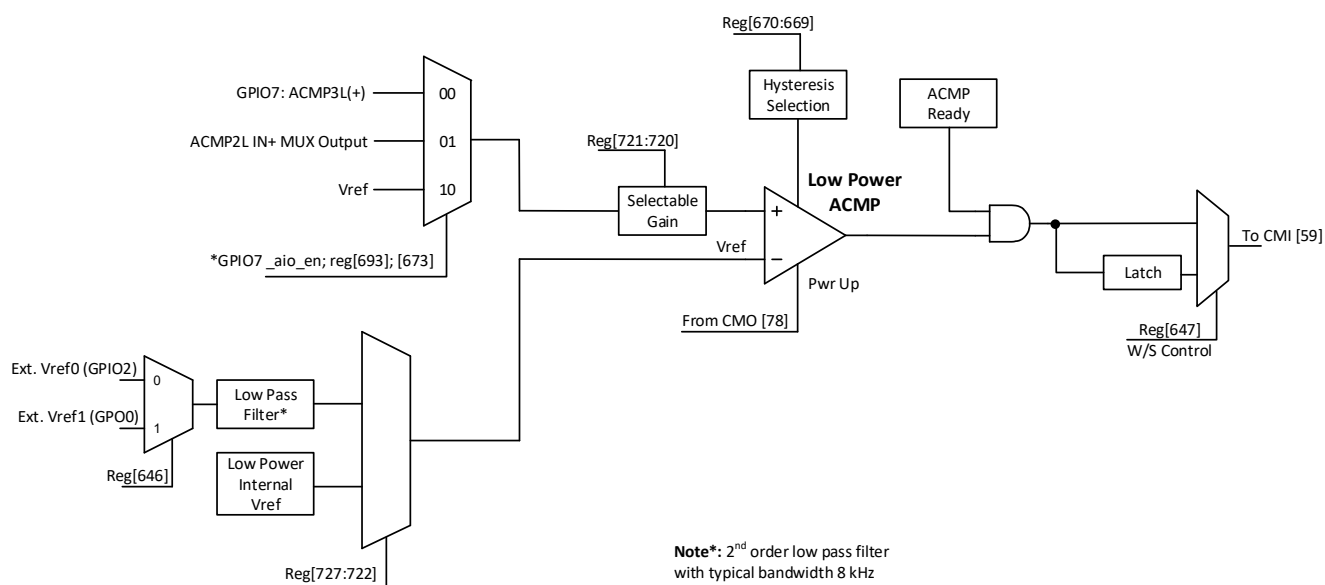
Figure 69. ACMP3L Block Diagram
