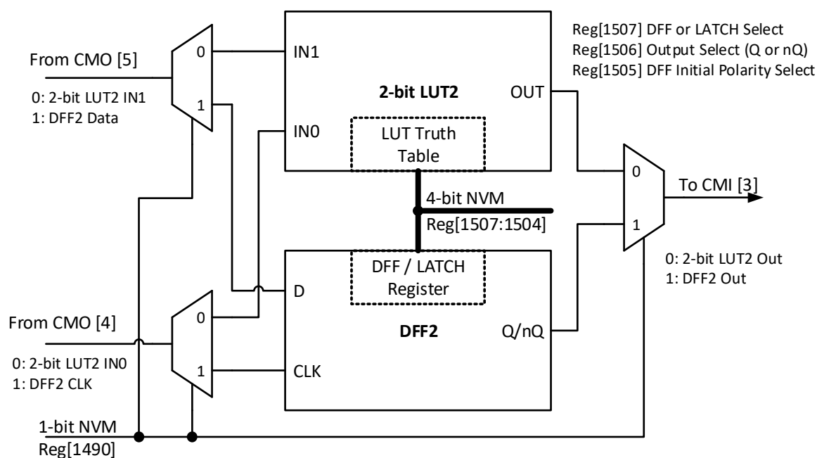
Figure 21. 2-bit LUT2 or DFF2
