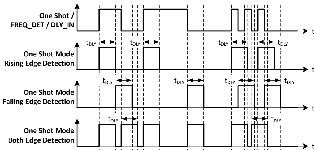
Figure 52. One-Shot Function Timing Diagram
