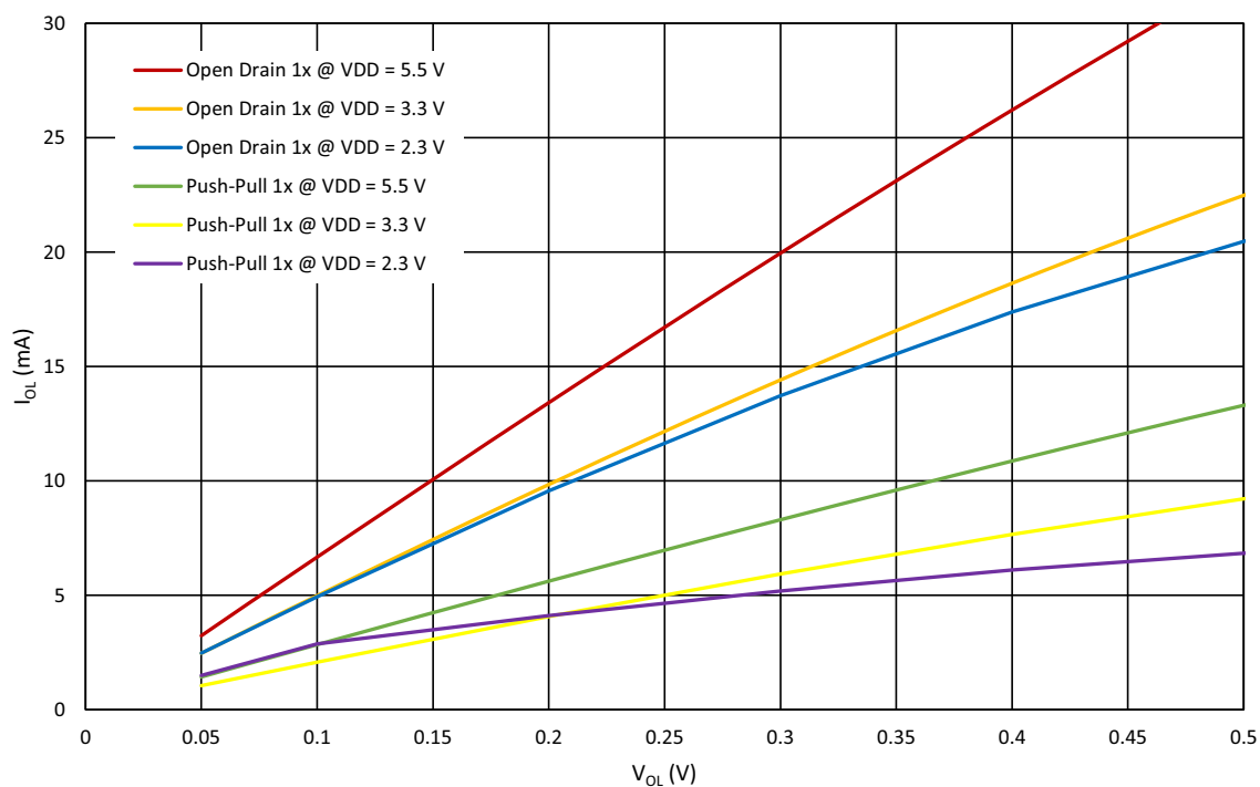
Figure 10. Typical Low Level Output Current vs. Low Level Output Voltage, 1x Drive at T_A = 25\text{ }^{\circ}\text{C}
