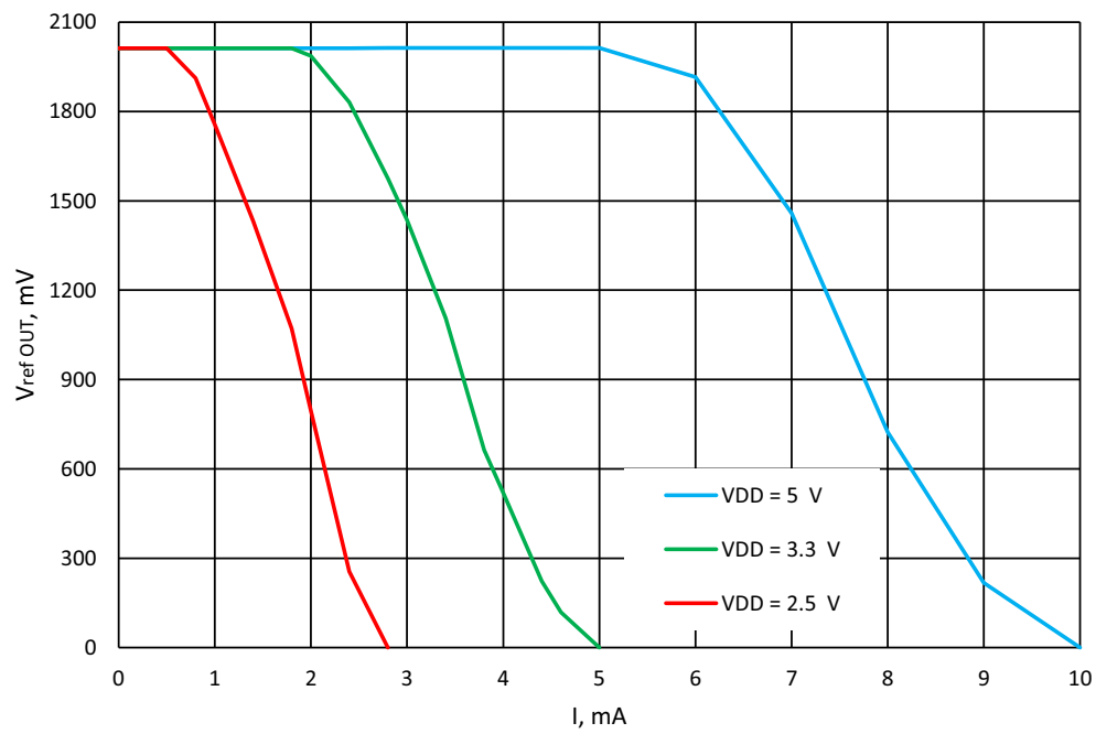
Figure 83. Typical Load Regulation, V_{ref} = 2016 \text{ mV} , T = -40^\circ\text{C} to +105^\circ\text{C} , Buffer - Enabled
