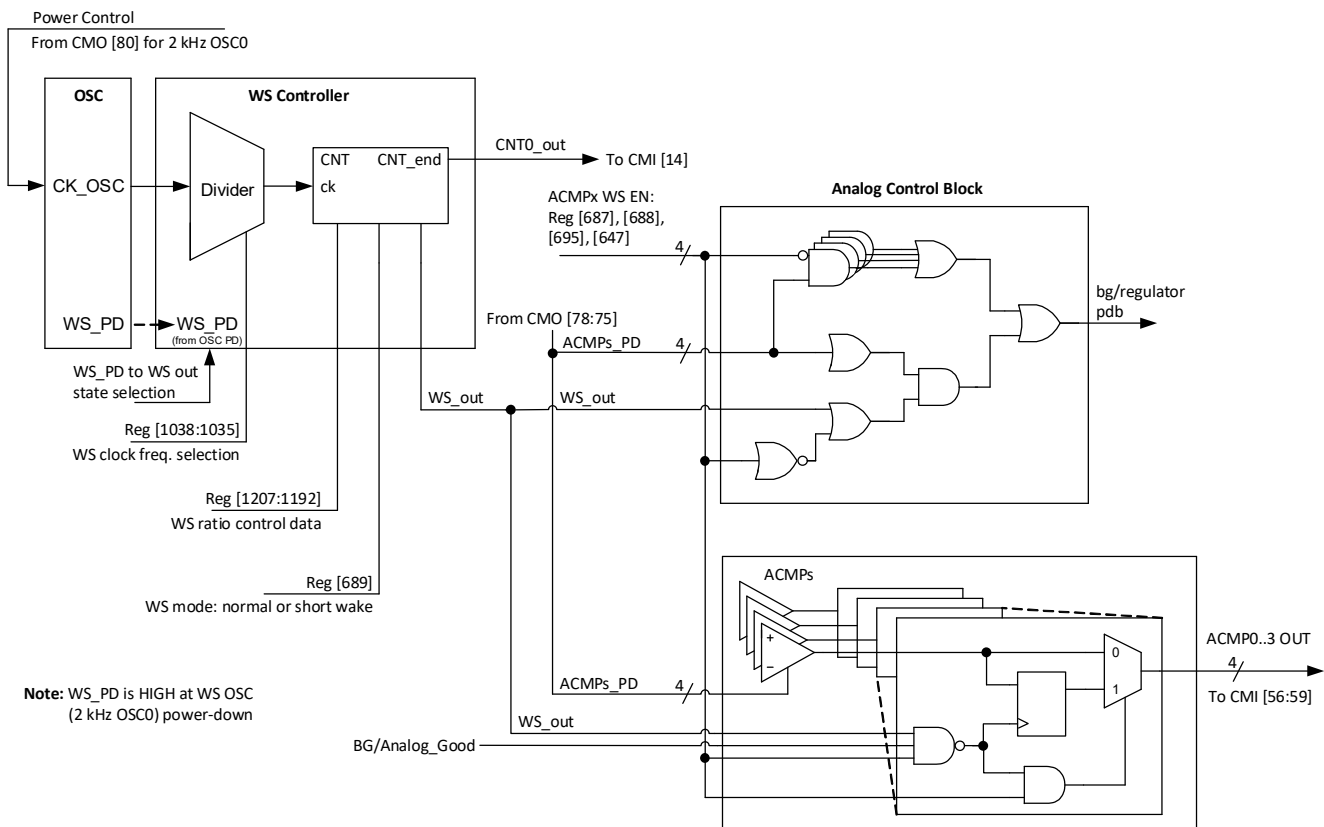
Figure 61. Wake/Sleep Controller
