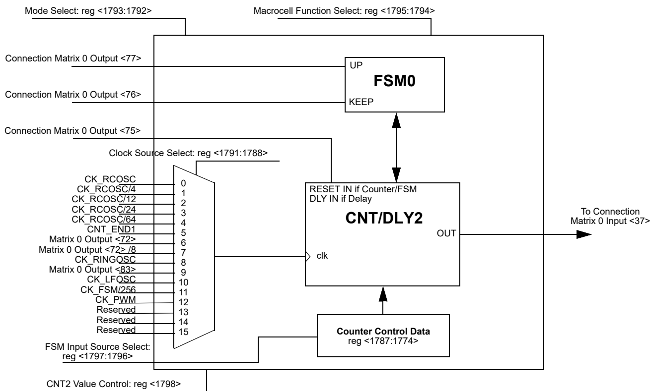
Figure 79. CNT/DLY2/FSM0
