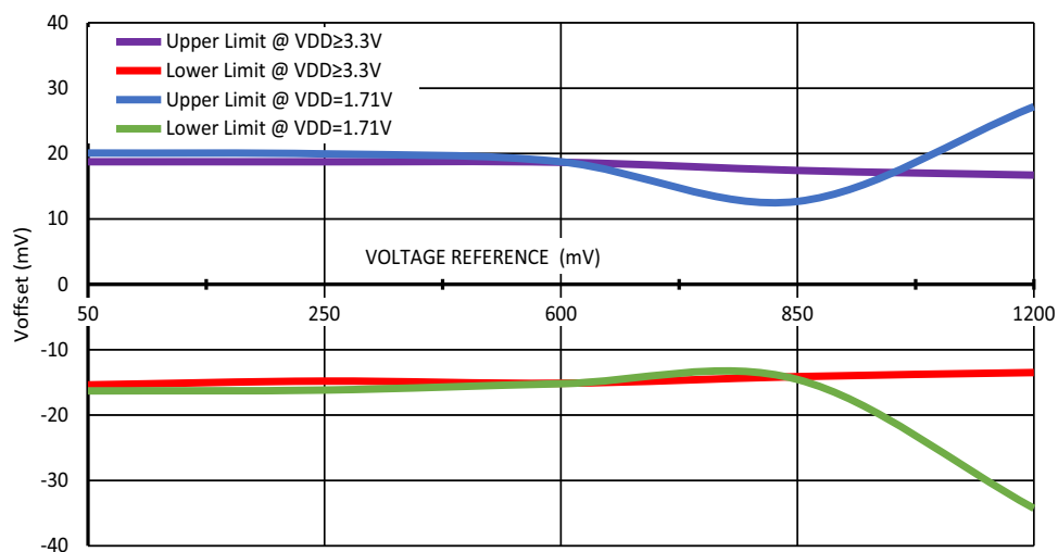
Figure 51. Buffer Input Voltage Offset vs. Voltage Reference at T = (-40.... +85)°C, Buffer Bandwidth = 5 kHz, Vhys = 0 mV, Gain = 1
