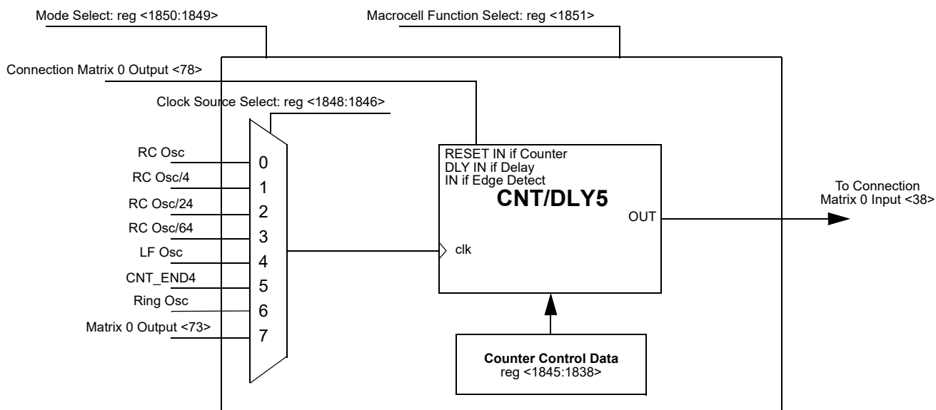
Figure 82. CNT/DLY5
