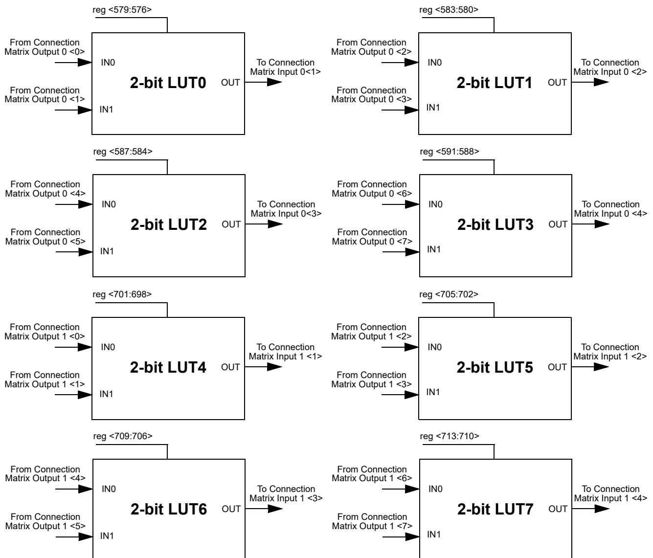
Figure 42. 2-bit LUTs
