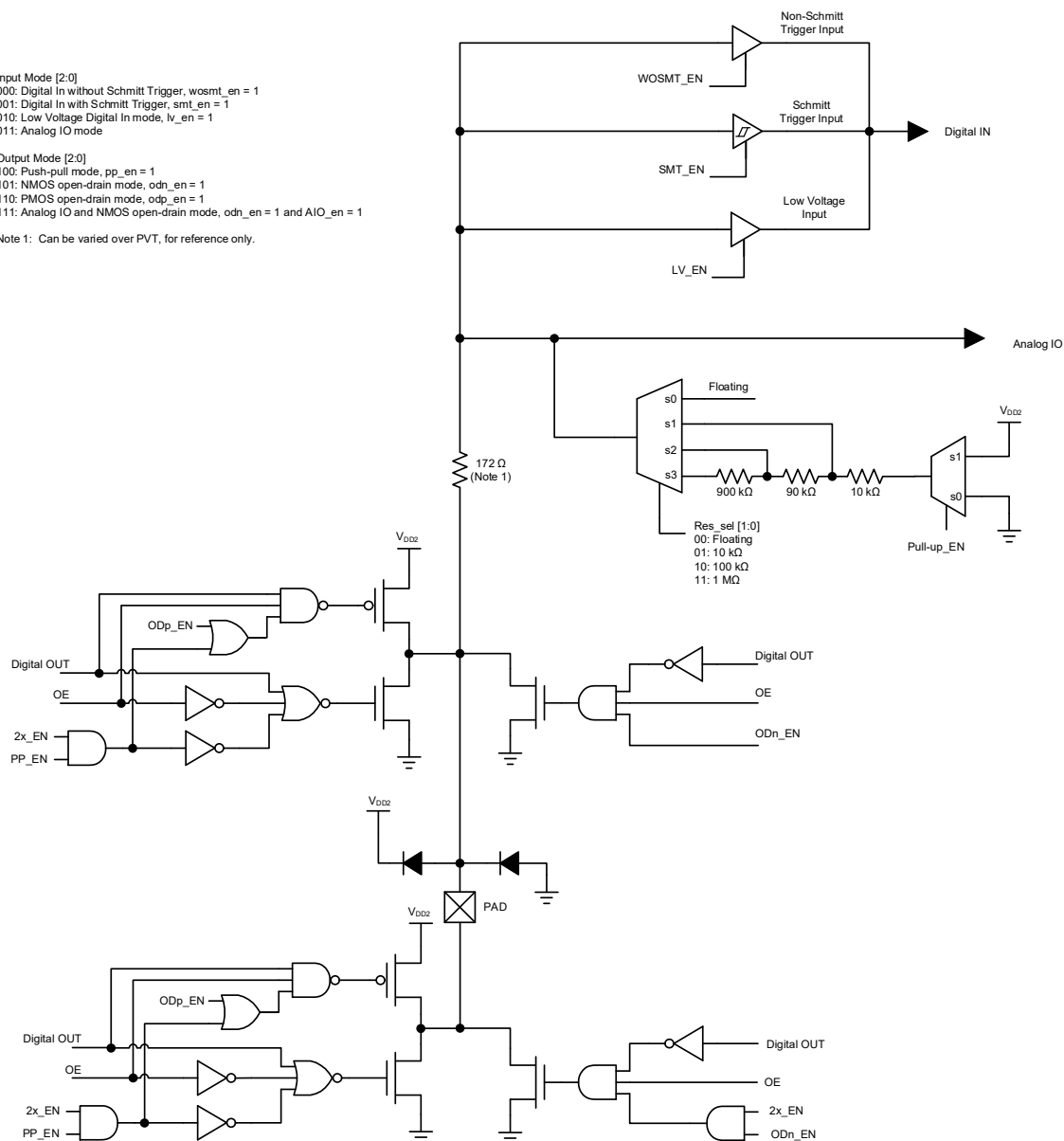
Figure 7. Register OE IO Structure Diagram
