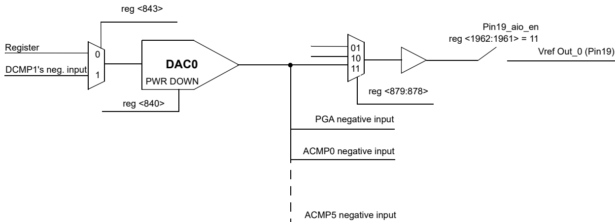
Figure 40. DAC0 Functional Diagram
