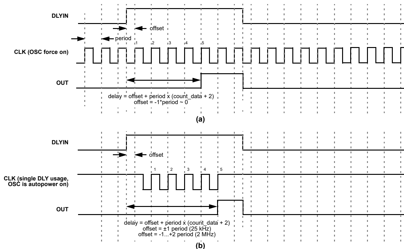
Figure 87. Timing (rising edge) for count data = 3: (a) oscillator is in Force Power On Mode or an external oscillator is used, (b) oscillator is in Auto Power On Mode
