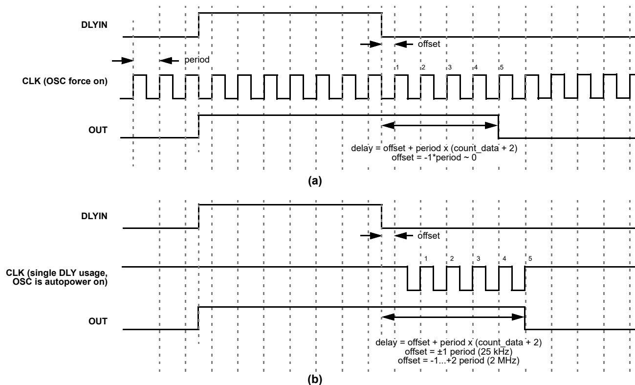
Figure 88. Timing (falling edge) for count data = 3: (a) oscillator is in Force Power On Mode or an external oscillator is used, (b) oscillator is in Auto Power On Mode
