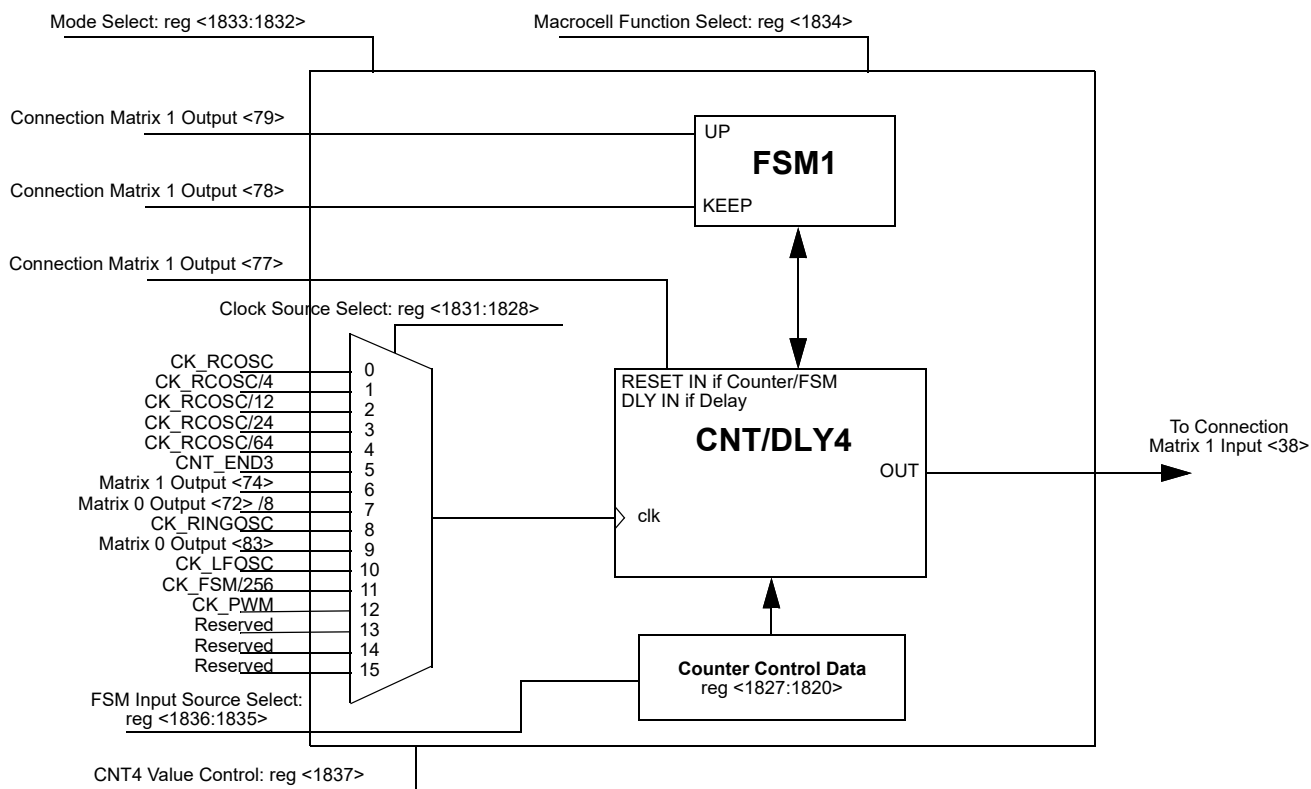
Figure 81. CNT/DLY4/FSM1
