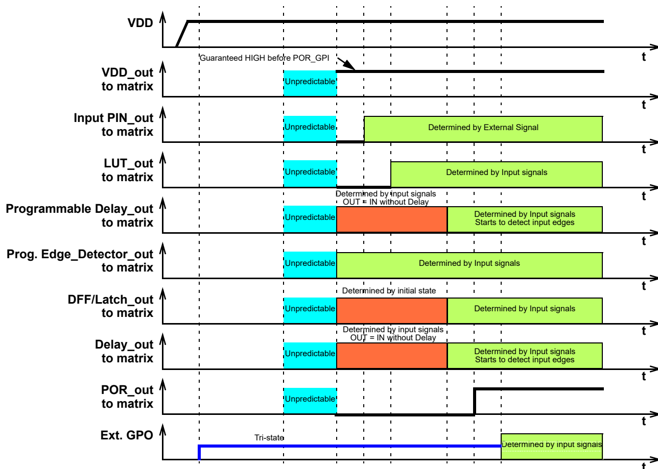
Figure 125. Internal Macrocell States during POR sequence
