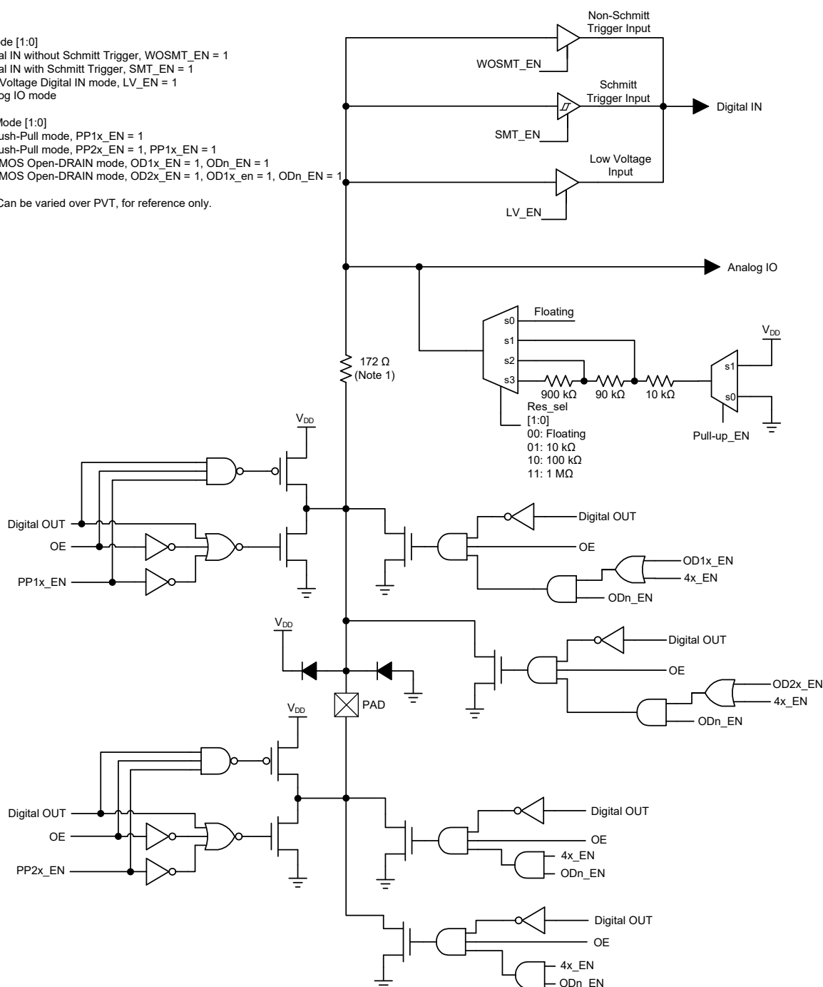
Figure 5. Matrix OE IO 4x Drive Structure Diagram
