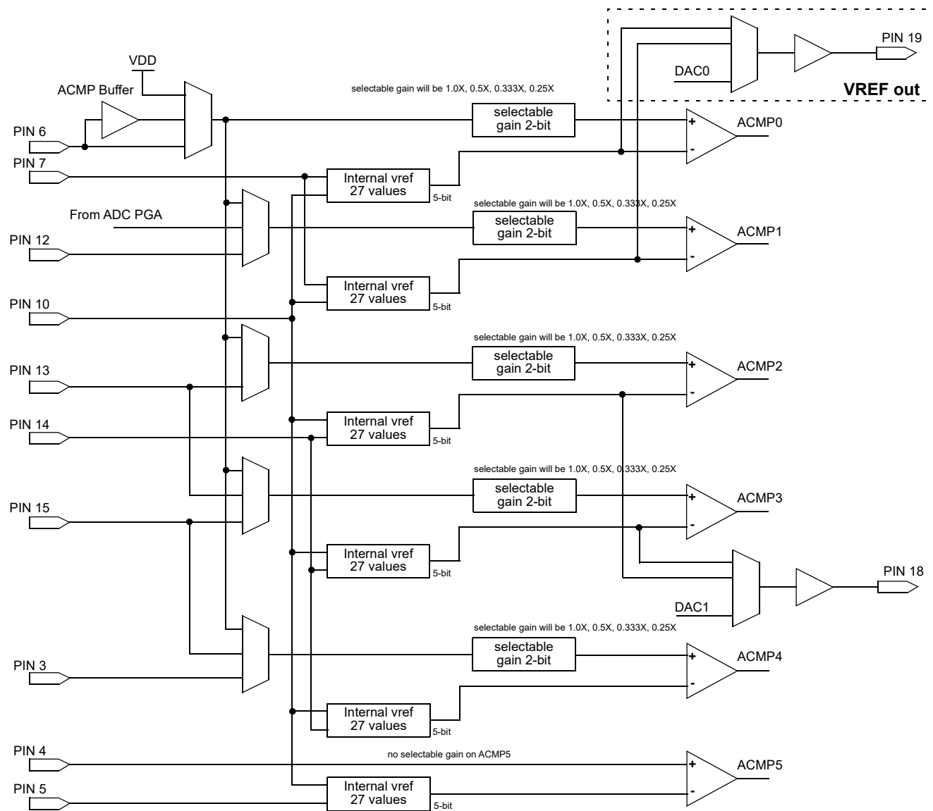
Figure 55. ACMP Master Architecture Diagram
