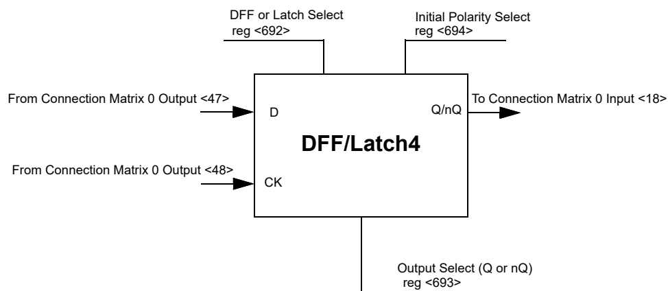
Figure 66. DFF/Latch4
