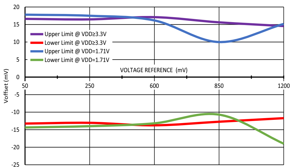
Figure 52. Buffer Input Voltage Offset vs. Voltage Reference at T = (-40.... +85)°C, Buffer Bandwidth = 20 kHz, Vhys = 0 mV, Gain = 1
