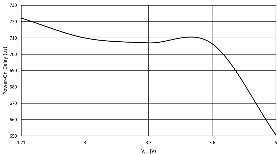
Figure 106. LF Oscillator Maximum Power-On Delay vs. V_{DD} at T = 25\text{ }^{\circ}\text{C} , OSC = 1.73 kHz
