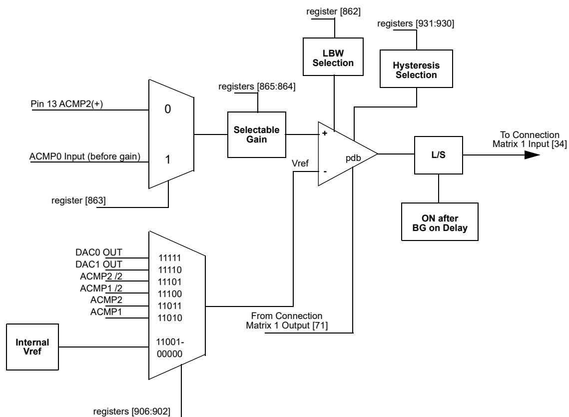
Figure 45. ACMP2 Block Diagram
