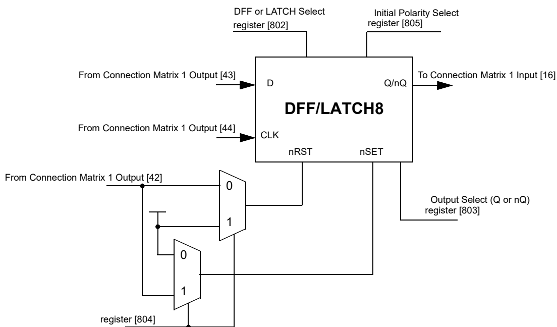
Figure 59. DFF/LATCH8
