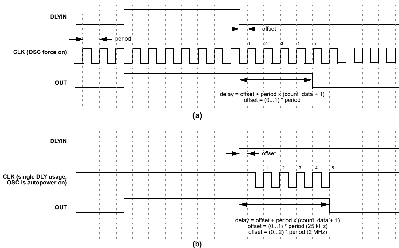
Figure 77. Timing (Falling Edge) for Count Data = 3: (a) Oscillator is in Force Power On Mode or an External Oscillator is Used, (b) Oscillator is in Auto Power On Mode
