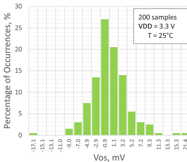
Figure 20. PGA Input Offset Distribution, Single-Ended Mode, G = 0.5
