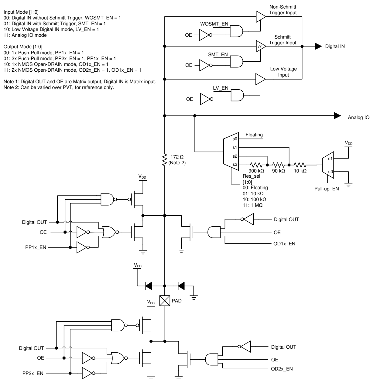
Figure 5. Matrix OE IO Structure Diagram
