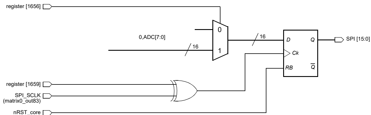
Figure 94. The SPI Used as ADC Data Buffer Diagram
