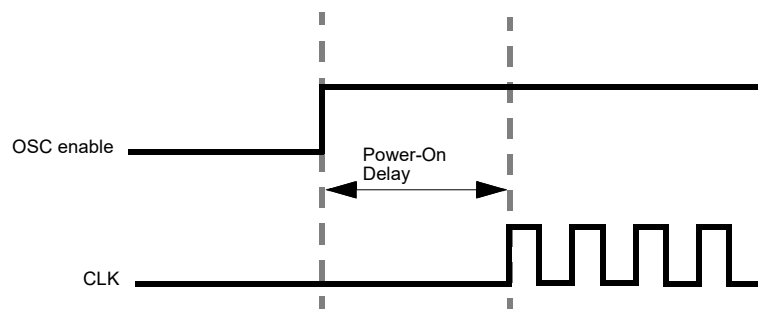
Figure 105. Oscillator Startup Diagram
