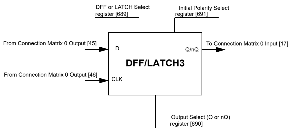
Figure 54. DFF/LATCH3
