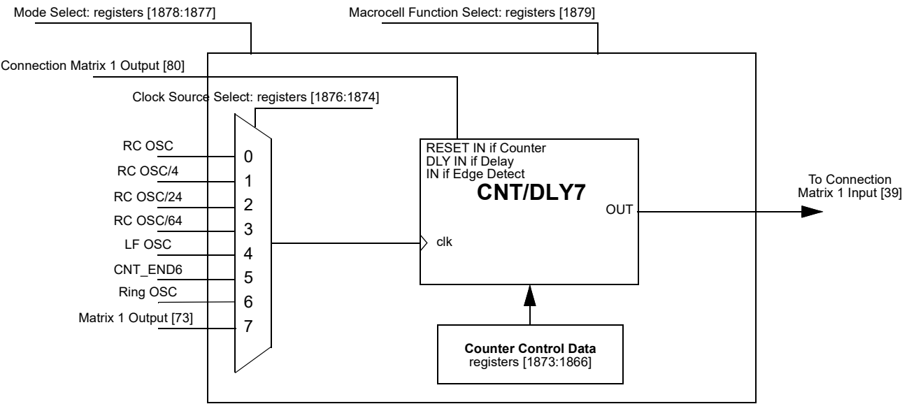
Figure 73. CNT/DLY7
