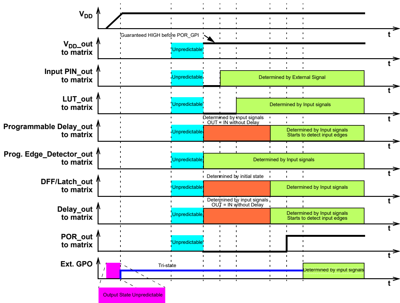
Figure 123. Internal Macrocell States during POR Sequence
