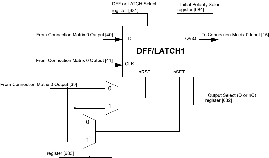
Figure 52. DFF/LATCH1
