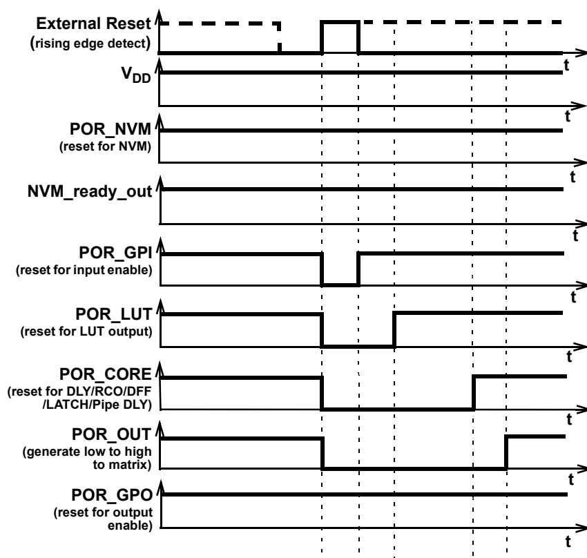
Figure 126. External Reset Sequence (Rising Edge Detect)
