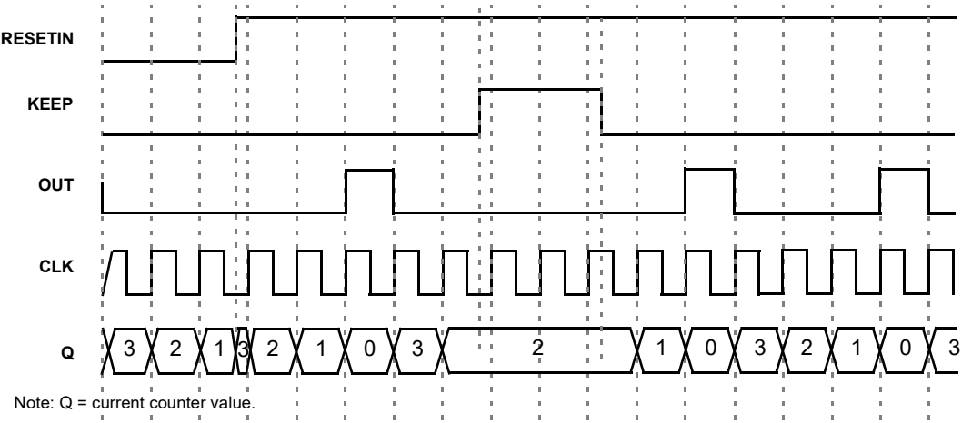
Figure 82. CNT/FSM Timing Diagram (Set Rising Edge Mode, Oscillator is Forced On, UP = 0) for Counter Data = 3
