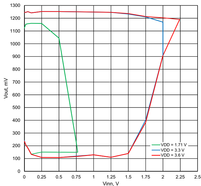
Figure 27. Typical Negative Input Voltage Range vs. Linear Output Voltage, Pseudo-Differential Mode, G = 2
