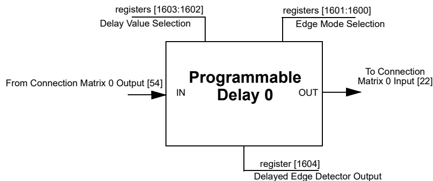
Figure 97. Programmable Delay
