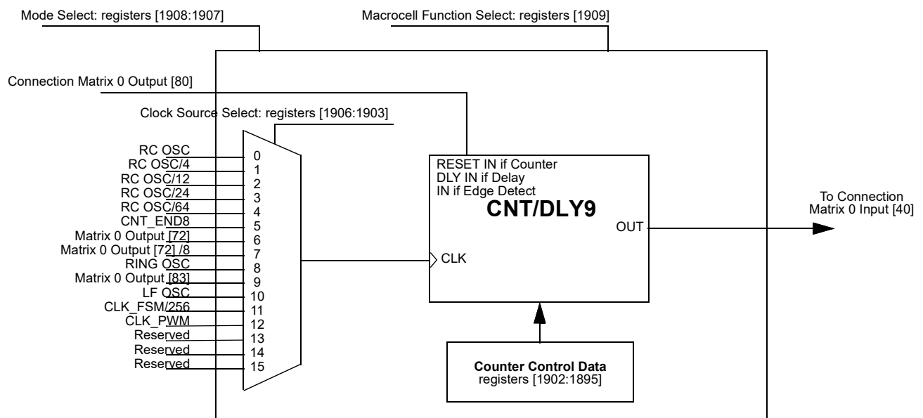
Figure 75. CNT/DLY9/PWM_RAMP
