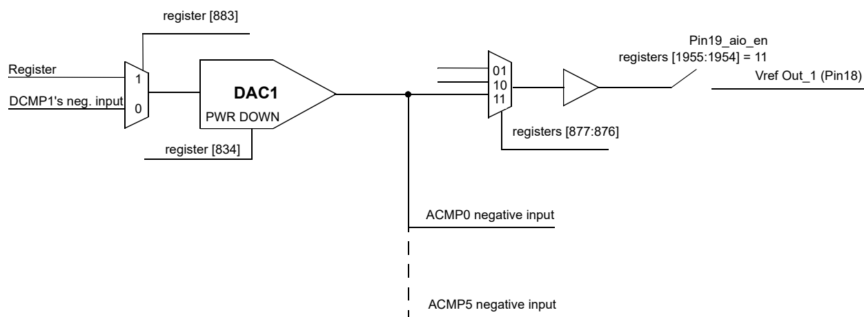
Figure 32. DAC1 Functional Diagram
