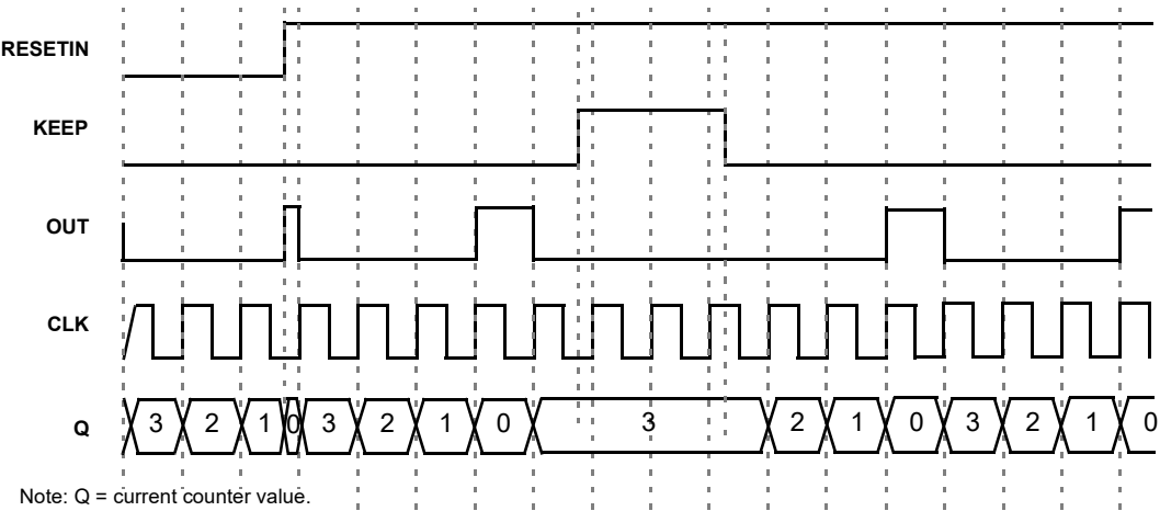
Figure 81. CNT/FSM Timing Diagram (Reset Rising Edge Mode, Oscillator is Forced On, UP = 0) for Counter Data = 3
