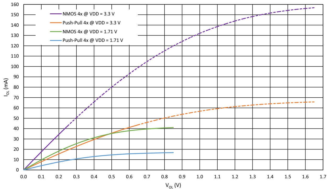
Figure 12. Typical Low Level Output Current vs. Low Level Output Voltage, 4x Drive at T = 25\text{ }^{\circ}\text{C}
