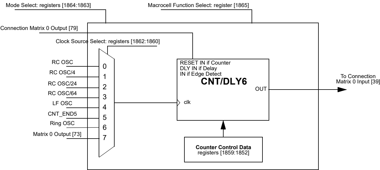
Figure 72. CNT/DLY6
