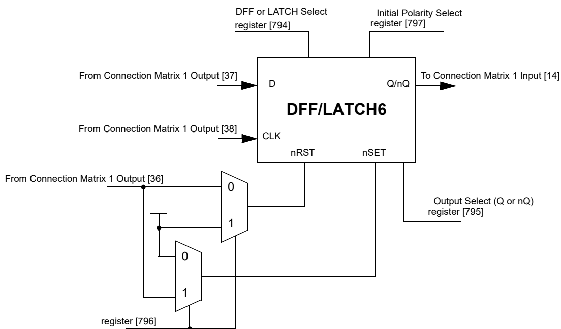
Figure 57. DFF/LATCH6
