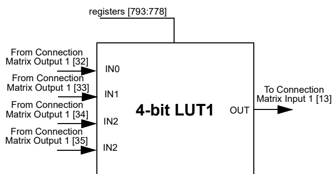
Figure 37. 4-bit LUT1
