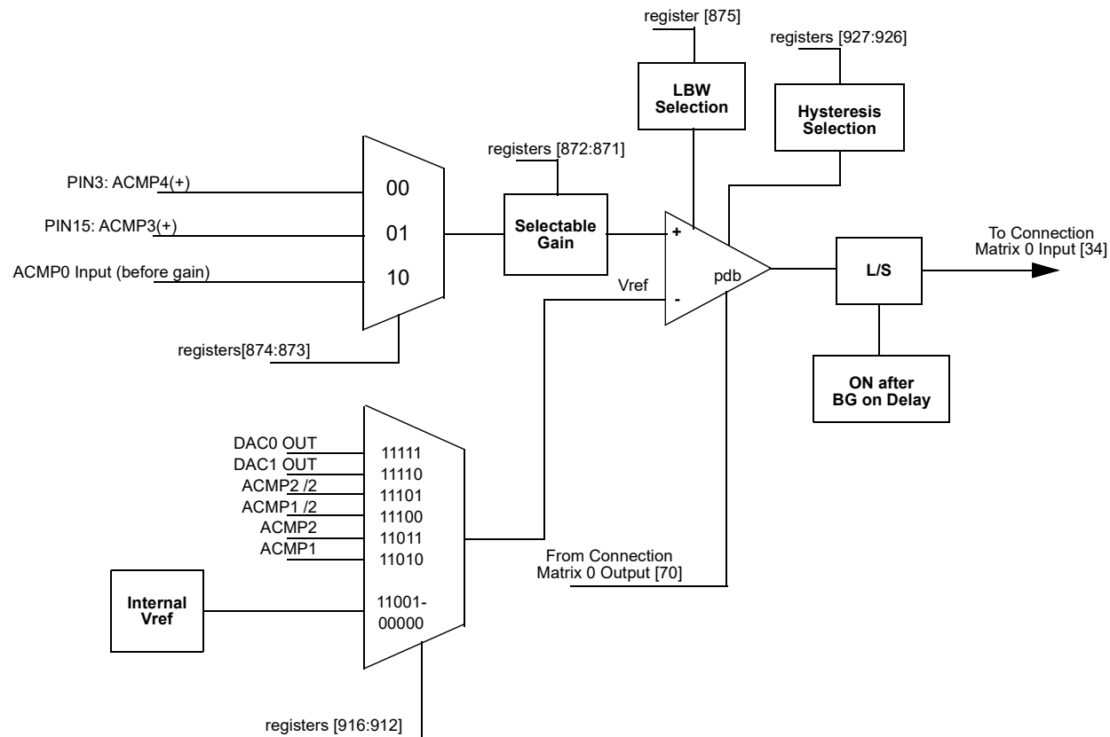
Figure 47. ACMP4 Block Diagram
