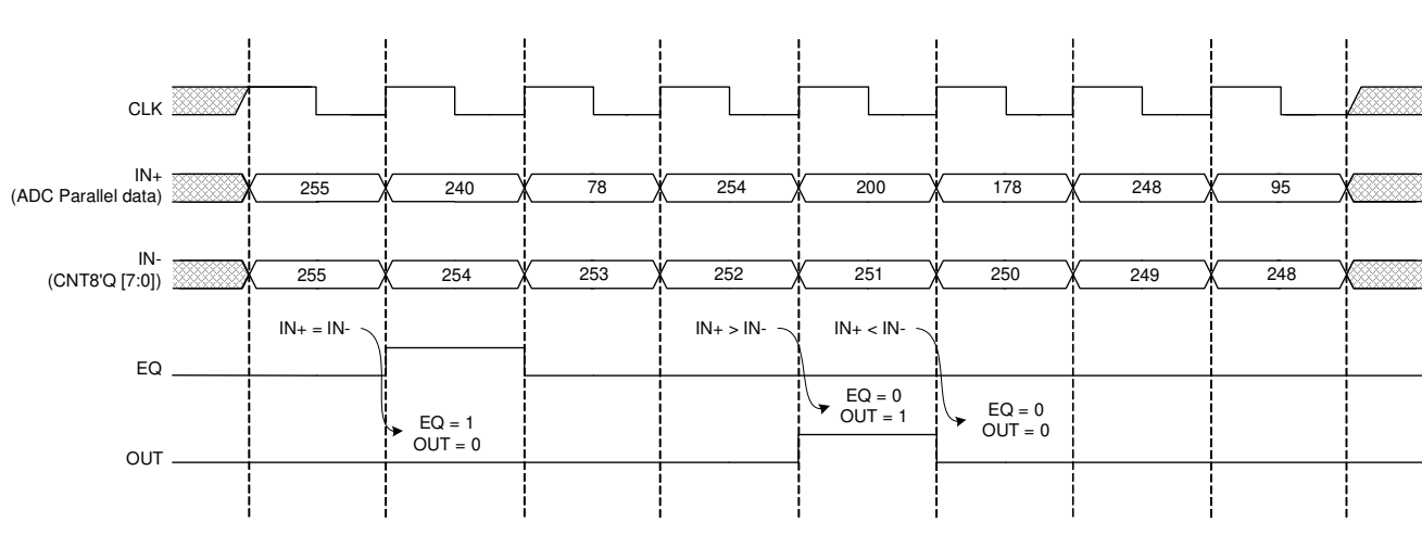
Figure 85. DCMP Timing Diagram
