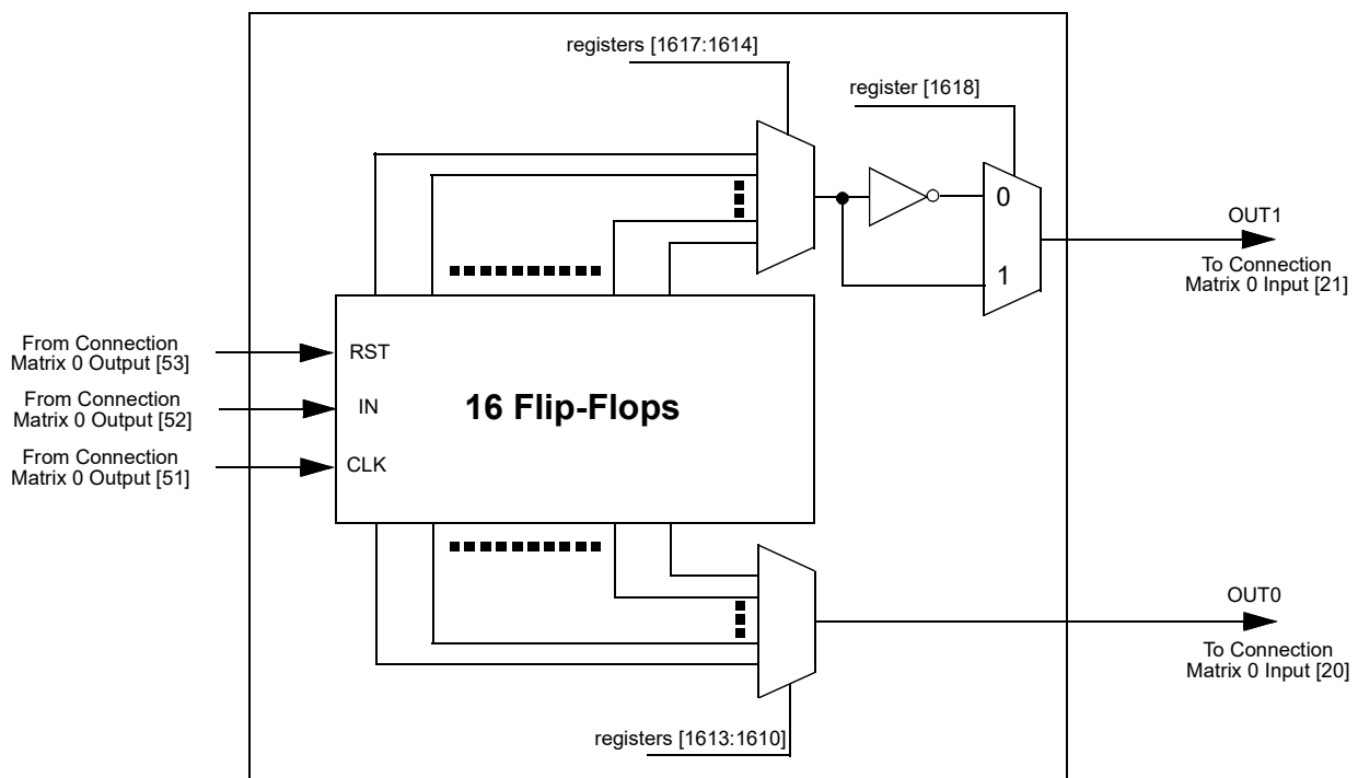
Figure 95. Pipe Delay 0
