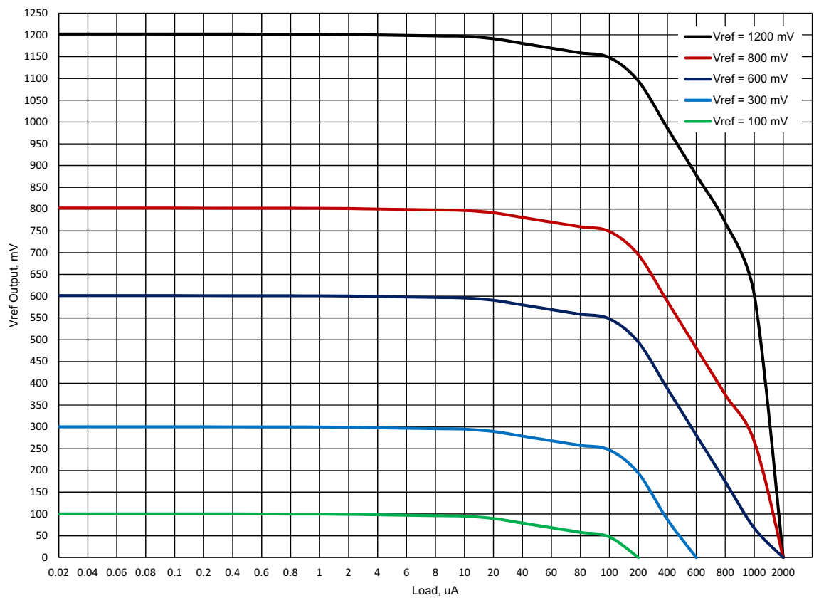
Figure 103. Typical Load Regulation, T = 25 °C, VDD = 3.3 V
