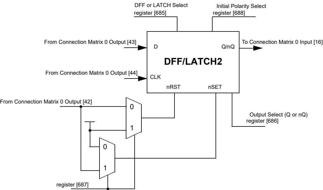
Figure 53. DFF/LATCH2
