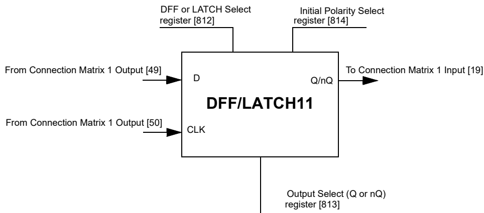
Figure 62. DFF/LATCH11
