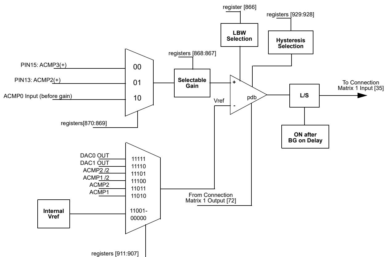
Figure 46. ACMP3 Block Diagram
