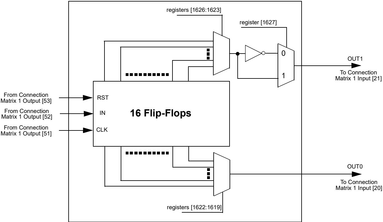
Figure 96. Pipe Delay 1
