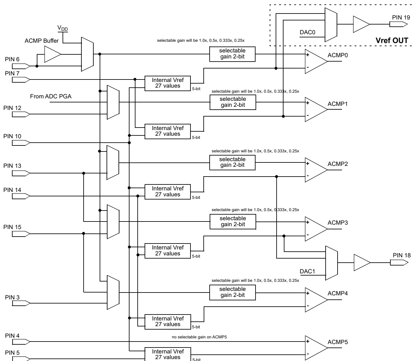
Figure 42. ACMP Master Architecture Diagram
