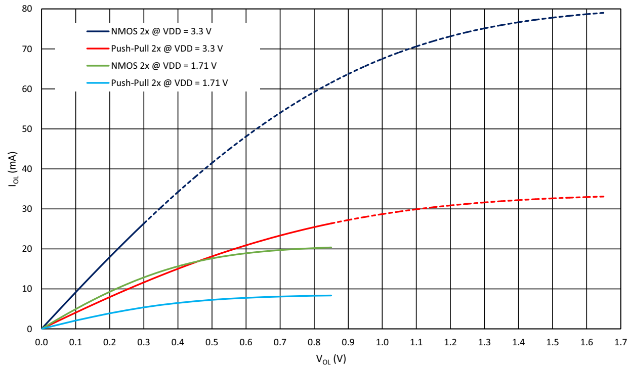
Figure 11. Typical Low Level Output Current vs. Low Level Output Voltage, 2x Drive at T = 25\text{ }^{\circ}\text{C}
