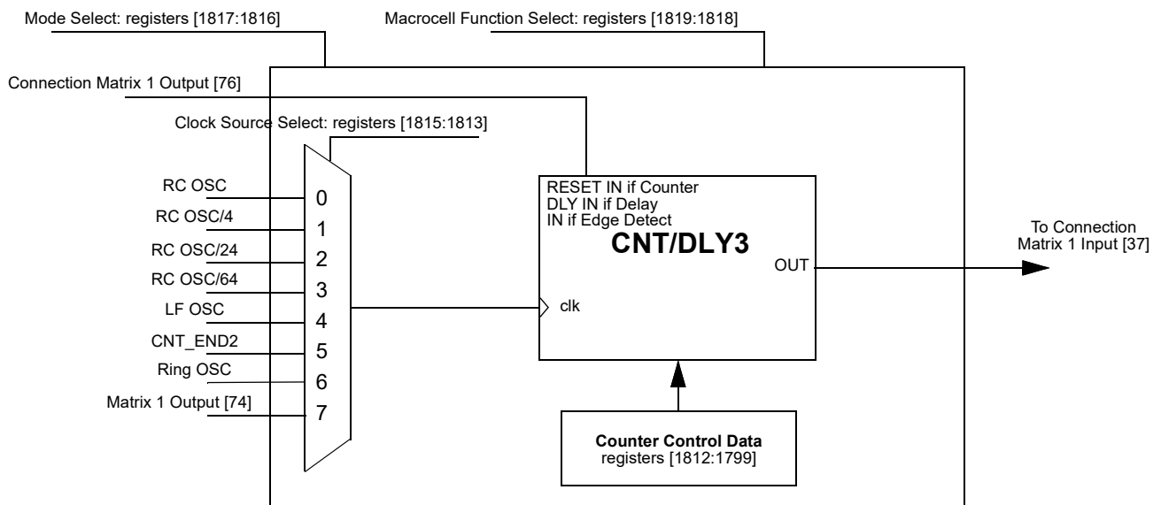
Figure 69. CNT/DLY3
