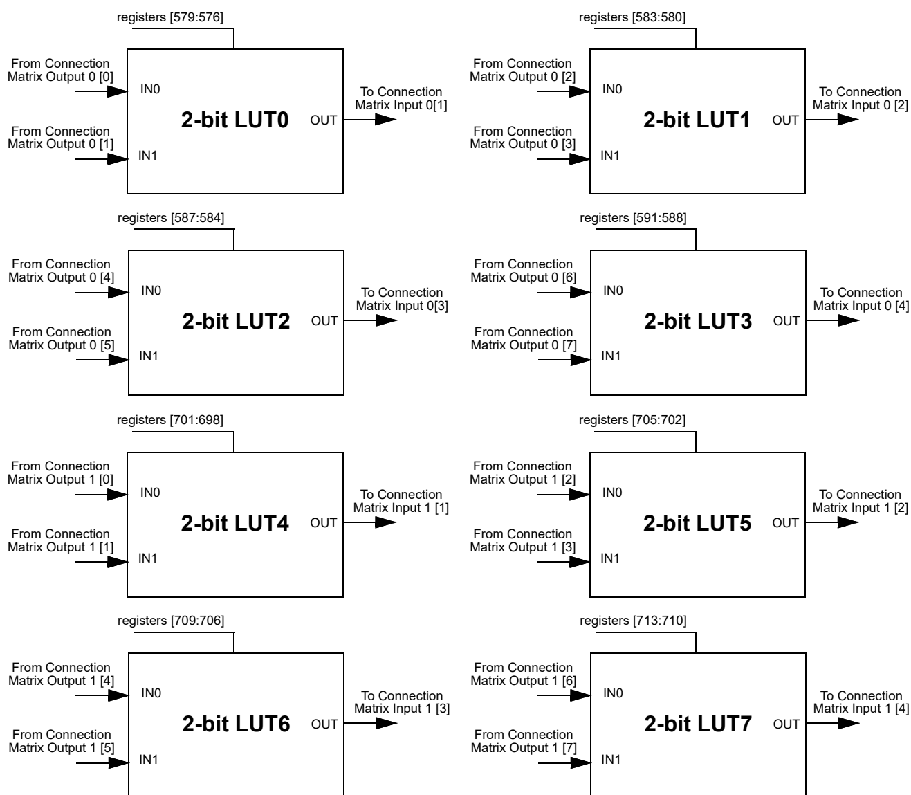
Figure 34. 2-bit LUTs
