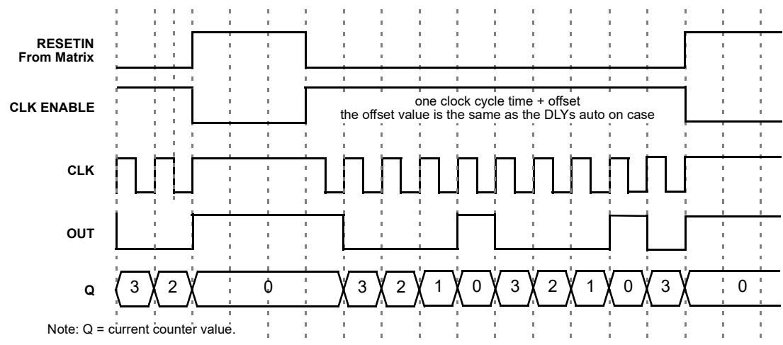
Figure 80. Timing (Reset High Level Mode, Oscillator is Autopowered On (Controlled by Reset)) for Count Data = 3
