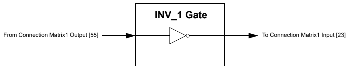
Figure 129. INV_1 Gate
