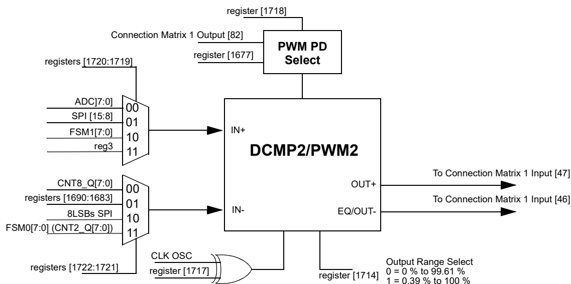
Figure 88. DCMP2/PWM2 Functional Diagram
