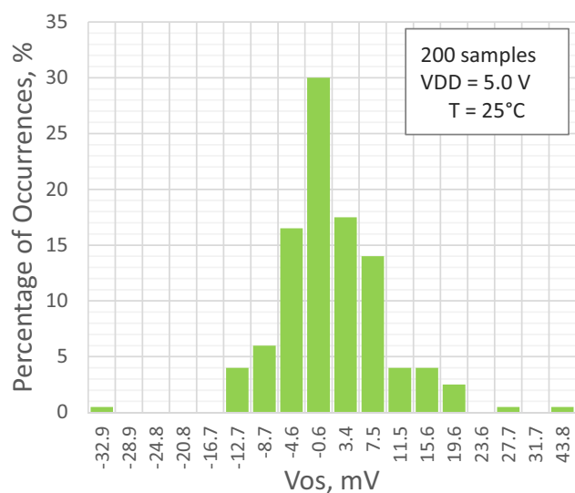
Figure 19. PGA Input Offset Distribution, Single-Ended Mode, G = 0.25
