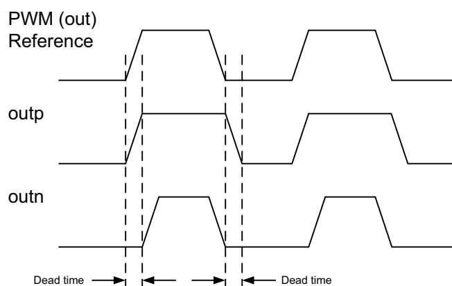
Figure 89. PWM Dead Band Control Timing Diagram
