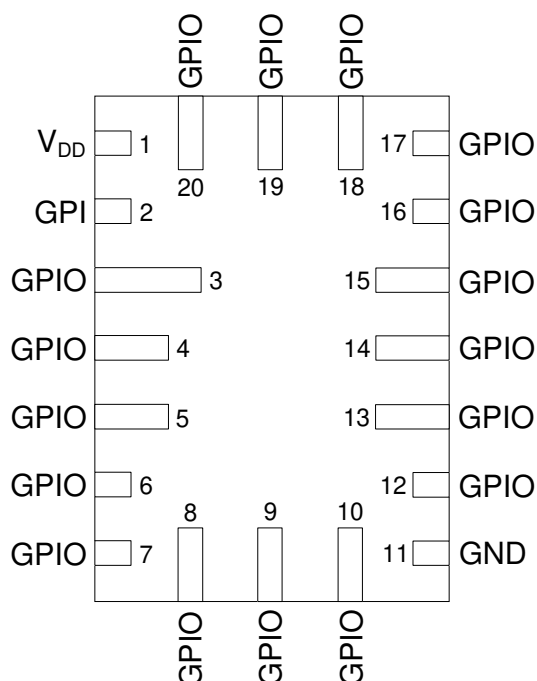
Figure 2. Pin Assignments - STQFN-20 (Top View)
