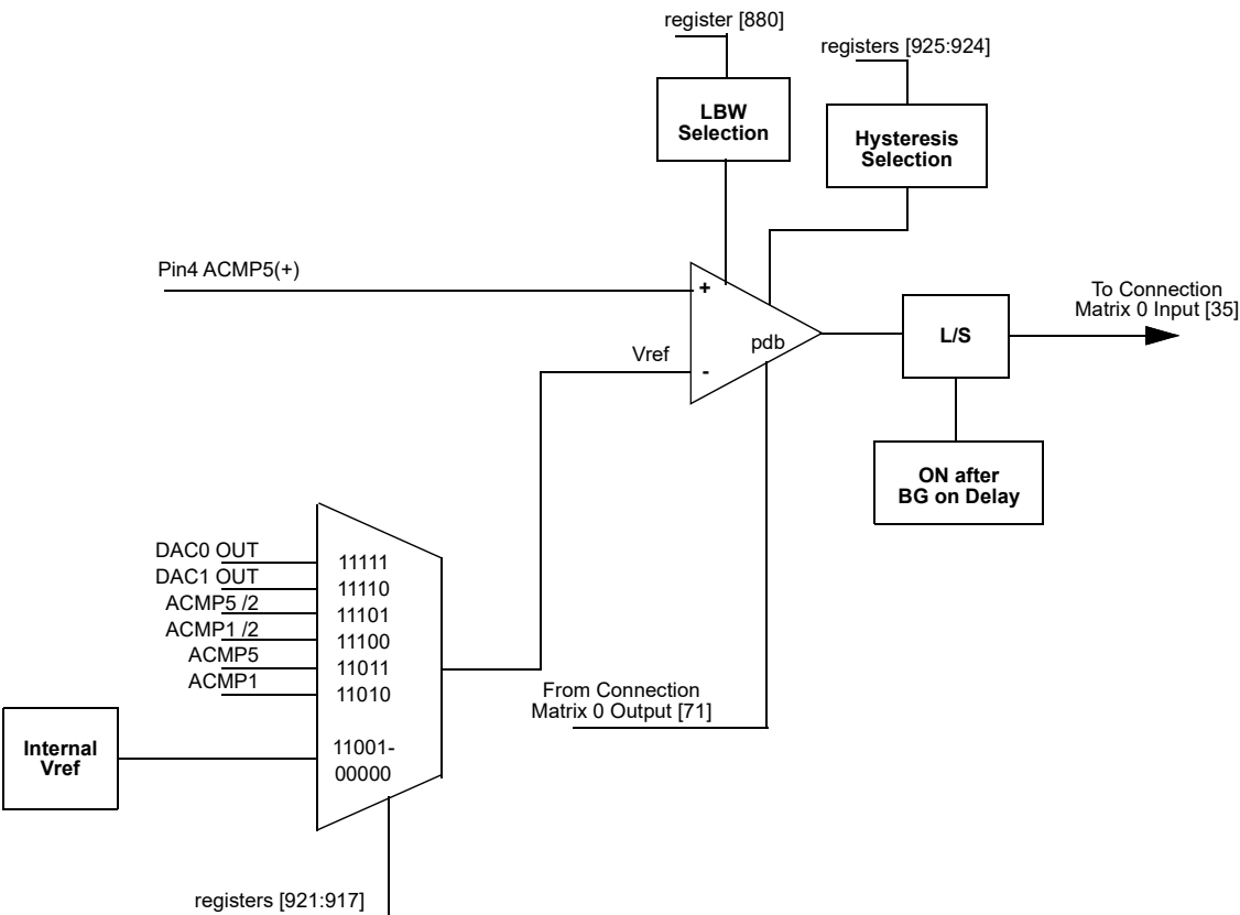
Figure 48. ACMP5 Block Diagram
