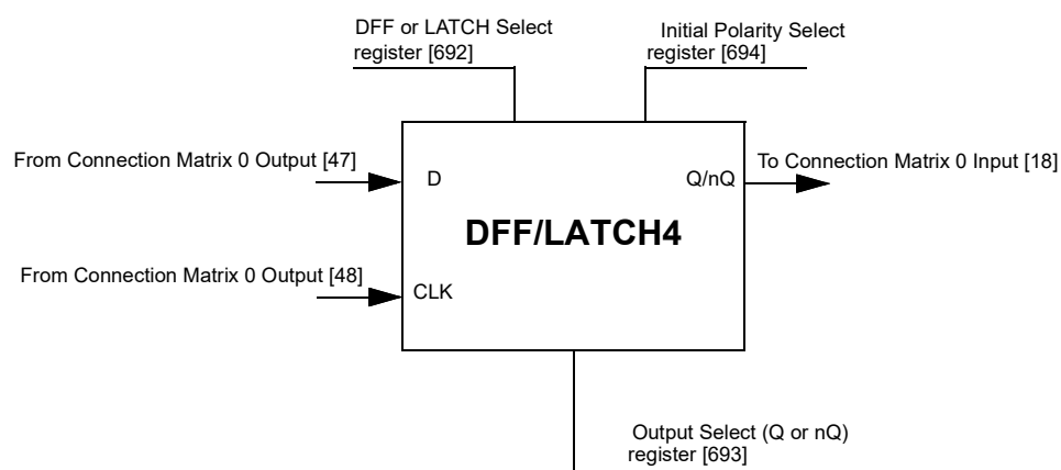
Figure 55. DFF/LATCH4
