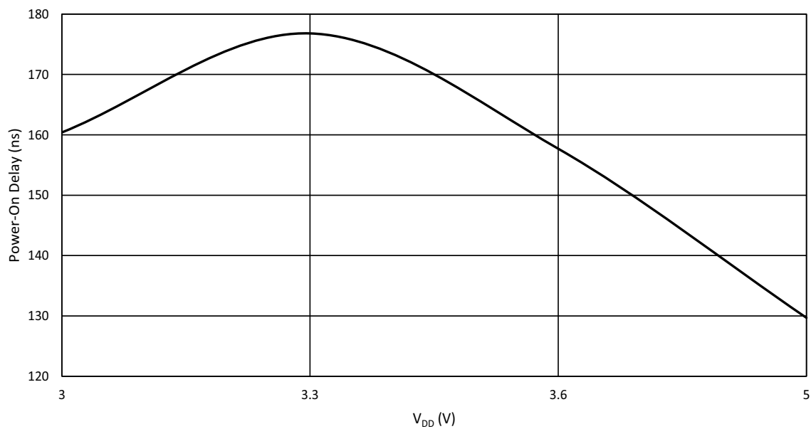
Figure 109. Ring Oscillator Maximum Power-On Delay vs. V_{DD} at T = 25\text{ }^{\circ}\text{C} , \text{OSC} = 27\text{ MHz}
