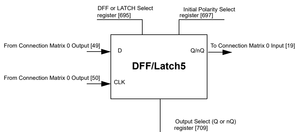
Figure 56. DFF/LATCH5
