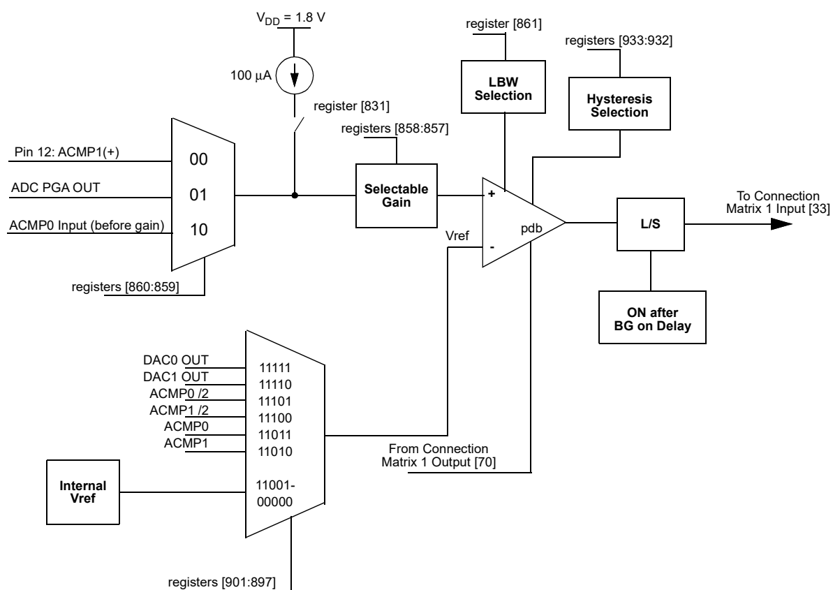
Figure 44. ACMP1 Block Diagram
