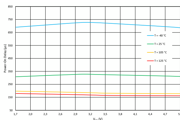
Figure 41. Maximum Power-On Delay vs. V_{DD} , BG = 100 \mu s, Regulator and Charge Pump Set to Automatic ON/OFF
