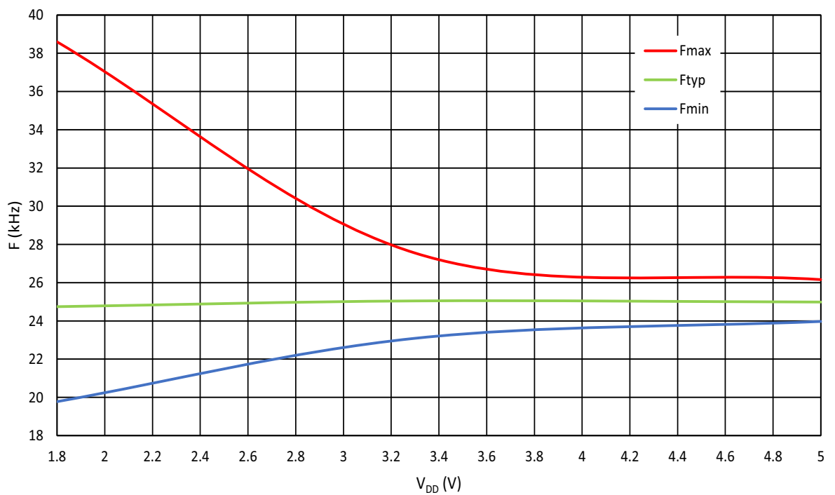
Figure 115. RC Oscillator Frequency vs. V DD , RC OSC = 25 kHz, T = -40 °C to 105 °C
