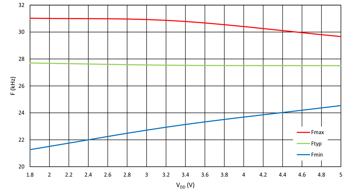
Figure 116. Ring Oscillator Frequency vs. V DD , OSC = 27 MHz, T = 25 °C
