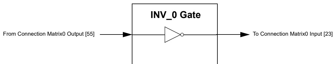
Figure 128. INV_0 Gate
