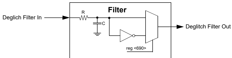
Figure 23. Deglitch Filter
