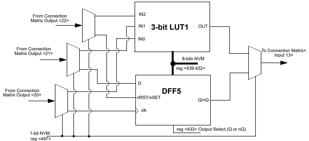
Figure 14. 3-bit LUT1 or DFF5
