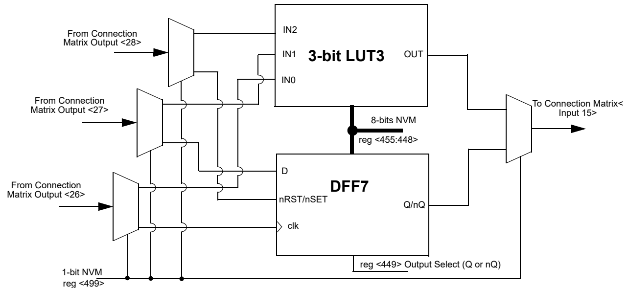
Figure 16. 3-bit LUT3 or DFF7
