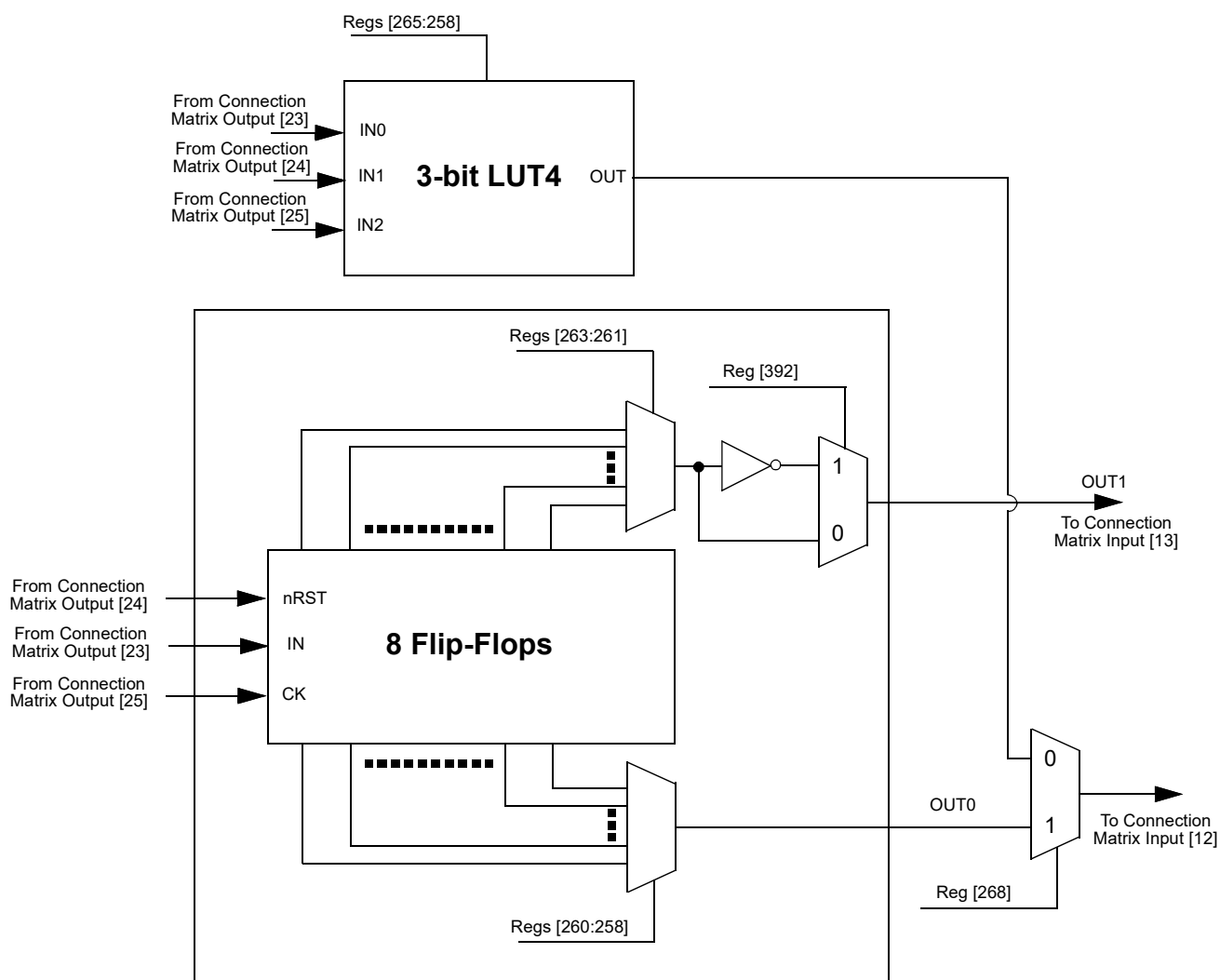
Figure 15. 3-bit LUT4 or Pipe Delay
