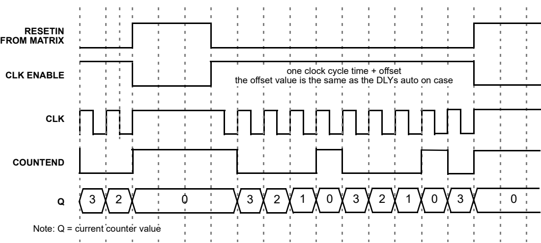
Figure 19. Timing (Reset High Level Mode, Oscillator is Auto Powered On (Controlled by Reset)) for Count Data = 3
