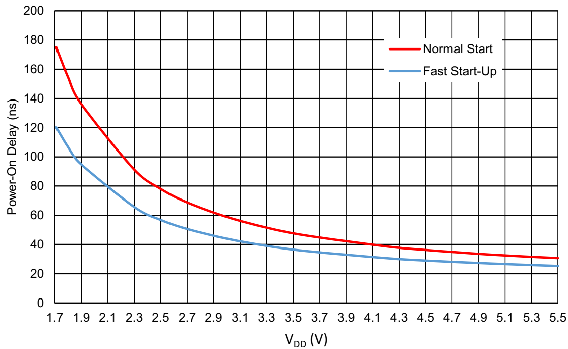
Figure 33. Oscillator Maximum Power-On Delay vs. V_{DD} at T_A = 25\text{ }^{\circ}\text{C} , OSC = 2 MHz
