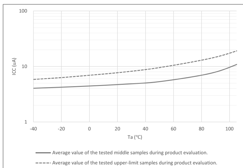
Figure 2.5 Temperature dependency in Deep Software Standby mode, power not supplied to SRAM or USB resume detecting unit, power-on reset circuit low-power function enabled (reference data)
