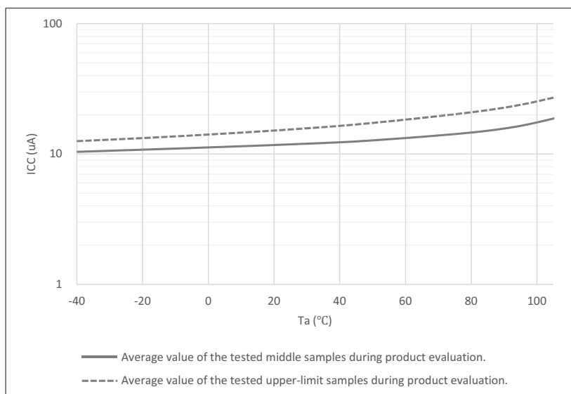
Figure 2.4 Temperature dependency in Deep Software Standby mode, power not supplied to SRAM or USB resume detecting unit, power-on reset circuit low-power function disabled (reference data)
