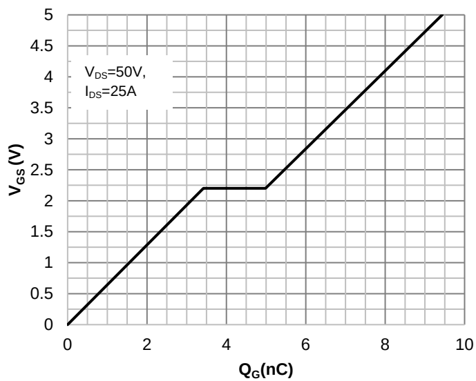
Figure 10. Gate Charge
