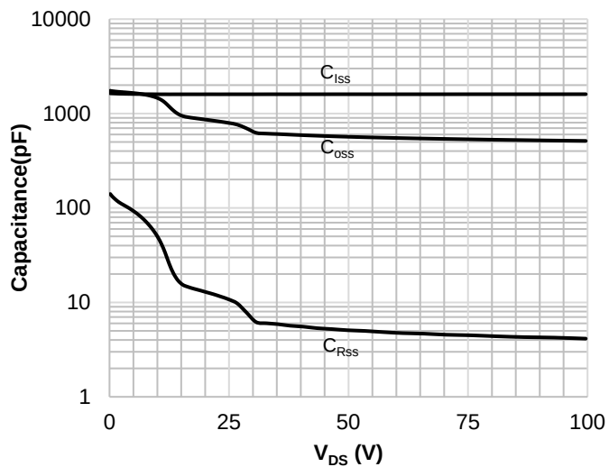
Figure 6. Typical Capacitance Characteristics
