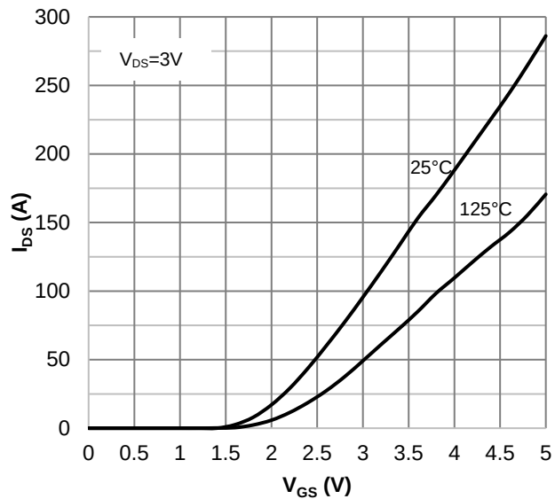
Figure 3. Typical Transfer Characteristics, Parameter T_J
