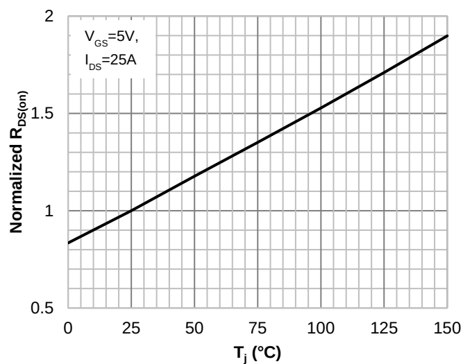
Figure 7. Normalized R_{DS(on)} , Parameter T_J
