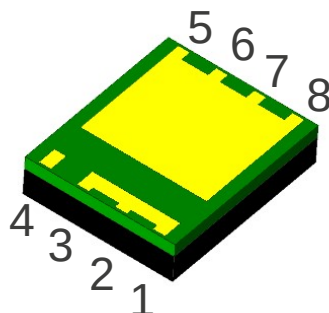
Figure 1. Pin Assignments – Bottom View
