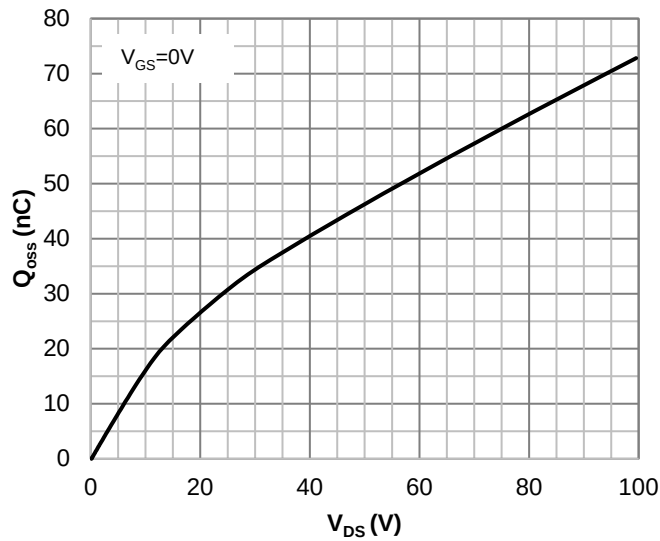
Figure 9. Typical Q_{oss}
