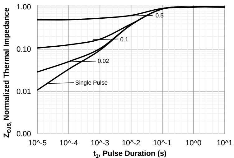
Figure 12. Junction-Board Transient Thermal Response, Parameter D = t_1/T
