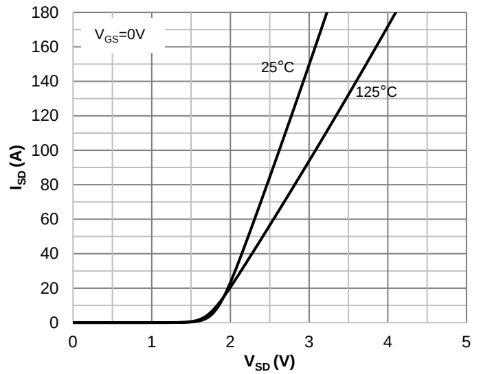
Figure 11. Reverse Conduction Characteristics, Parameter T_J
