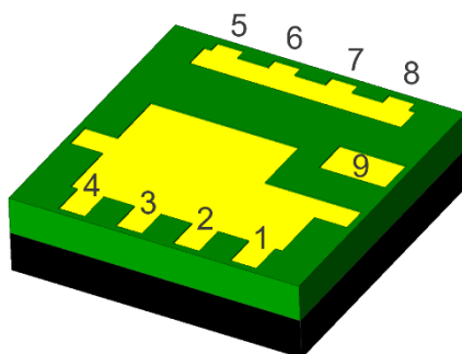
Figure 1. Pin Assignments – Bottom View
