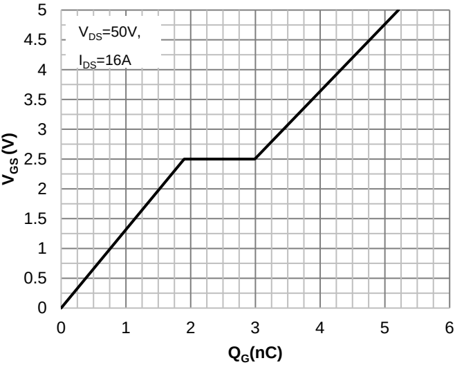
Figure 10. Gate Charge
