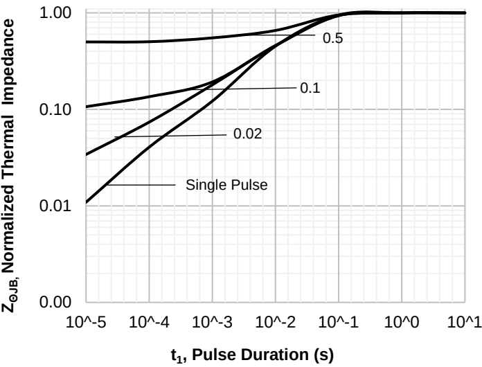
Figure 12. Junction-Board Transient Thermal Response, Parameter D=t_i/T
