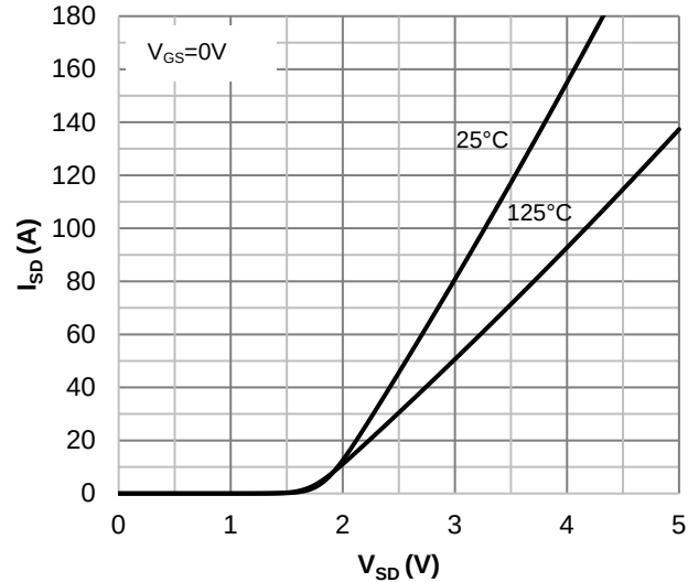
Figure 11. Reverse Conduction Characteristics, Parameter T_J
