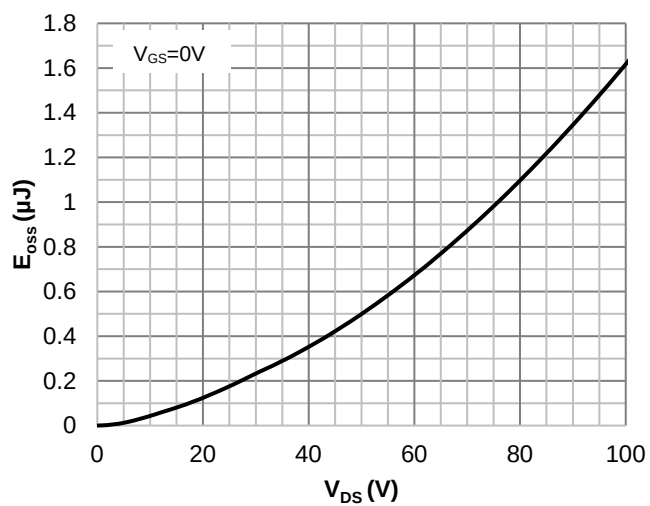
Figure 8. Typical C_{oss} Stored Energy
