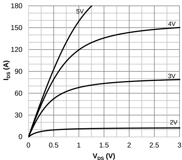
Figure 2. Typical Output Characteristics, Parameter V_{GS}
