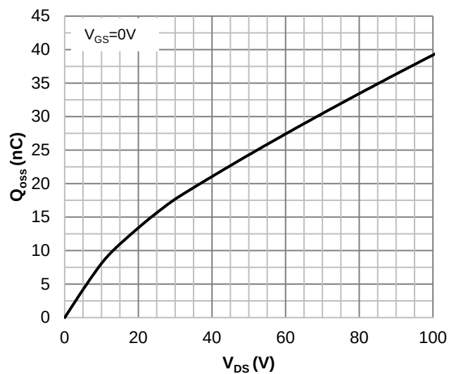
Figure 9. Typical Q_{oss}
