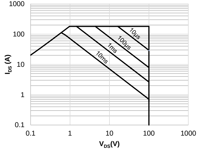
Figure 13. Safe Operating Area (Single Pulse), Parameter T_J = \text{Max Rated}
