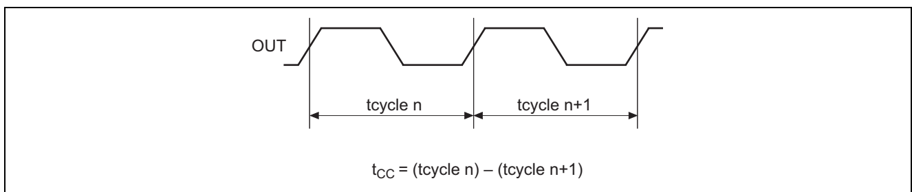
図 1 Cycle to cycle jitter
