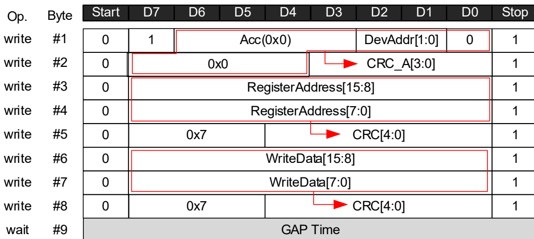
Figure 30. UART register write mode
