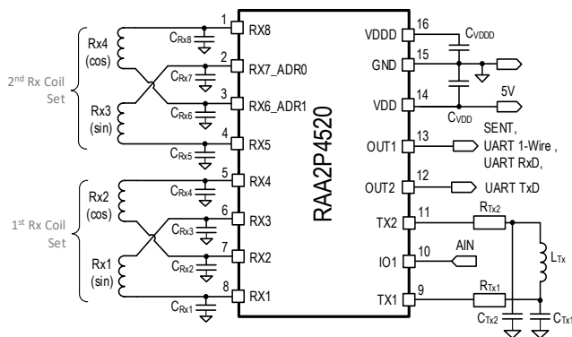
Figure 1. Application circuit example
