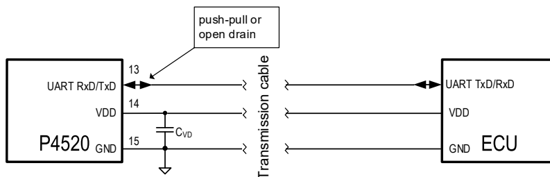
Figure 23. UART 1-wire point-to-point single wire bi-directional connection
