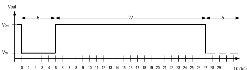
Figure 18. SENT nibble output for value = 15 DEC
