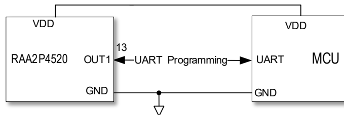
Figure 35. UART single wire NVM programming
