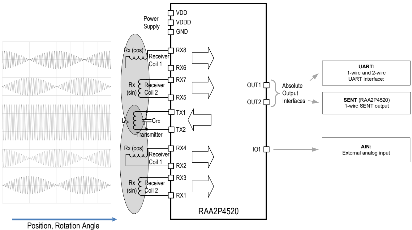
Figure 3. Input and output signals of RAA2P4520
