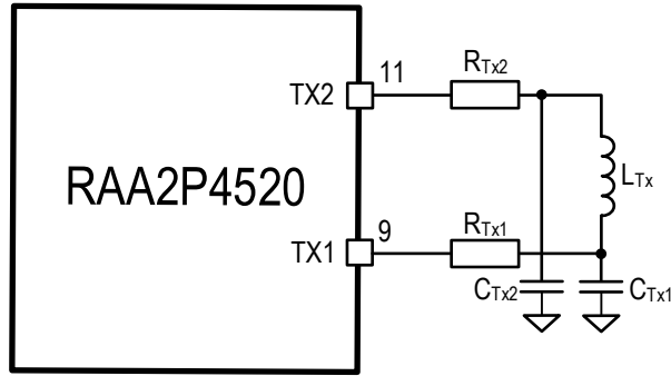
Figure 5. LC oscillator connection with split TX capacitors
