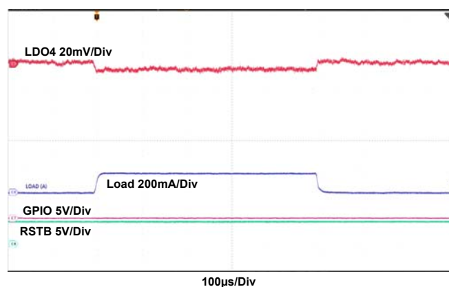
Figure 18. V_{OUT4} Load Transient, 0A to 0.375A
