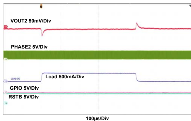
Figure 16. V_{OUT2} Load Transient, 0A to 0.375A
