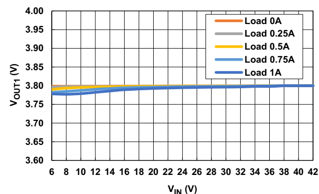
Figure 13. V_{OUT1} = 3.8V , Line Regulation
