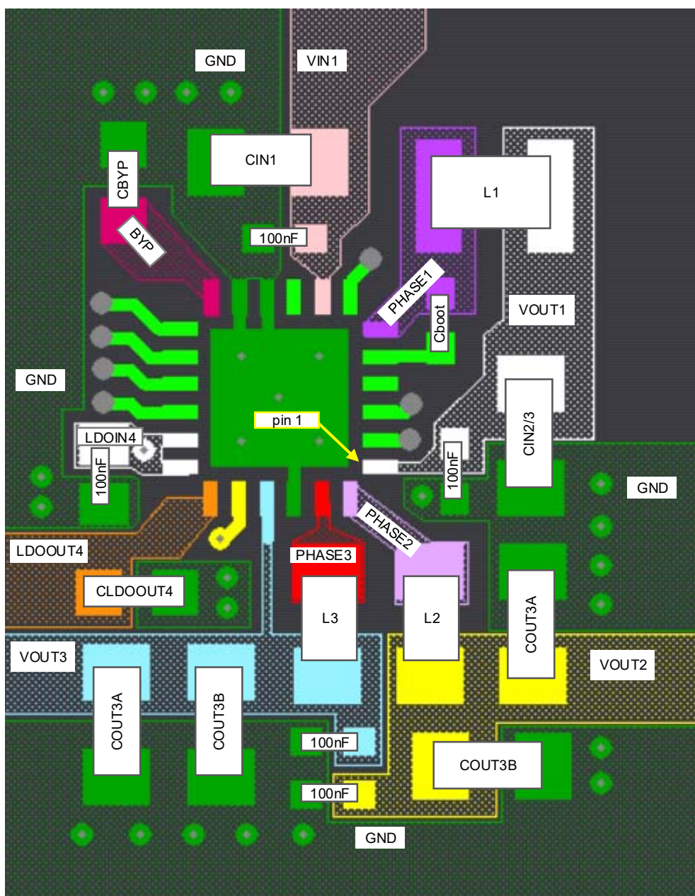
Figure 31. PCB Layout
