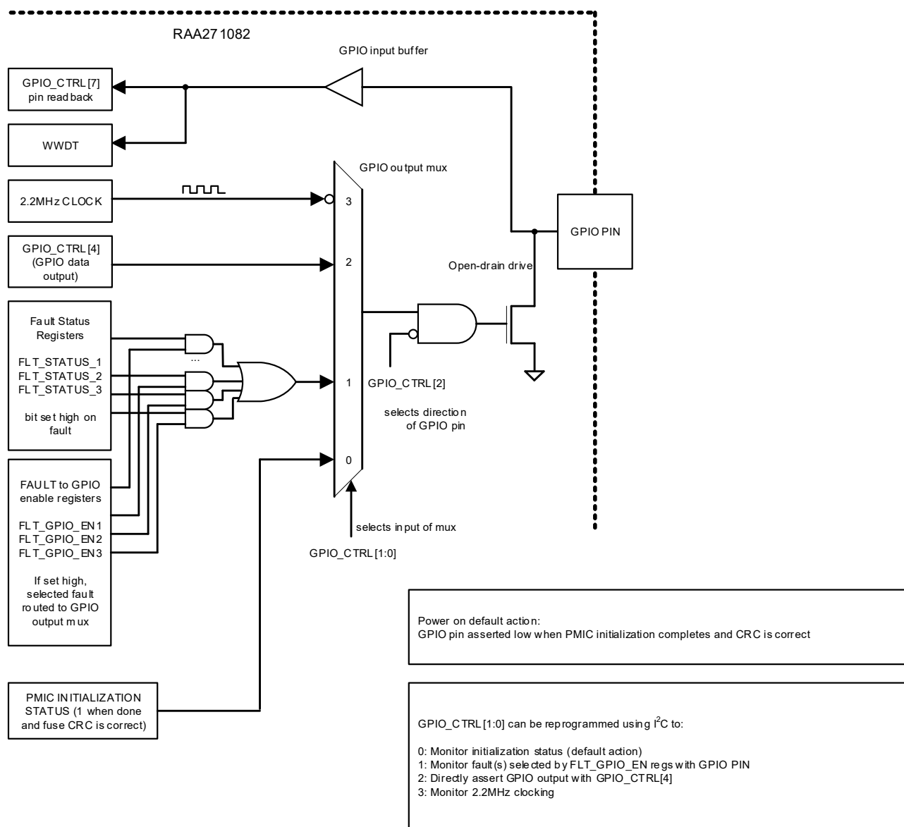
Figure 28. GPIO Block Diagram
