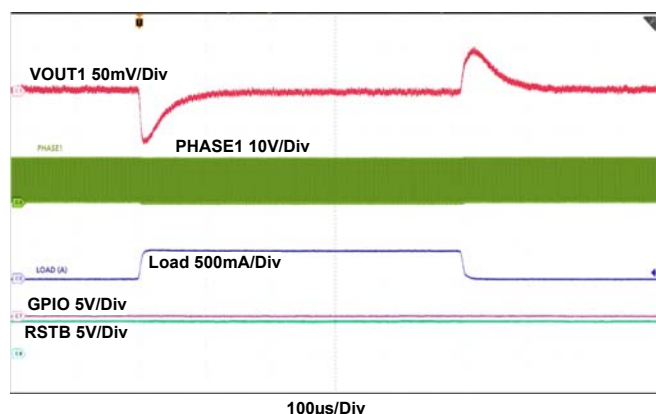
Figure 15. V_{OUT1} Load Transient, 0A to 0.375A
