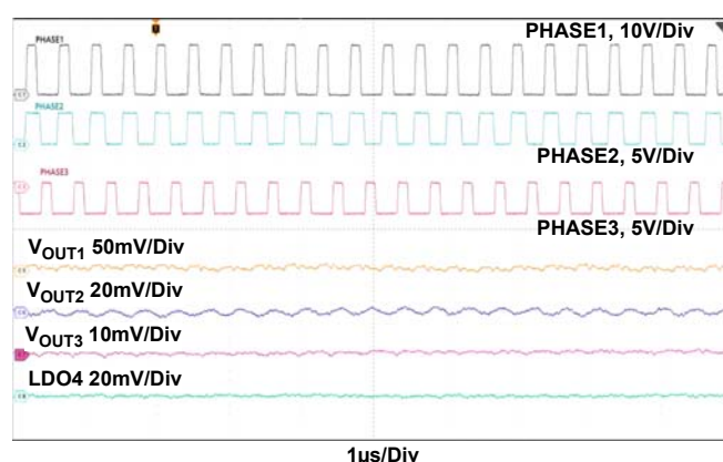
Figure 20. Switching Operation
