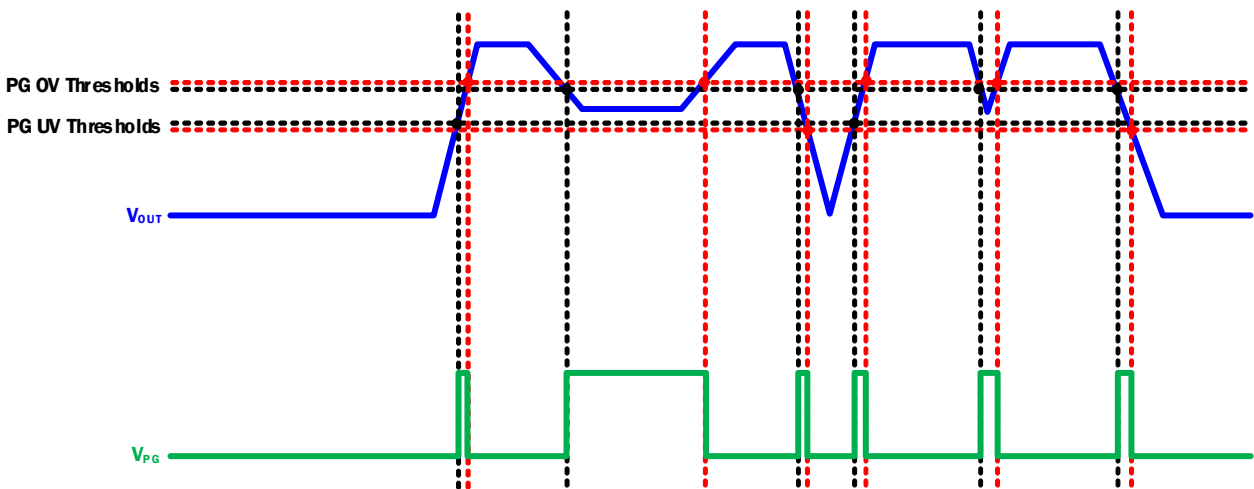
Figure 138. PG Operation
