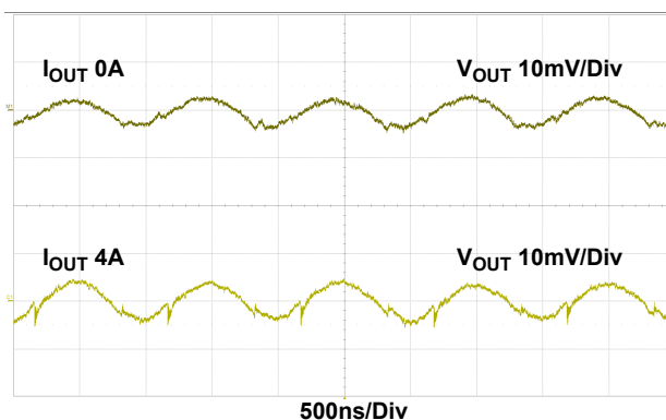
Figure 8. Output Ripple, V_{IN} = 3.3\text{V} , V_{OUT} = 0.9\text{V} , f_{SW} = 1\text{MHz} , C_{OUT} = 2 \times 22\mu\text{F} Ceramic
