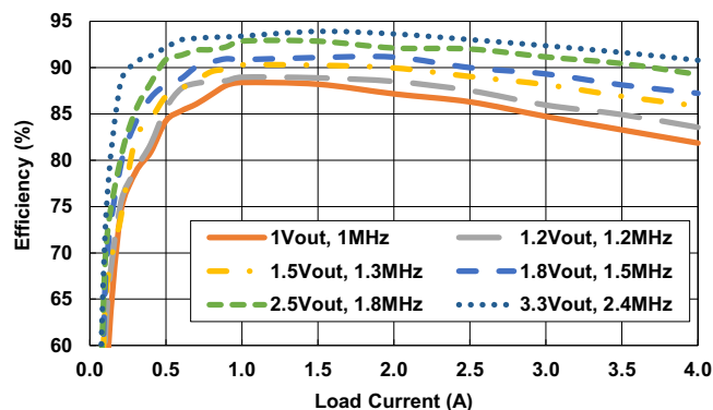
Figure 6. V_{IN} = 5\text{V}
