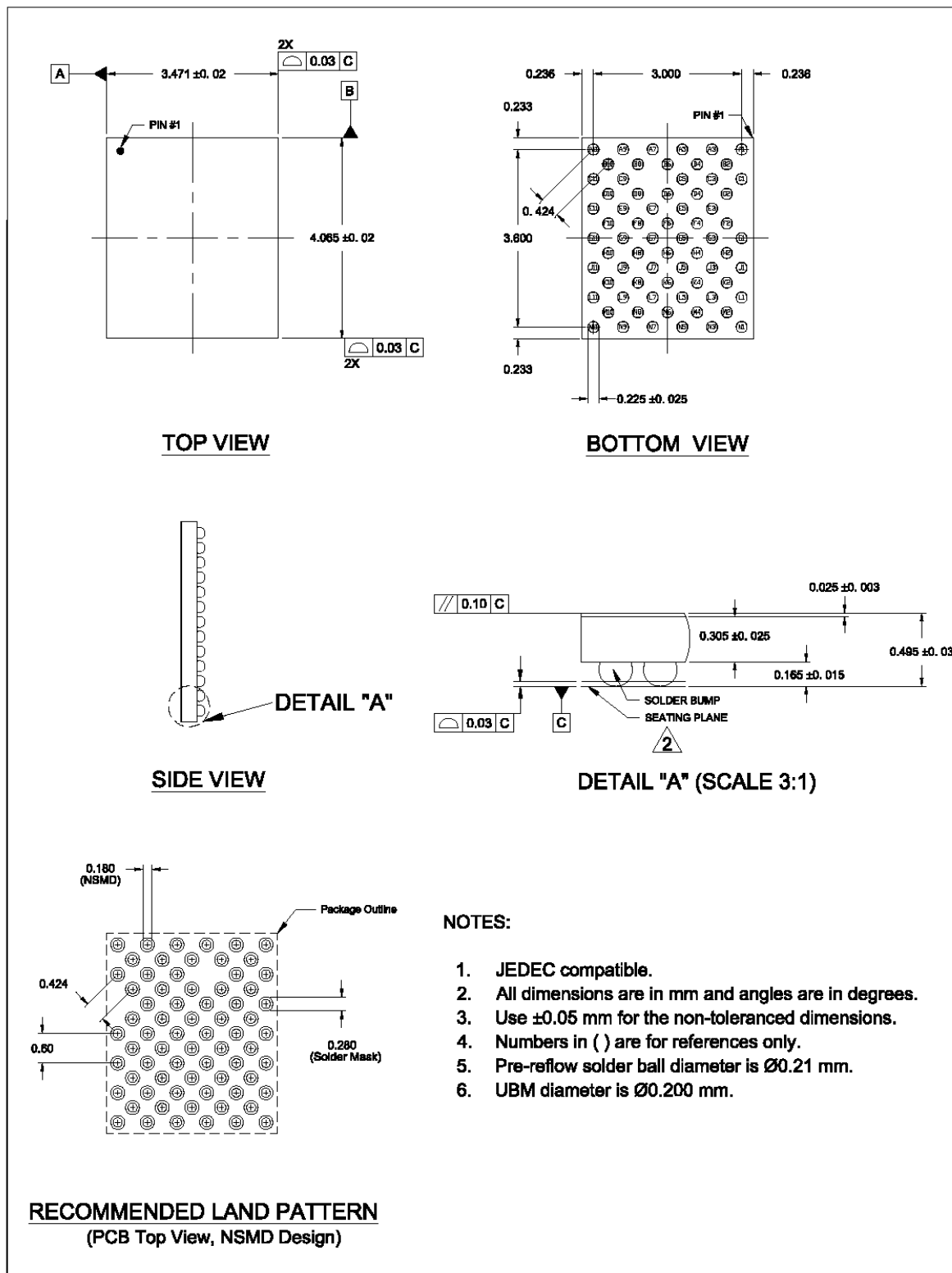
Figure 70. WLCSP70 package outline drawing
