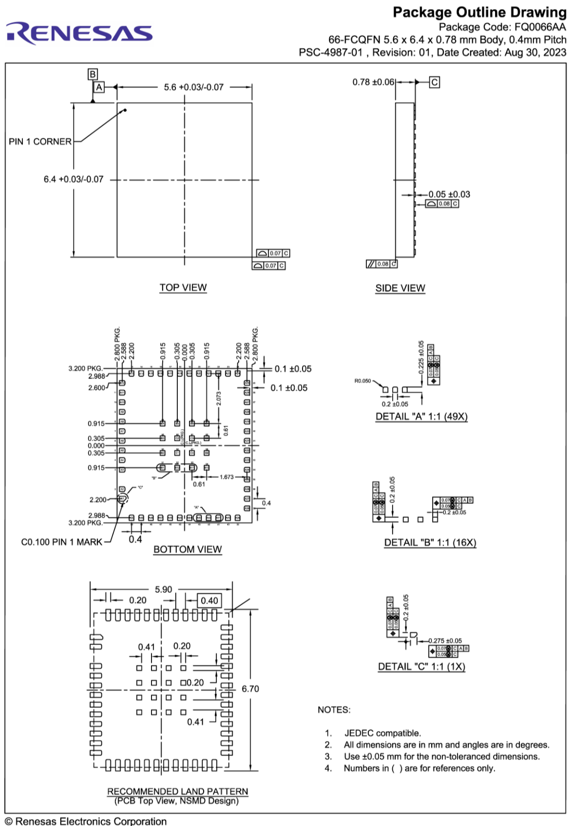
Figure 69. FCQFN66 package outline drawing
