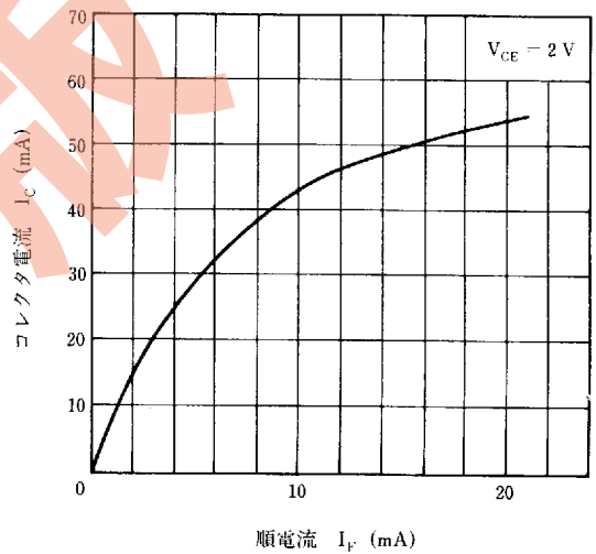
COLLECTOR CURRENT vs. FORWARD CURRENT
