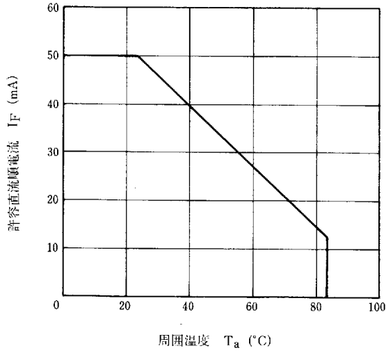
MAX. FORWARD CURRENT vs. AMBIENT TEMPERATURE
