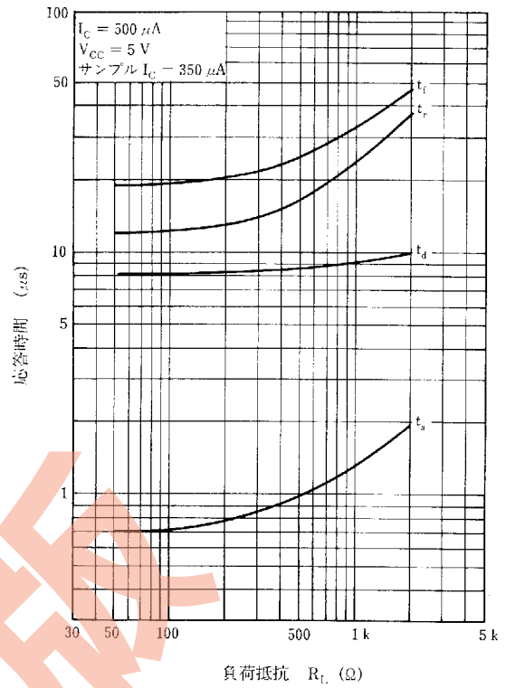
SWITCHING TIME vs. LOAD RESISTANCE
