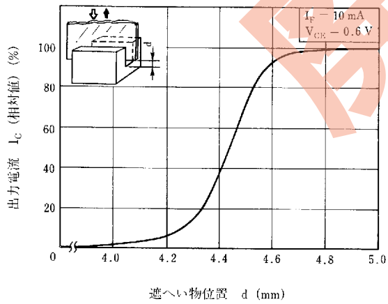
OUTPUT CHARACTERISTICS
