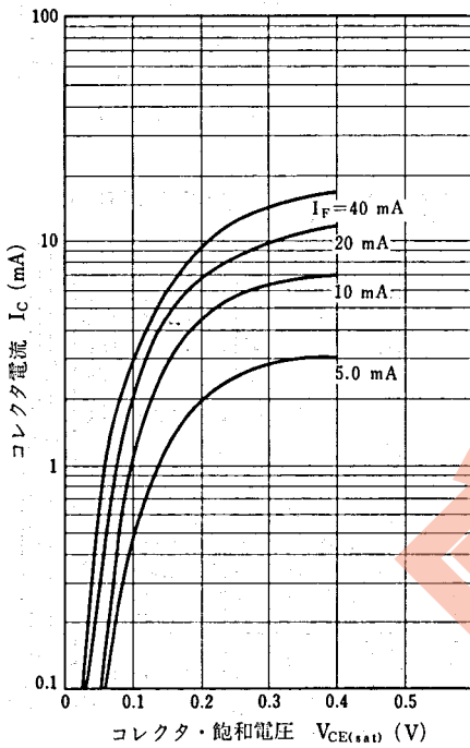
COLLECTOR CURRENT vs. COLLECTOR SATURATION VOLTAGE
