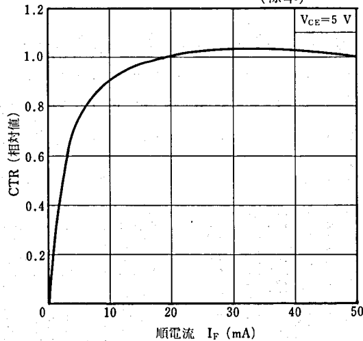
NORMALIZED CURRENT TRANSFER RATIO vs. FORWARD CURRENT (標準)
