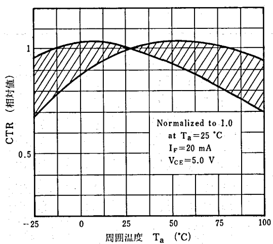
NORMALIZED CURRENT TRANSFER RATIO vs. AMBIENT TEMPERATURE
