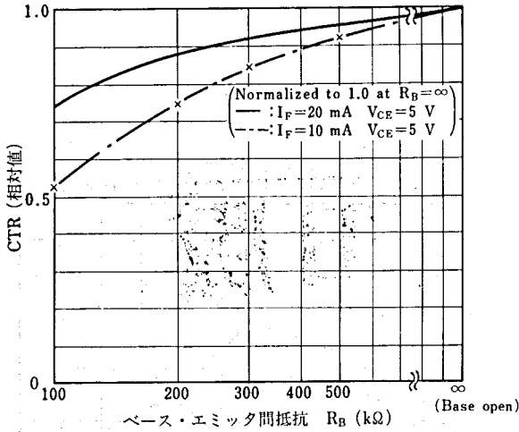
NORMALIZED CURRENT TRANSFER RATIO vs. EMITTER TO BASE RESISTANCE (PS2001B)
