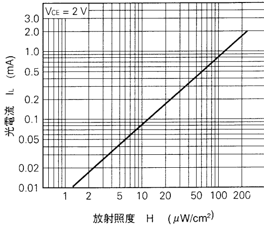
PHOTO CURRENT vs. IRRADIANCE
