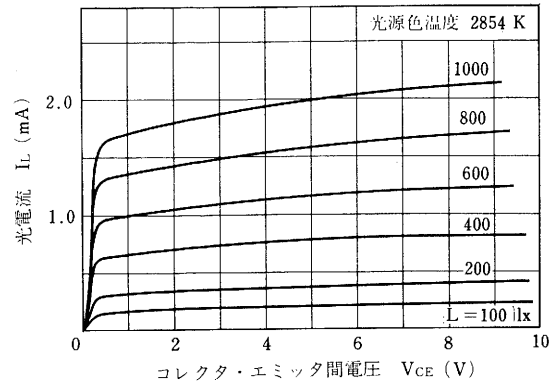
PHOTO CURRENT vs. COLLECTOR TO EMITTER VOLTAGE
