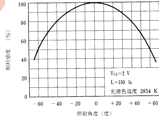
ANGULAR RESPONSE
