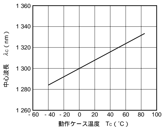
TEMPERATURE DEPENDENCY OF CENTER WAVELENGTH FOR NDL7408P SERIES
