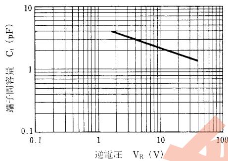
TERMINAL CAPACITANCE vs. REVERSE VOLTAGE
