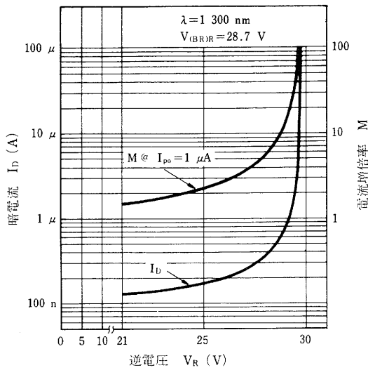
DARK CURRENT AND MULTIPLICATION FACTOR vs. REVERSE VOLTAGE
