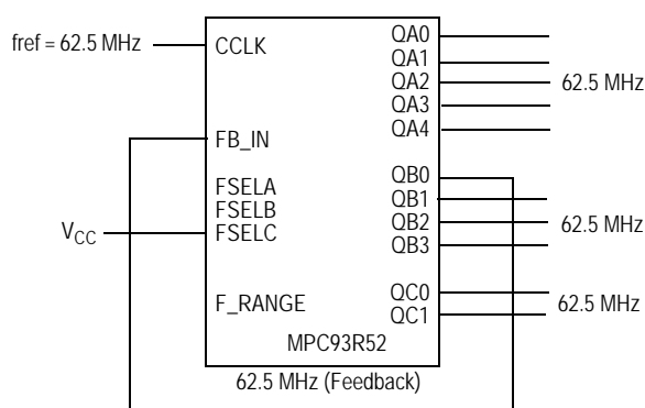
MPC93R52 zero-delay (feedback of QB0 = 62.5 MHz). All control pins are left open except FSEL = 1. All outputs are locked in frequency and phase to the input clock.
