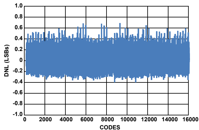
FIGURE 12. DIFFERENTIAL NONLINEARITY
