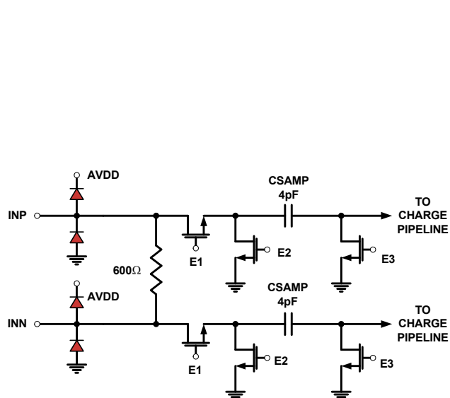
FIGURE 45. ANALOG INPUTS
