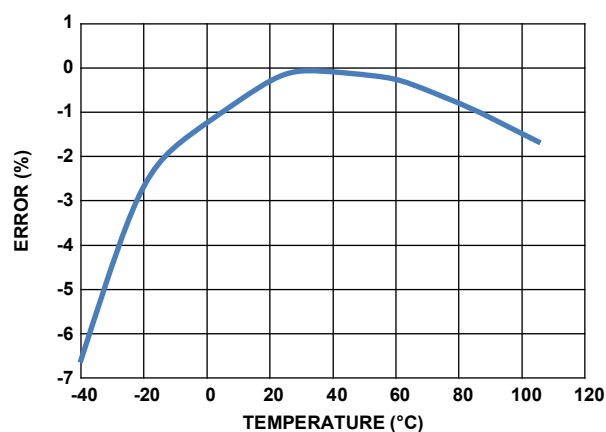
Figure 21. 4MHz Oscillator Error vs Temperature
