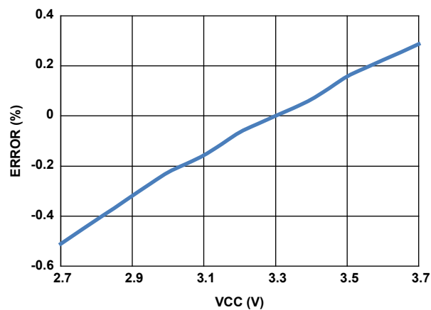
Figure 23. 32kHz Oscillator Error vs VCC
