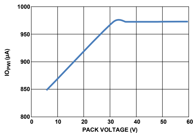
Figure 19. Open Wire Test Current vs Pack Voltage (1mA Setting)
