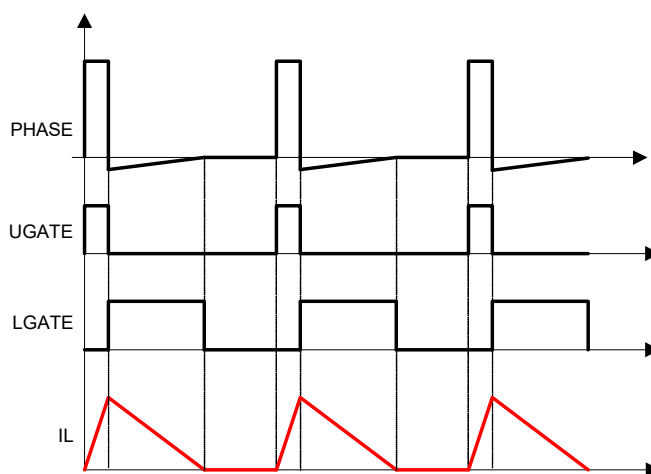
Figure 34. Diode Emulation
