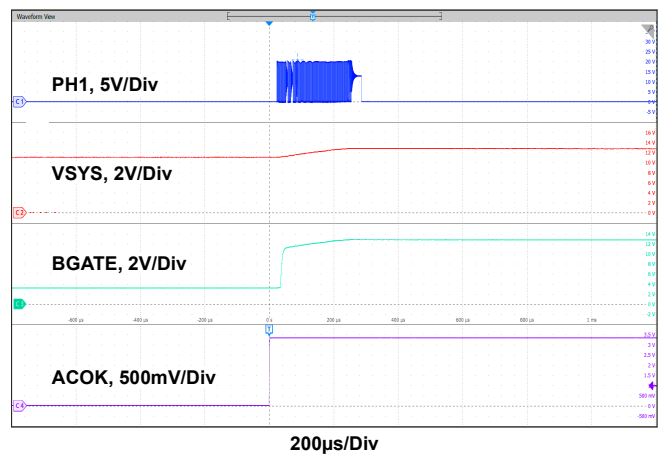
Figure 8. Adapter Insertion, V_{ADP} = 20V , V_{BAT} = 11V , ChargeCurrent = 0A (Figure 7 Zoomed In)
