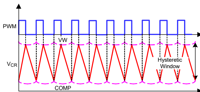
Figure 32. R3 Modulator Operation Principles In Steady State
