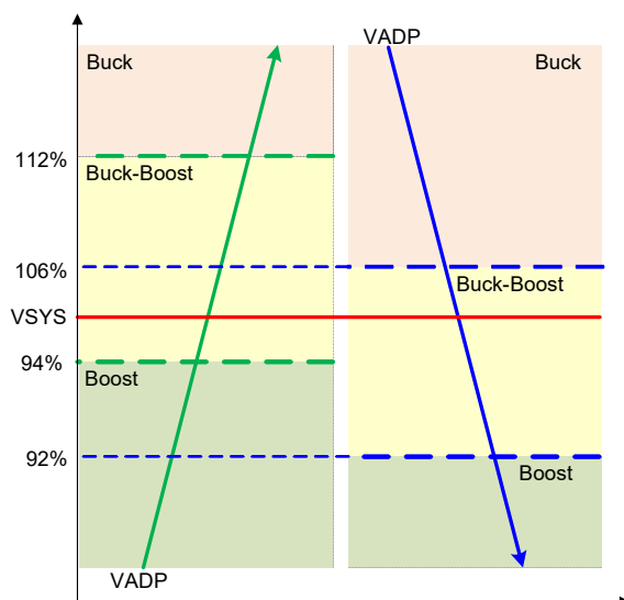
Figure 28. Operation Mode
