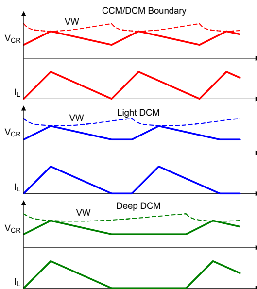
Figure 35. Period Stretching
