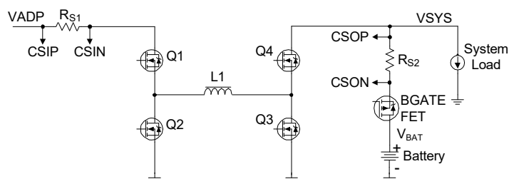
Figure 27. Buck-Boost Charger Topology
