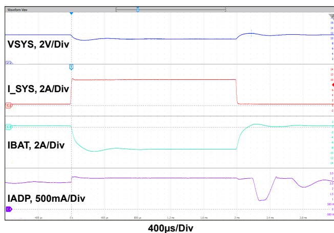
Figure 13. Boost Mode, Charging Current Loop to Adapter Current Loop Transition. V_{ADP} = 5V , MaxSystemVoltage = 12.576V , V_{BAT} = 11V , System Load 0.5A to 10A Step, AdapterCurrentLimit = 3A , ChargeCurrent = 0.5A
