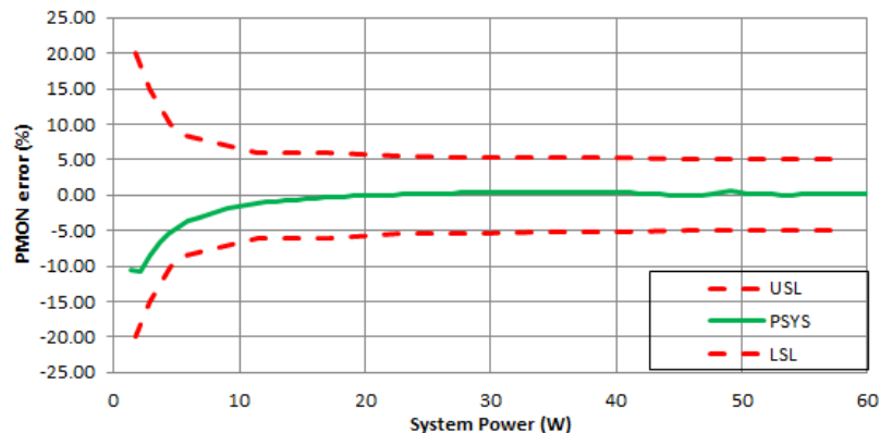
Figure 38. PSYS Accuracy and Limits
