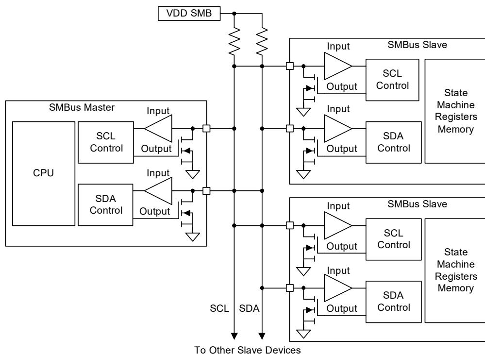
Figure 22. General SMBus
