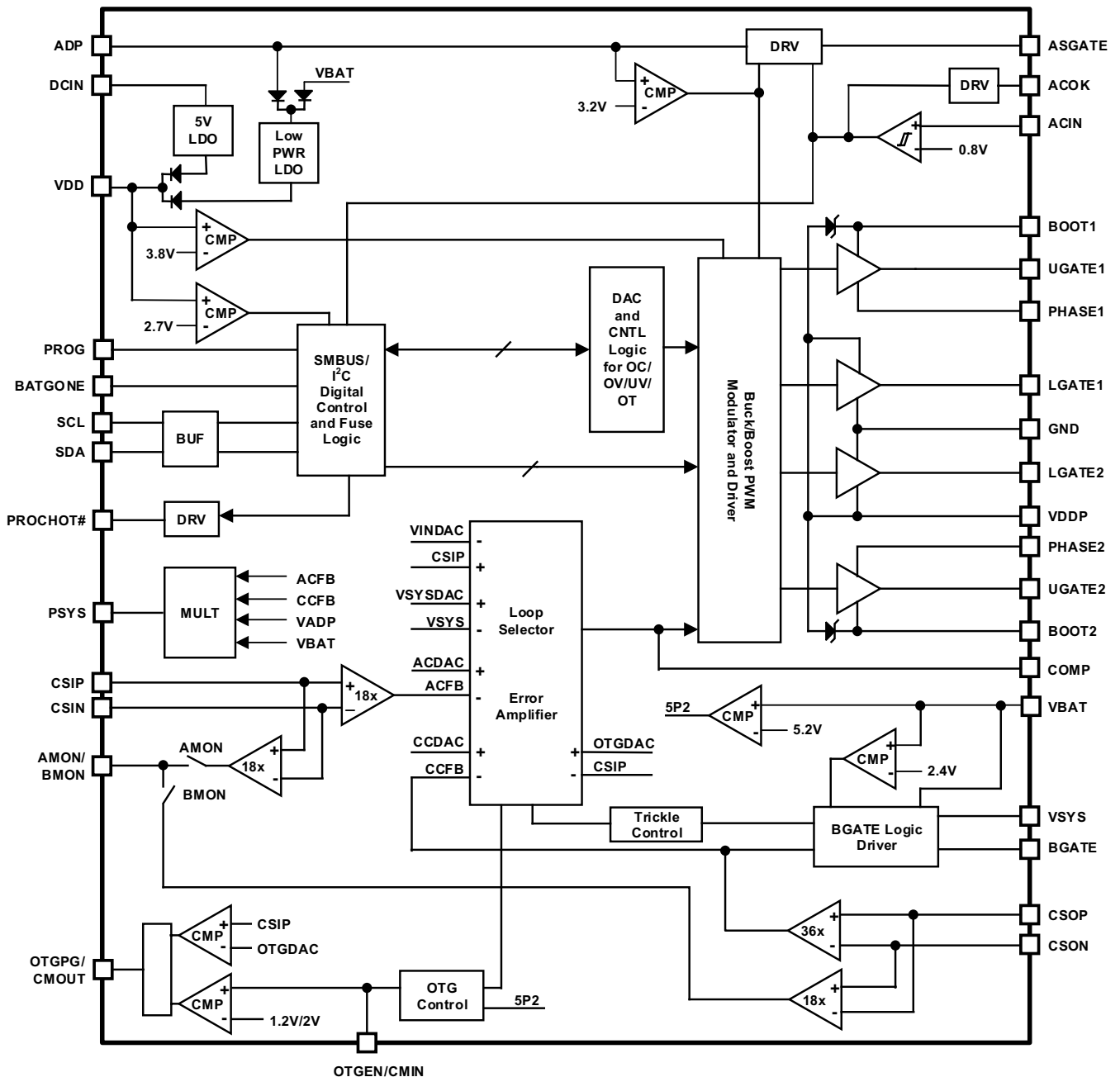
Figure 4. Block Diagram
