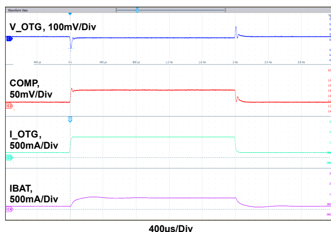
Figure 21. OTG Mode 0.5A to 2A Transient Load, OTG Voltage = 5.12V
