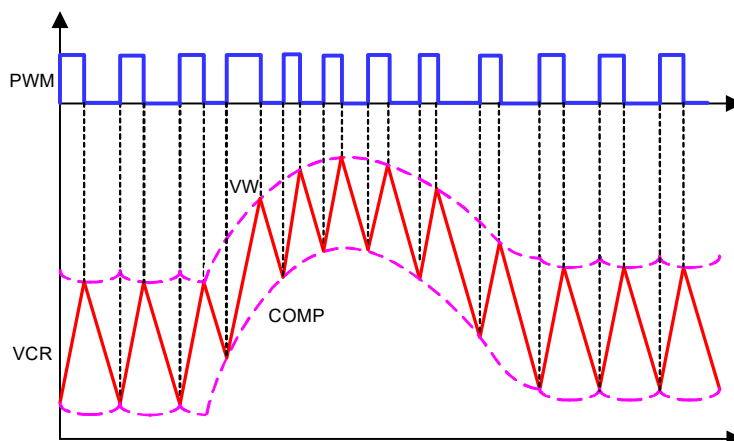
Figure 33. R3 Modulator Operation Principles In Dynamic Response
