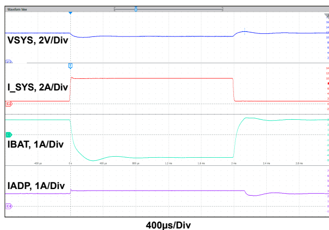
Figure 17. Buck Mode, Charging Current Loop to Adapter Current Loop Transition. V_{ADP} = 20V , MaxSystemVoltage = 12.576V , V_{BAT} = 11V , System Load 1A to 10A Step, AdapterCurrentLimit = 3A , ChargeCurrent = 3A
