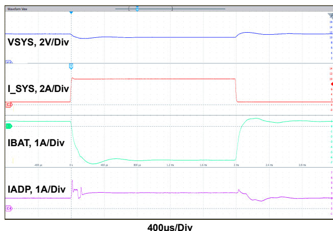
Figure 15. Buck-Boost Mode, Charging Current Loop to Adapter Current Loop Transition. V_{ADP} = 12V , MaxSystemVoltage = 12.576V , V_{BAT} = 11V , System Load 1A to 10A Step, AdapterCurrentLimit = 3A , ChargeCurrent = 1A
