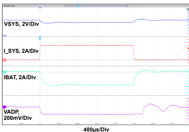
Figure 19. Boost Mode, Charging Current Loop to Input Voltage Loop Transition. V_{ADP} = 5.004V , MaxSystemVoltage = 12.576V , V_{BAT} = 11V , VINDAC = 4.437V , System Load 0A to 10A Step, ChargeCurrent = 0.5A
