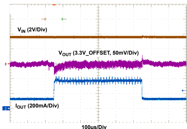
Figure 50. Load Transient: V_{IN} = 3.6V , V_{OUT} = 3.3V , I_{OUT} = 0.125A to 0.375A , Slew Rate = 1A/\mu s
