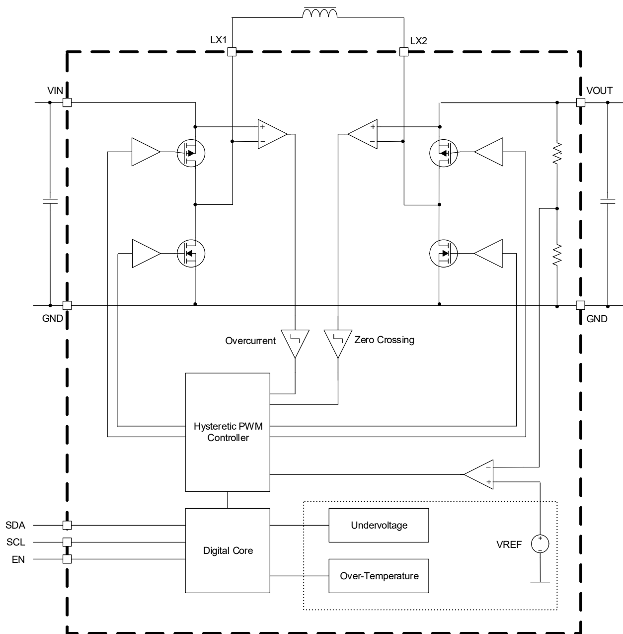
Figure 3. Block Diagram
