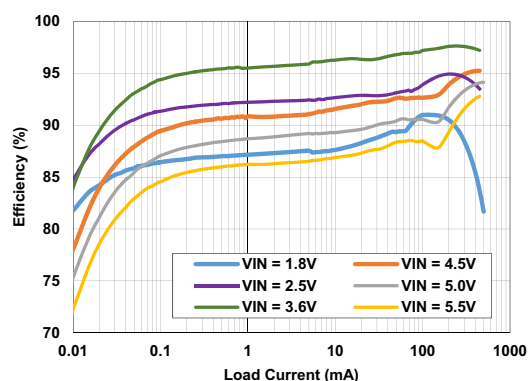
Figure 2. Efficiency vs Load Current: V_{OUT} = 3.3V , T_A = +25^\circ C
