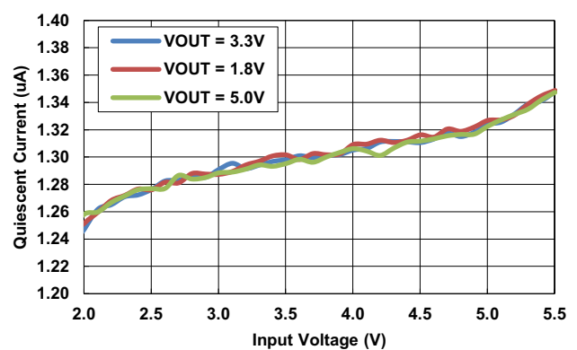
Figure 21. Quiescent Current vs Input Voltage
