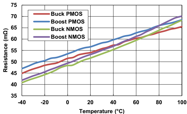
Figure 22. Switch Resistance vs Temperature
