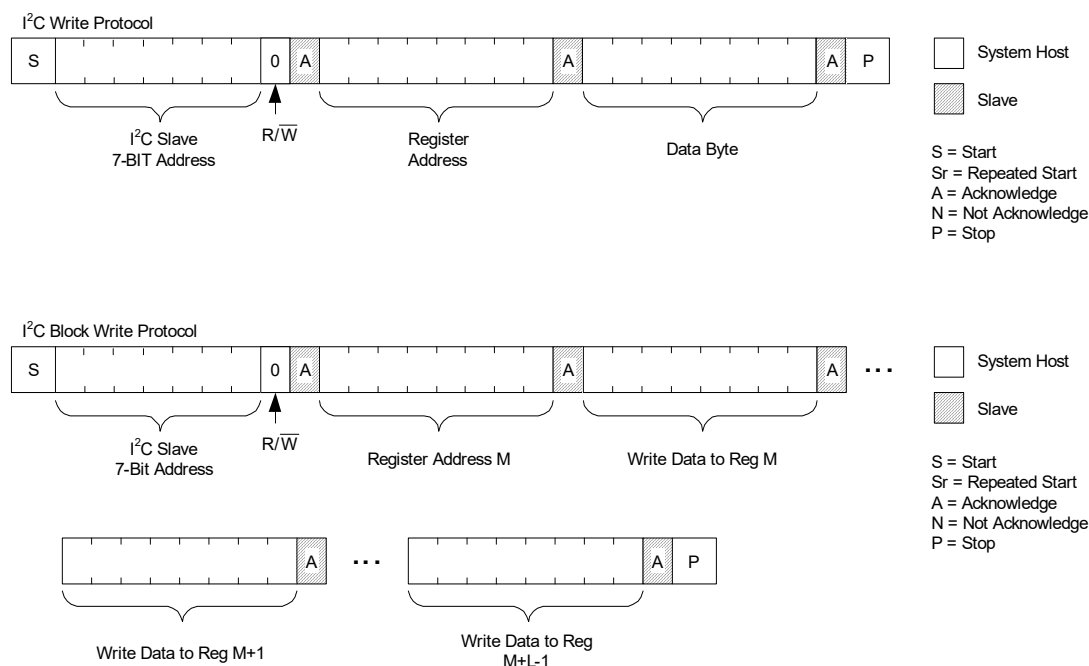
Figure 56. I²C Register Write Protocols
