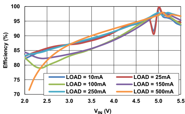
Figure 8. Efficiency vs Input Voltage: V_{OUT} = 5V
