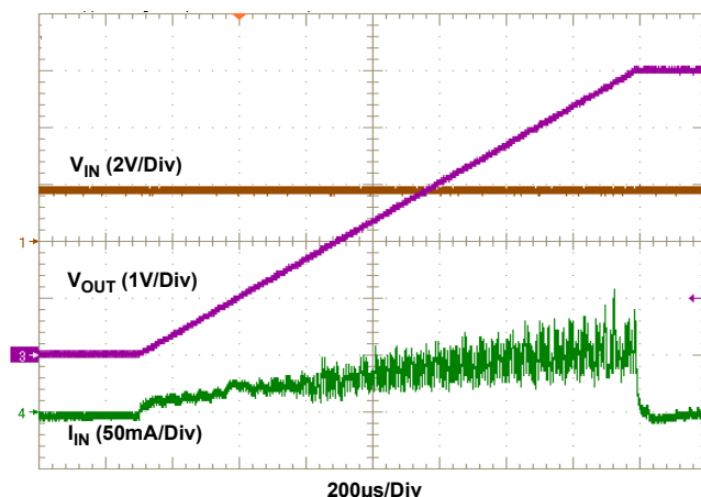
Figure 32. Soft-Start: V_{IN} = 1.8V , V_{SET} = 5.0V , No Load
