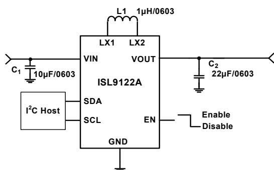
Figure 1. Typical Application (Minimum De-rated C_2 = 6\mu F )
