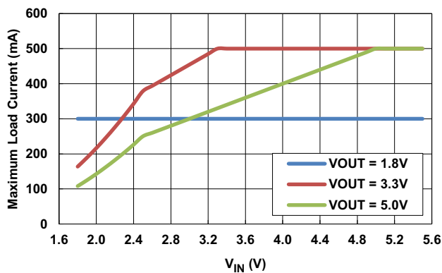
Figure 16. Maximum Load Current vs Input Voltage
