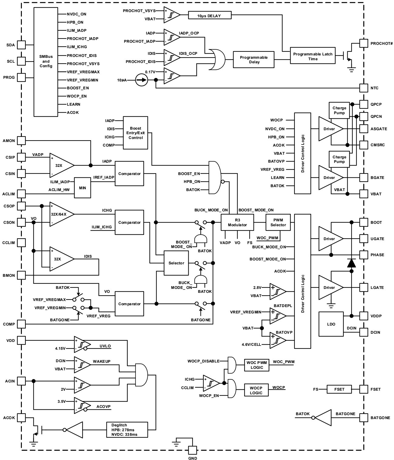
Figure 2. Block Diagram
