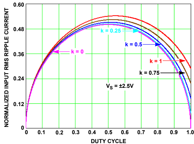
Figure 37. Normalized RMS Input Current at EFF = 1
