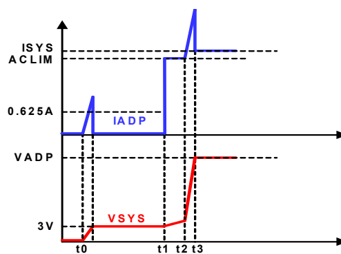
Figure 33. No Battery Soft-Start with I_{SYS} > ACLIM
