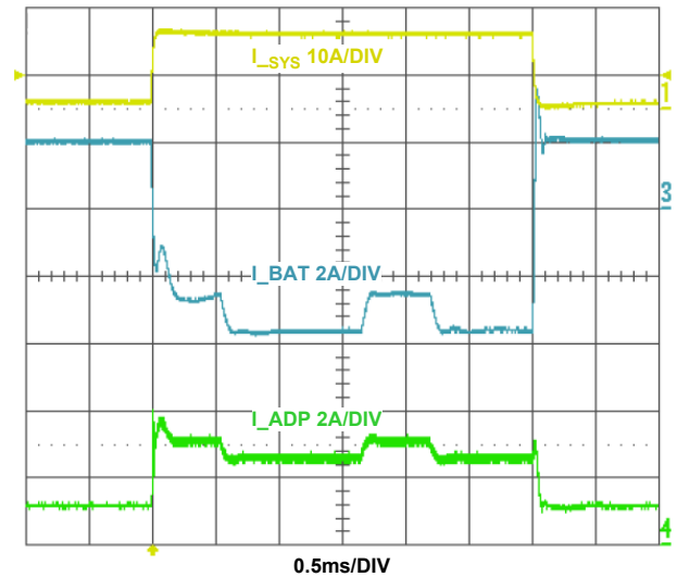
Figure 7. Two Level Adapter Current Limit. V_{ADP} = 20V , AdapterCurrentLimit1 = 2.56A , AdapterCurrentLimit2 = 3.072A , T2 = 500\mu s , T1 = 1ms , V_{BAT} = 7V , MaxChargeVoltage = 8.192V , ChargeCurrent = 2.016A , 1A to 12A System Load Step
