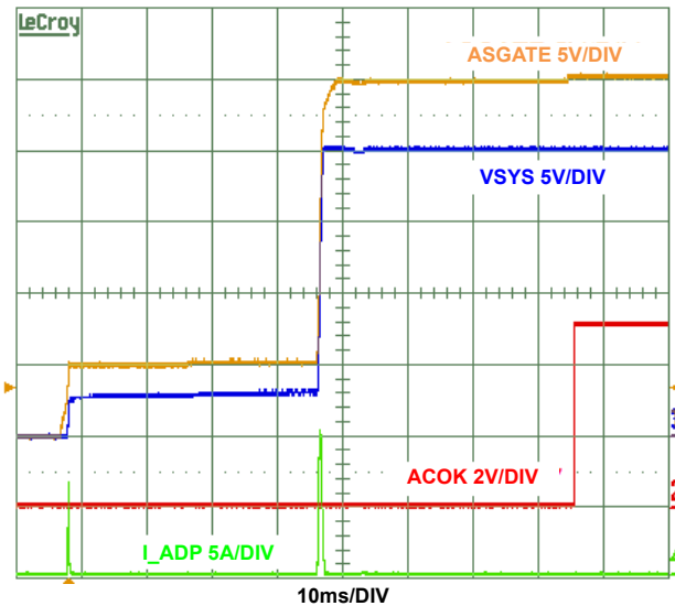
Figure 8. HPB: Adapter Insertion ASGATE Inrush Current Control. No Battery, V_{ADP} = 20V , 330 \mu F System Rail Capacitance
