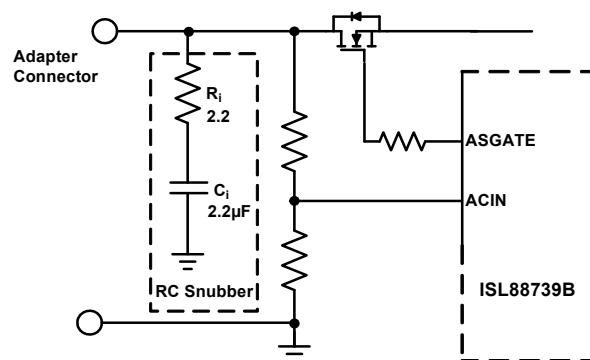
Figure 36. Adapter Input RC Snubber Circuit
