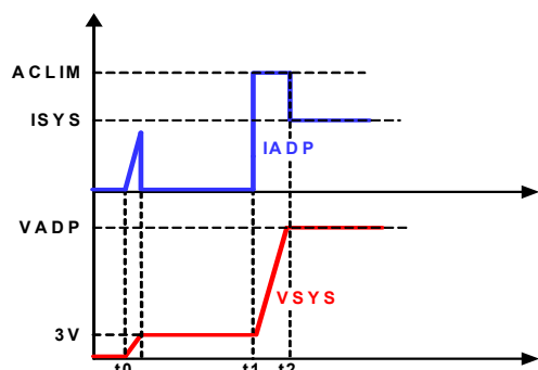
Figure 32. No Battery Soft-Start with I_{SYS} < ACLIM
