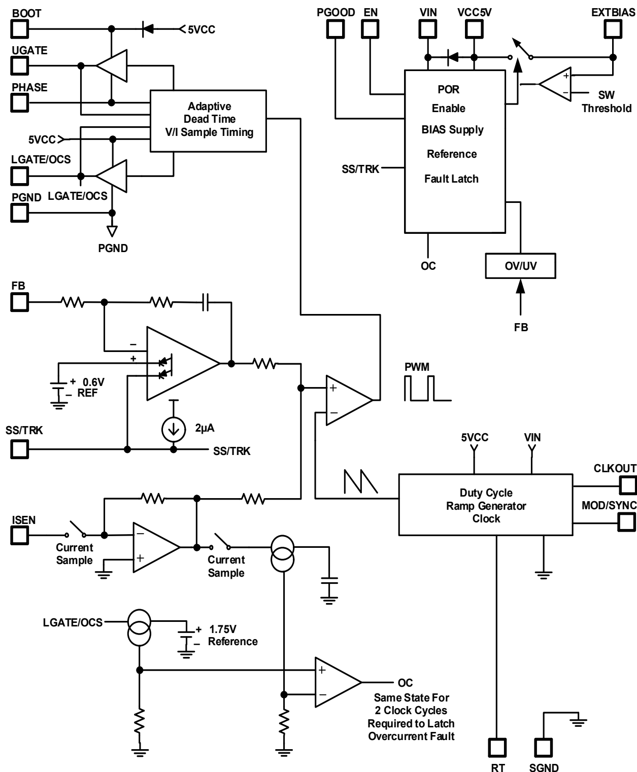
Figure 3. Block Diagram
