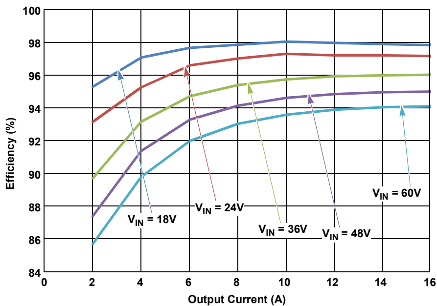
Figure 2. Efficiency
