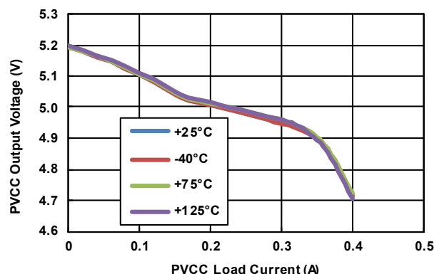
Figure 20. PVCC Output Voltage (V6 = 6V)
