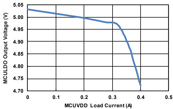
Figure 72. MCULDO Load Regulation, V6 = 6V
