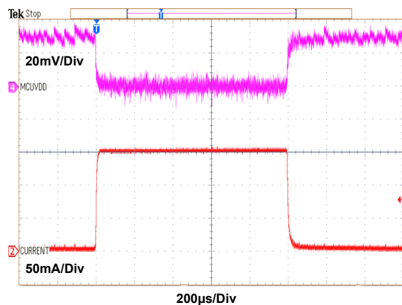
Figure 71. MCULDO Load Transient, I_{LOAD} = 0 to 150mA, MCULDO Offset = 5.0V
