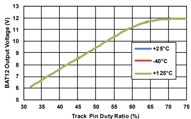
Figure 23. BAT12 Output Voltage (Digital Tracking Mode, FTRK = 500kHz, Buck Mode, DE Mode, Phase Drop Disabled, f_{CLK} = 100kHz )
