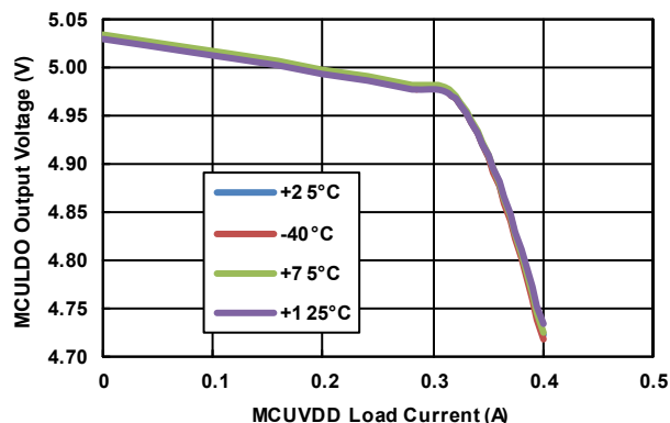
Figure 19. MCULDO Output Voltage (V6 = 6V)
