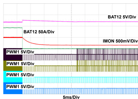
Figure 65. RL = 0.10\Omega \rightarrow 0.15\Omega
