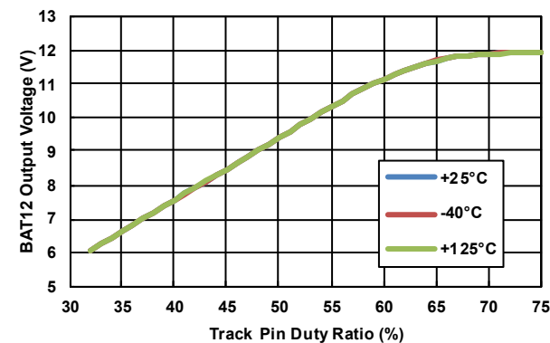
Figure 24. BAT12 Output Voltage (Digital Tracking Mode, FTRK = 200kHz, Buck Mode, DE Mode, Phase Drop Disabled, f_{CLK} = 100kHz )
