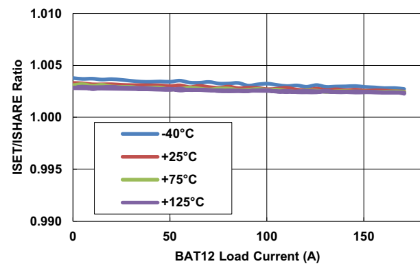
Figure 99. ISET/ISHARE Ratio vs Load Current in Buck/FPWM/NO-PD
