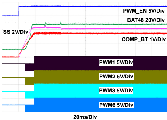
Figure 43. Soft-Start in Boost/DE/NO-PD, 12V to 48V, 6Ω Load on BAT48
