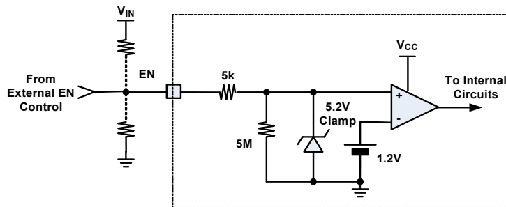
Figure 132. Enable Block
