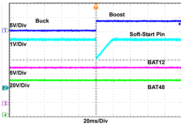
Figure 121. Buck to Boost
