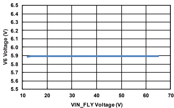
Figure 76. V6 Line Regulation, Temperature = +25°, f_{SW} = 100kHz, V12 Load = 200mA
