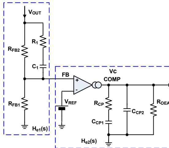
Figure 139. Type-3 Compensation
