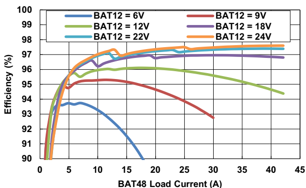
Figure 2. Boost Mode, DE Mode, Phase-Drop Enabled
