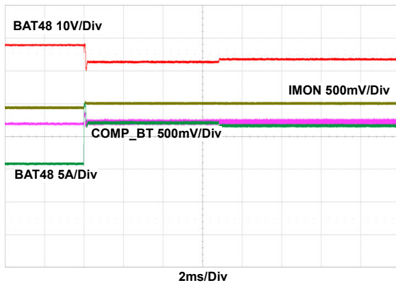
Figure 66. Average Constant Current Control Loop, CCL Transition in Boost/DE/NO-PD, RL1 = 2.5\Omega \rightarrow 2\Omega
