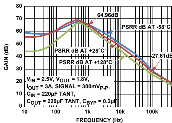
FIGURE 28. PSRR
