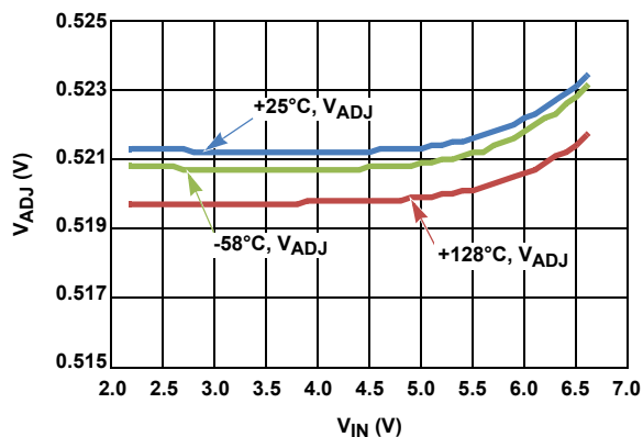
FIGURE 17. V_{IN} vs V_{ADJ} OVER-TEMPERATURE
