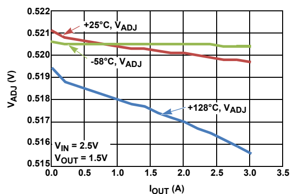
FIGURE 12. LOAD REGULATION, V_{ADJ} vs I_{OUT}
