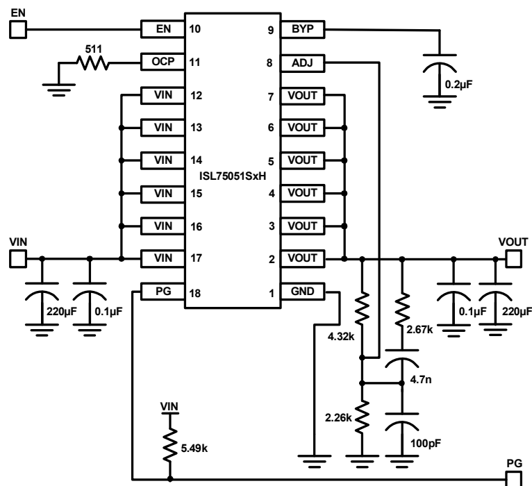
FIGURE 4. TYPICAL APPLICATION
