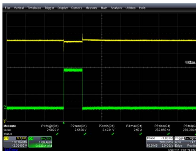
FIGURE 22. TRANSIENT LOAD RESPONSE, V_{IN} = 3.3V , V_{OUT} = 2.5V , C_{OUT} = 220\mu F , 25m\Omega
