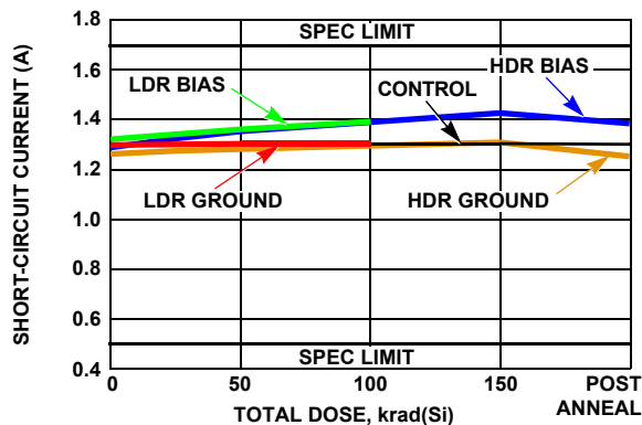
FIGURE 10. OUTPUT SHORT-CIRCUIT CURRENT, R_{SET} = 5.11k\Omega , 5.5V IN
