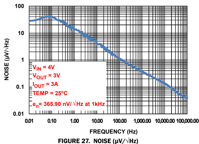
FIGURE 27. NOISE (μV/√Hz)
