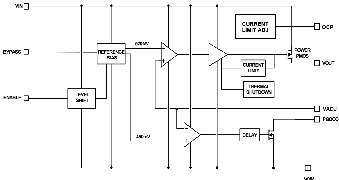
FIGURE 3. BLOCK DIAGRAM
