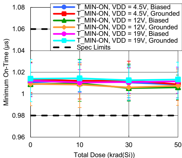
Figure 98. Minimum On-Time with R_{BLANK} = 10.5k\Omega vs TID
