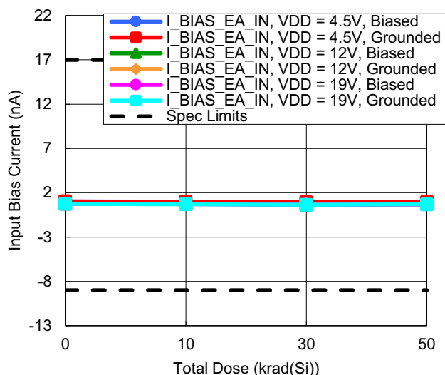
Figure 96. Input Bias Current with VCM = 2V vs TID
