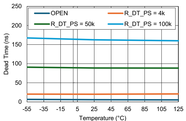
Figure 36. OUTB Falling to SRB Rising Dead Time vs Temperature at Various R_{DT\_PS} Resistors with V_{DD} = 19V
