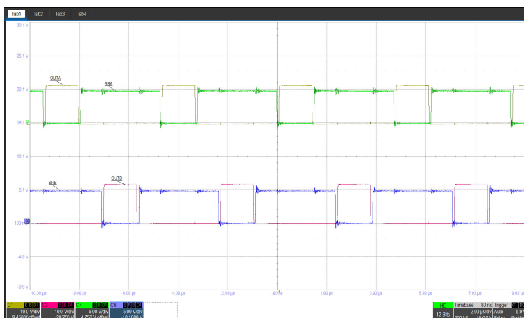
Figure 51. DCSL Tied to Ground PWM Outputs Waveforms
