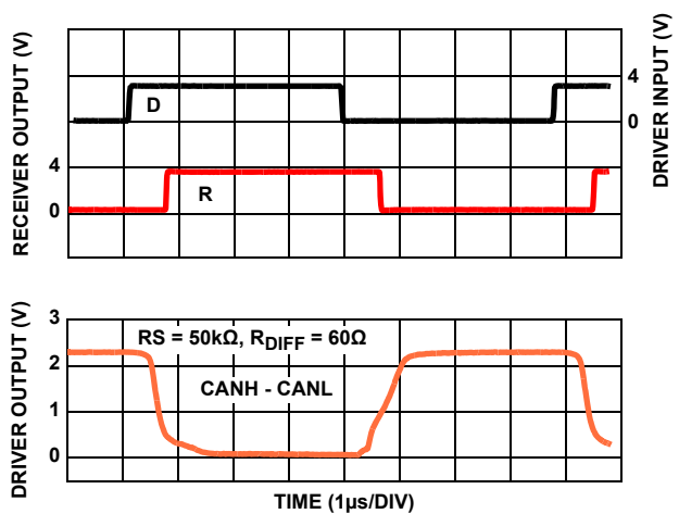
FIGURE 42. SLOW DRIVER AND RECEIVER WAVEFORMS
