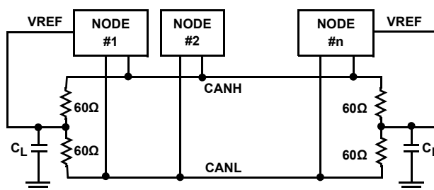
FIGURE 18. SPLIT TERMINATION
