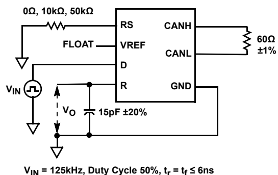
FIGURE 15A. TOTAL LOOP DELAY TEST CIRCUIT
