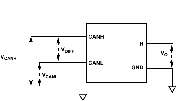
Figure 15. Receiver Voltage Definitions
