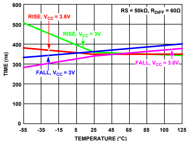
Figure 38. Transmitter Rise and Fall Times vs Temperature at Slow Speed
