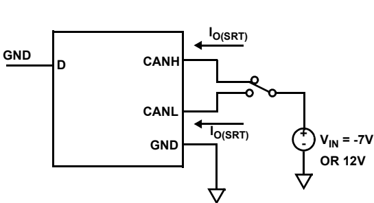
Figure 24. Output Short-Circuit Current Test Circuit
