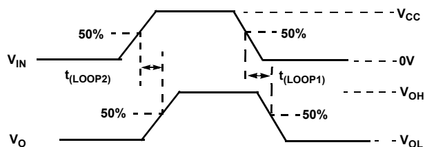
Figure 21. Total Loop Delay Measurement Points
