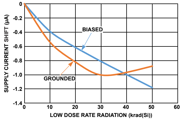
FIGURE 69. I_{EE} SUPPLY CURRENT SHIFT vs LDR RADIATION
