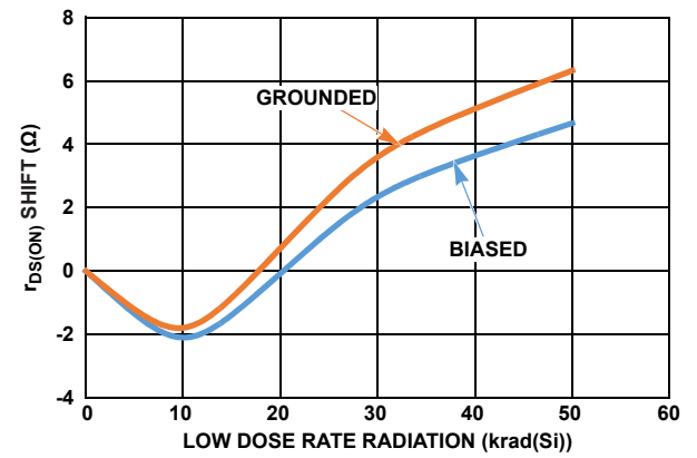
FIGURE 73. r_{DS(ON)} SHIFT ( V_{IN} = -5V ) vs LDR RADIATION
