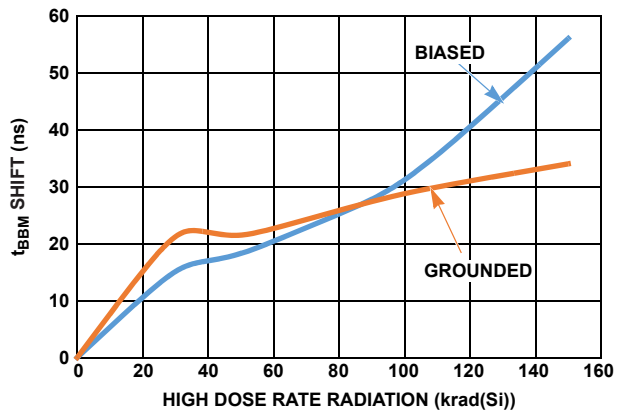
FIGURE 53. t_{BBM} SHIFT vs HDR RADIATION
