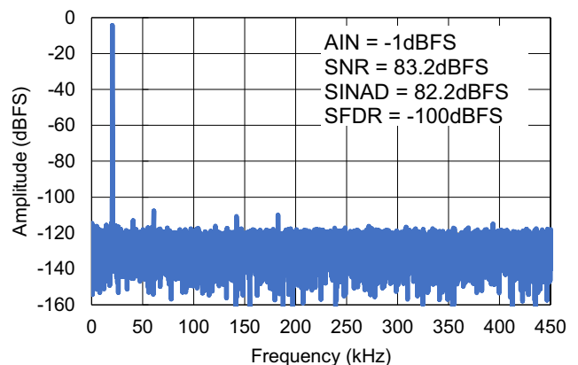
Figure 2. FFT - 20.3kHz
