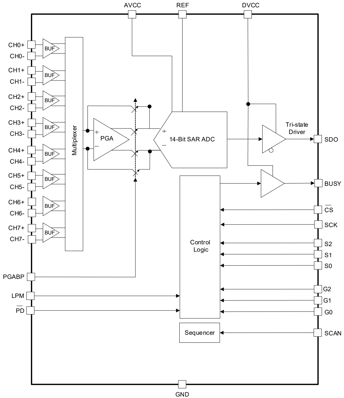
Figure 4. Block Diagram
