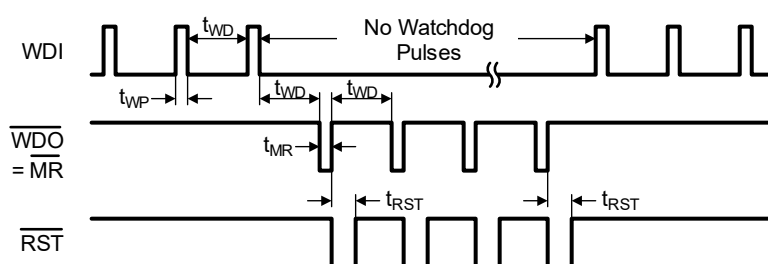
Figure 37. /WDO, /RST Timing Diagram
