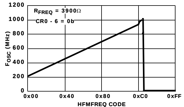
FIGURE 6. HFM CONTROL; V_{SO} = 4.5V ; TEMP = +125^{\circ}C
