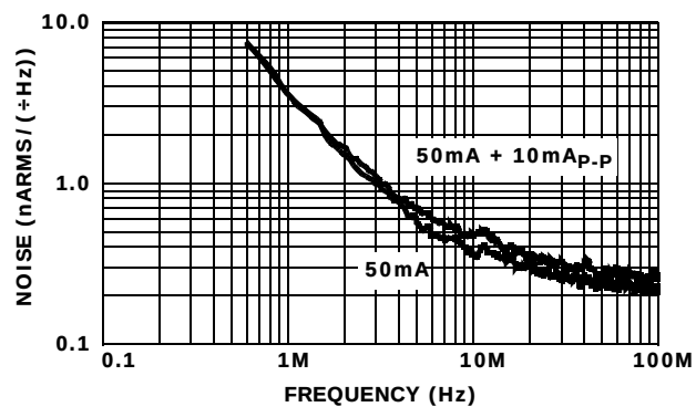
FIGURE 9. I_{\text{BLUE}} NOISE vs FREQUENCY
